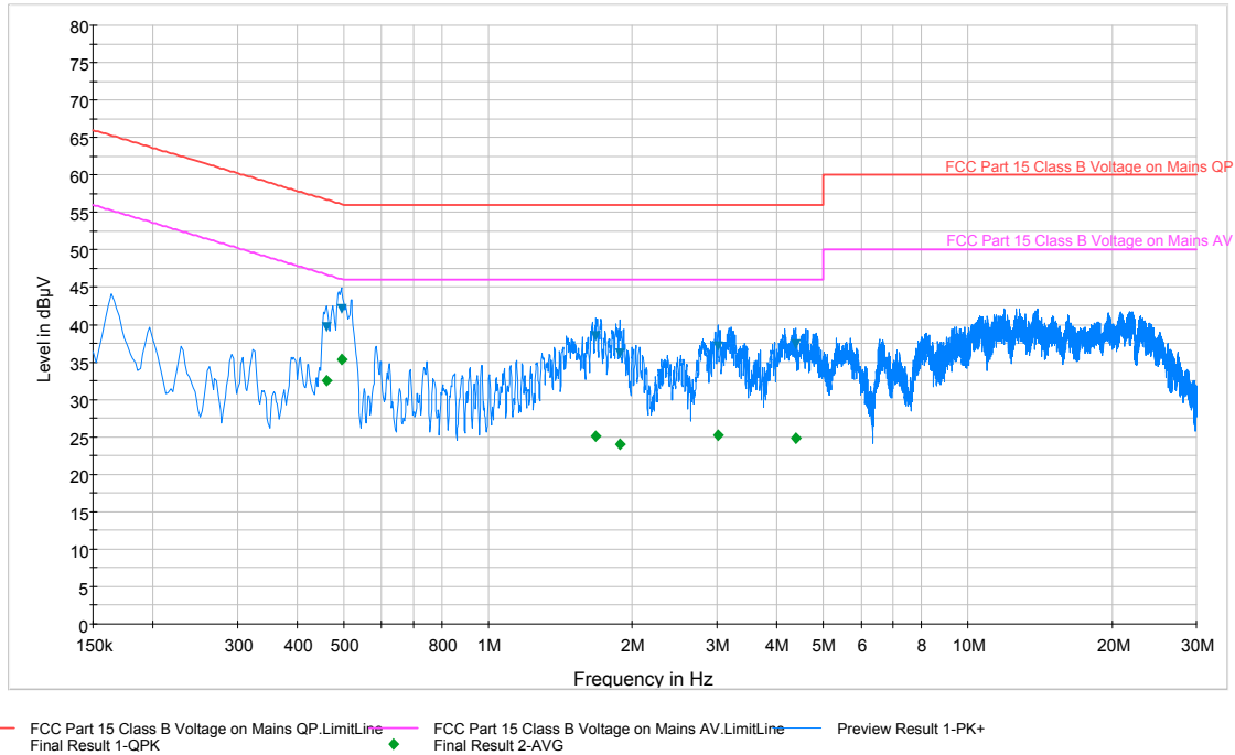
Plot 6-47. Line-Conducted Test Plot (N)
