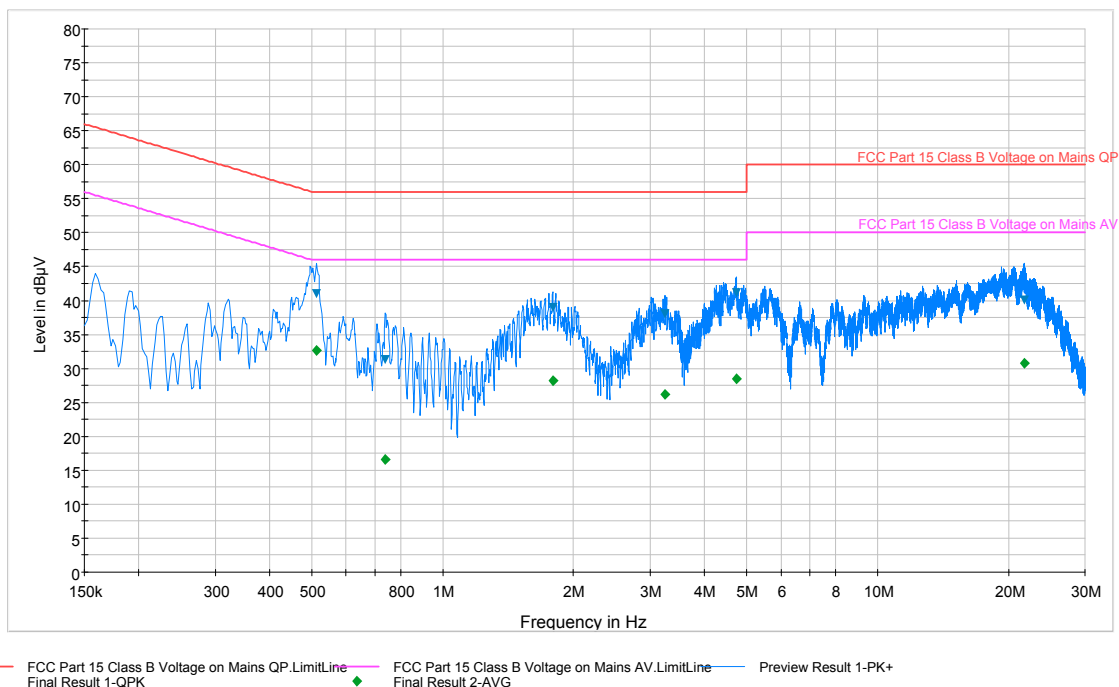
Plot 6-46. Line-Conducted Test Plot (L1)
