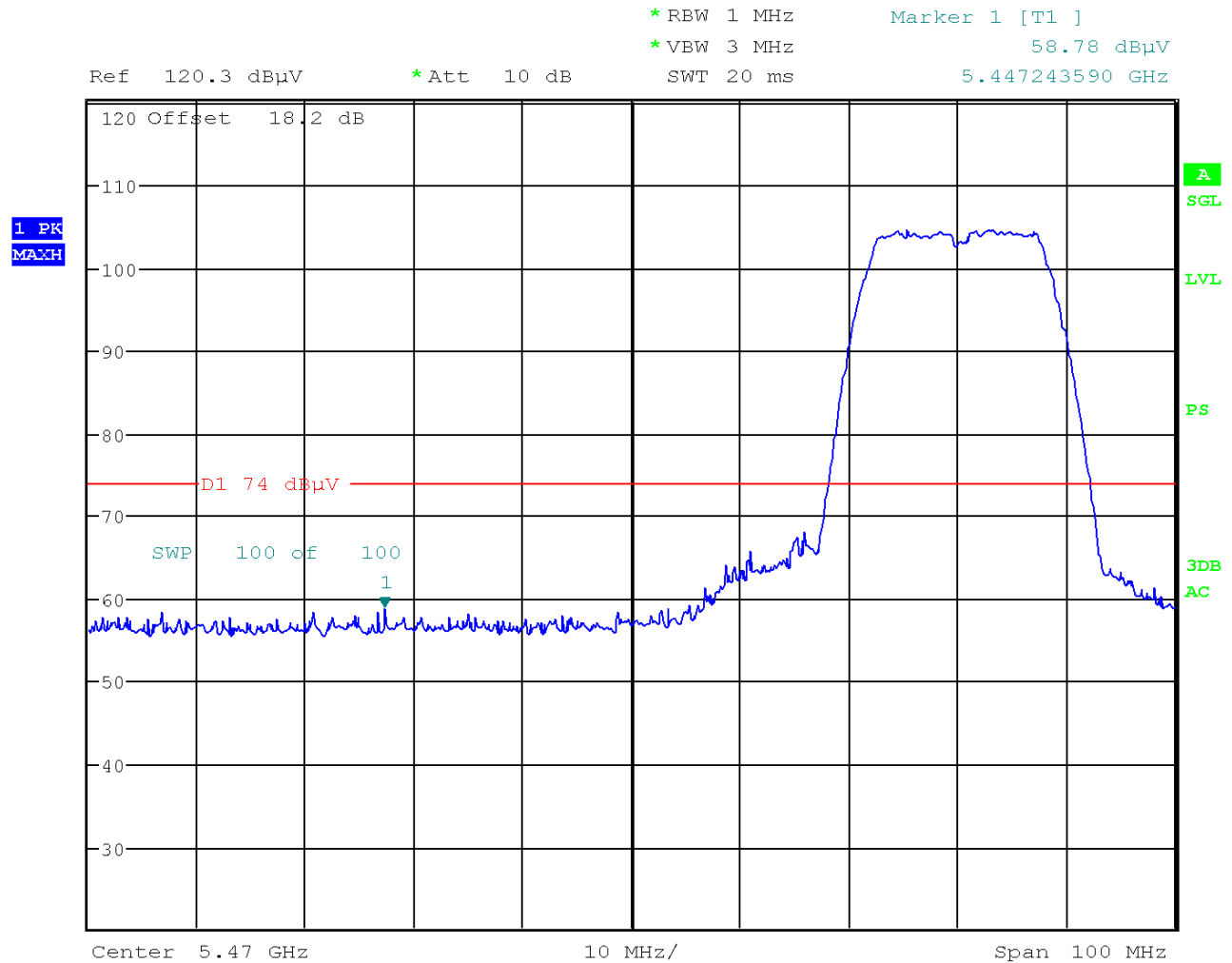
Plot 6-6. Radiated Restricted Lower Band Edge Plot (Peak – UNII Band 2C)
