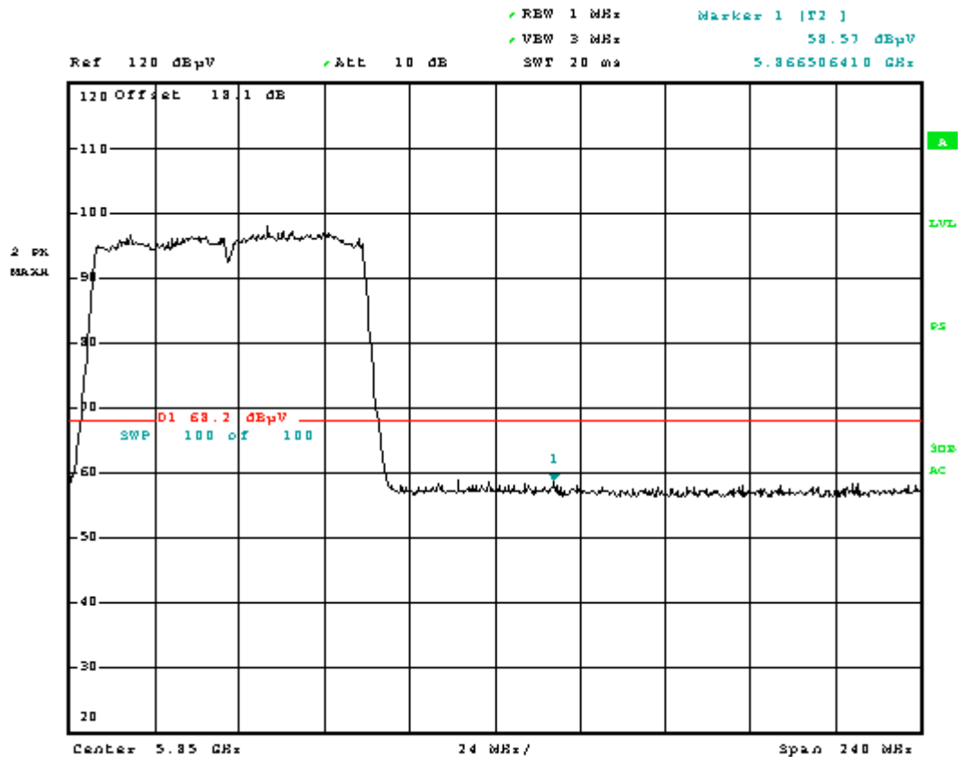
Plot 6-21. Radiated Restricted Upper Band Edge Plot (Peak – UNII Band 3)
