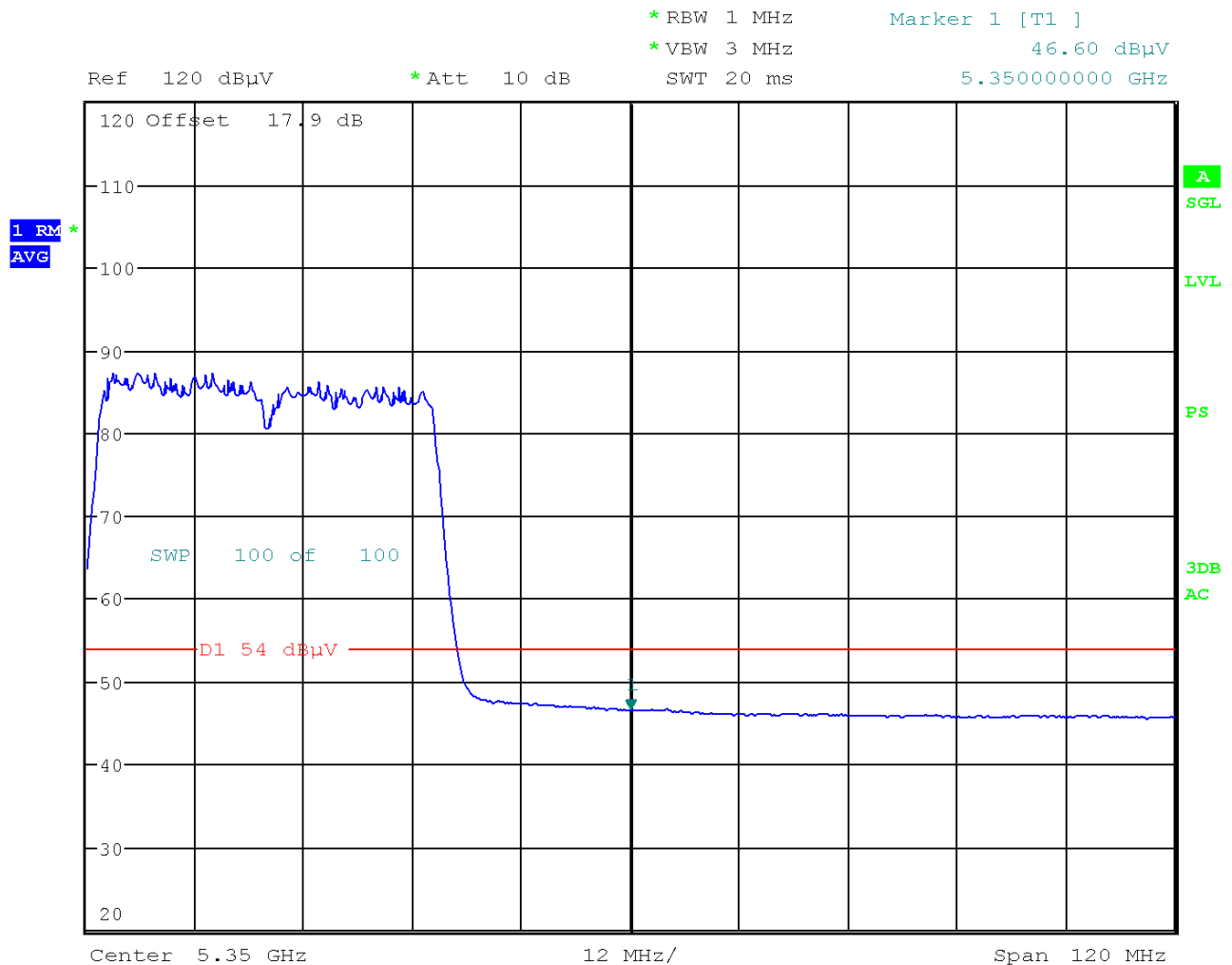
Plot 6-10. Radiated Restricted Upper Band Edge Plot (Average – UNII Band 2A)
