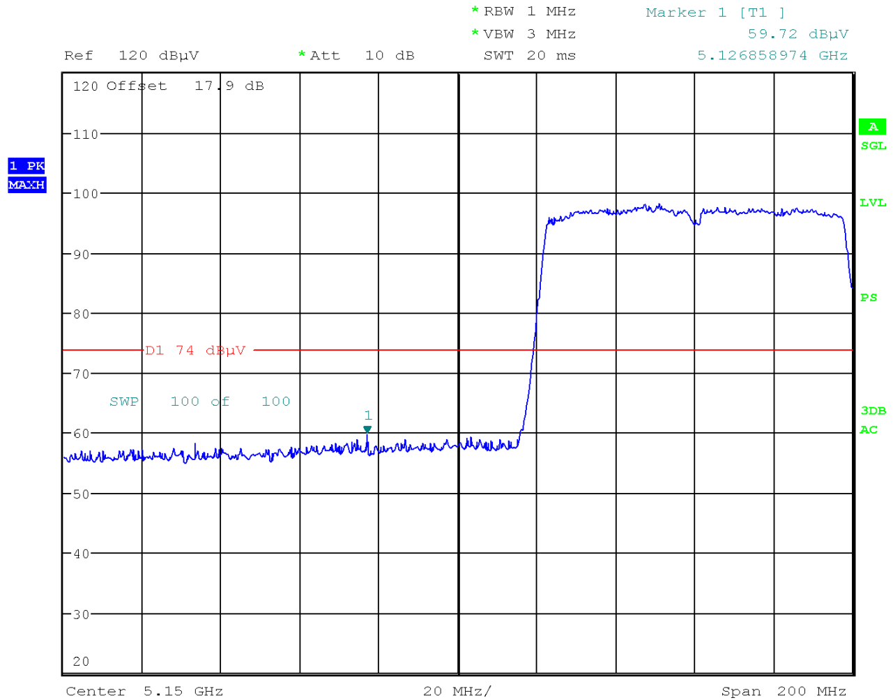
Plot 6-16. Radiated Restricted Lower Band Edge Plot (Peak – UNII Band 1)
