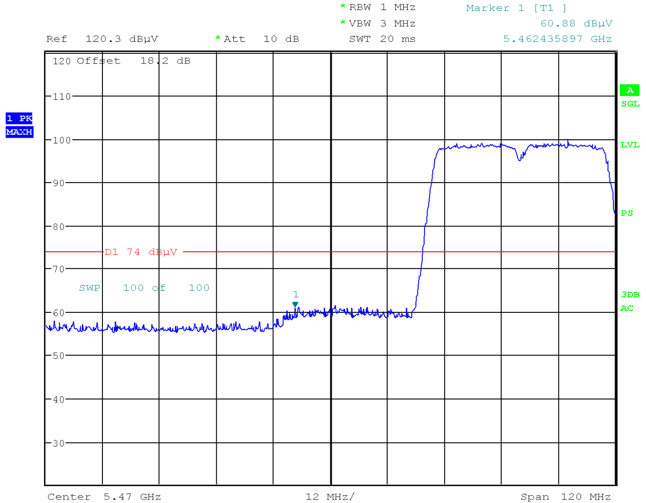
Plot 6-13. Radiated Restricted Lower Band Edge Plot (Peak – UNII Band 2C)
