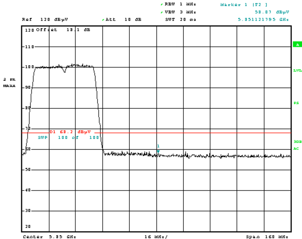
Plot 6-14. Radiated Upper Band Edge Plot (Peak – UNII Band 3)
