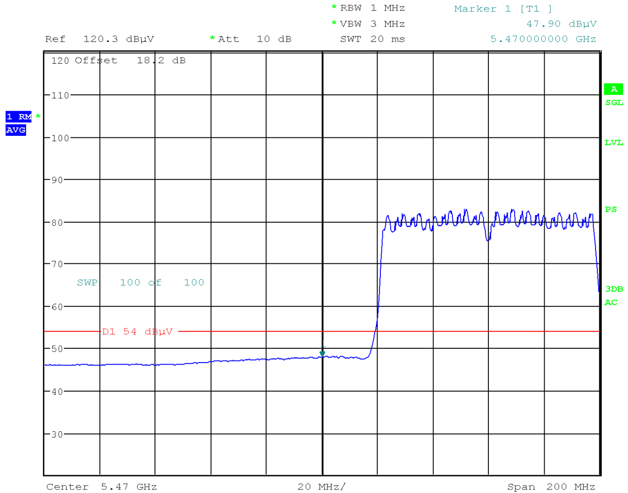
Plot 6-19. Radiated Restricted Lower Band Edge Plot (Average – UNII Band 2C)
