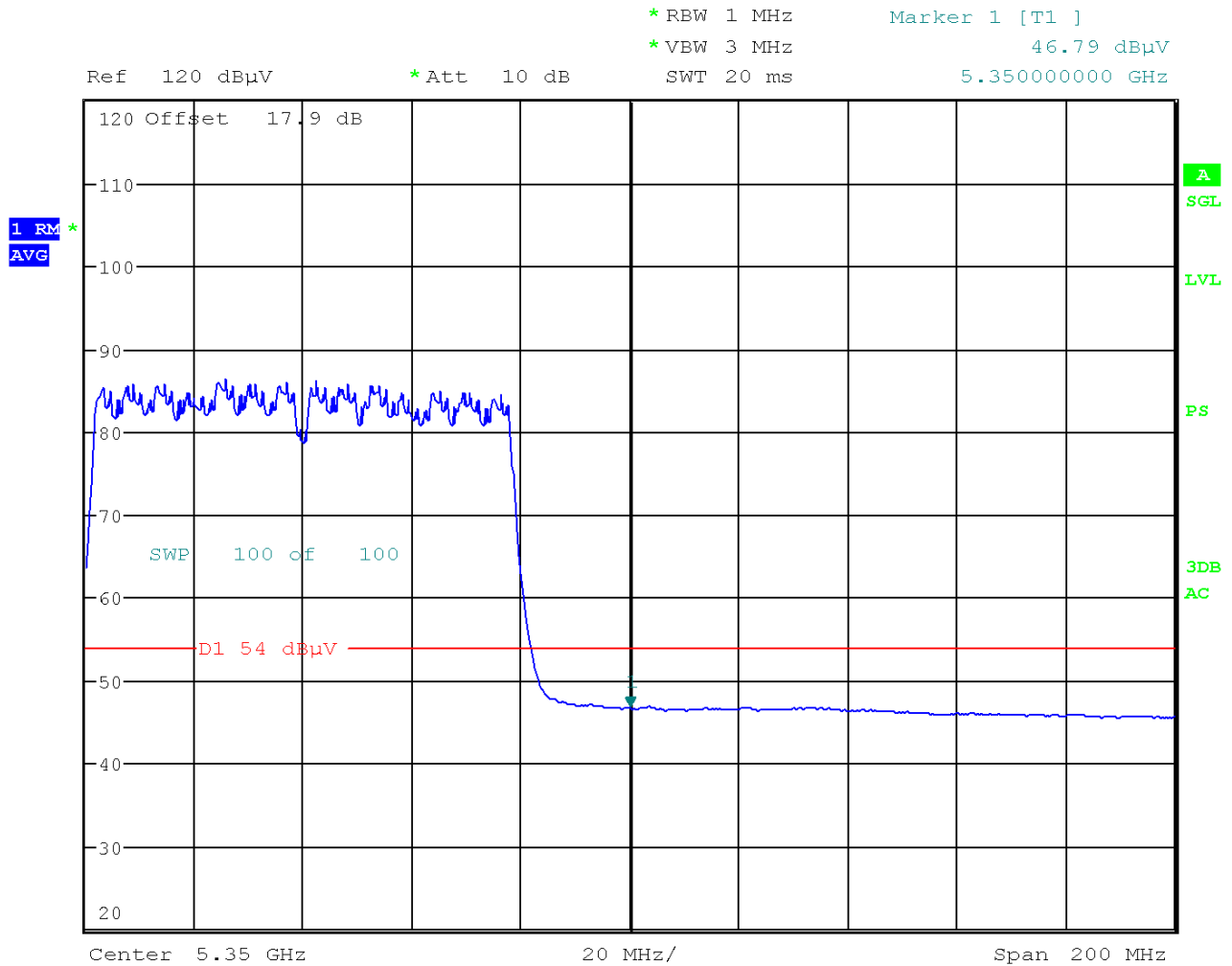
Plot 6-17. Radiated Restricted Upper Band Edge Plot (Average - UNII Band 2A)
