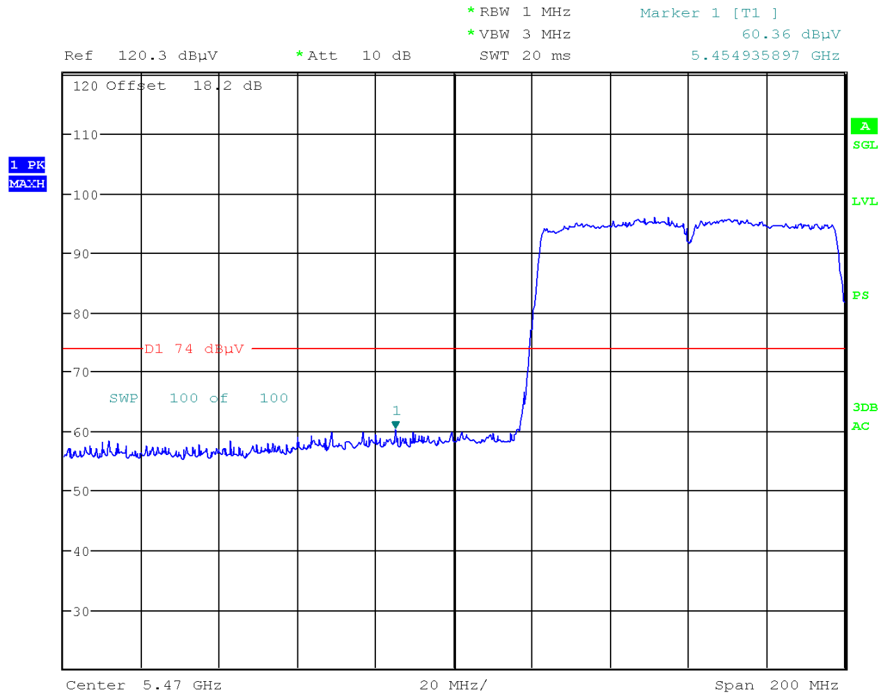
Plot 6-20. Radiated Restricted Lower Band Edge Plot (Peak – UNII Band 2C)
