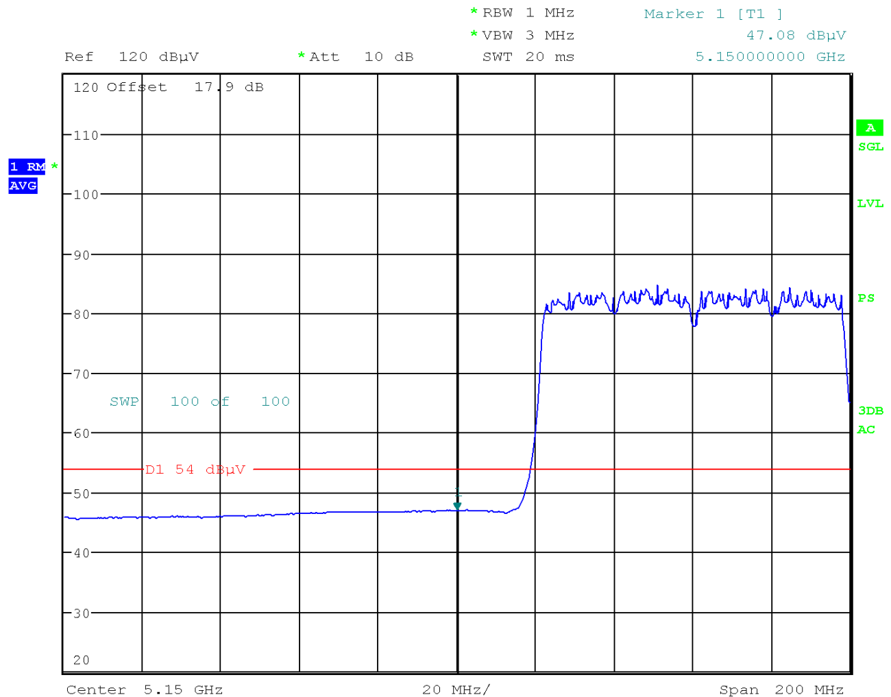
Plot 6-15. Radiated Restricted Lower Band Edge Plot (Average – UNII Band 1)
