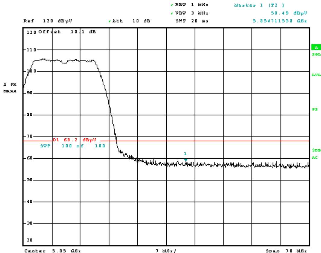
Plot 6-7. Radiated Upper Band Edge Plot (Peak – UNII Band 3)
