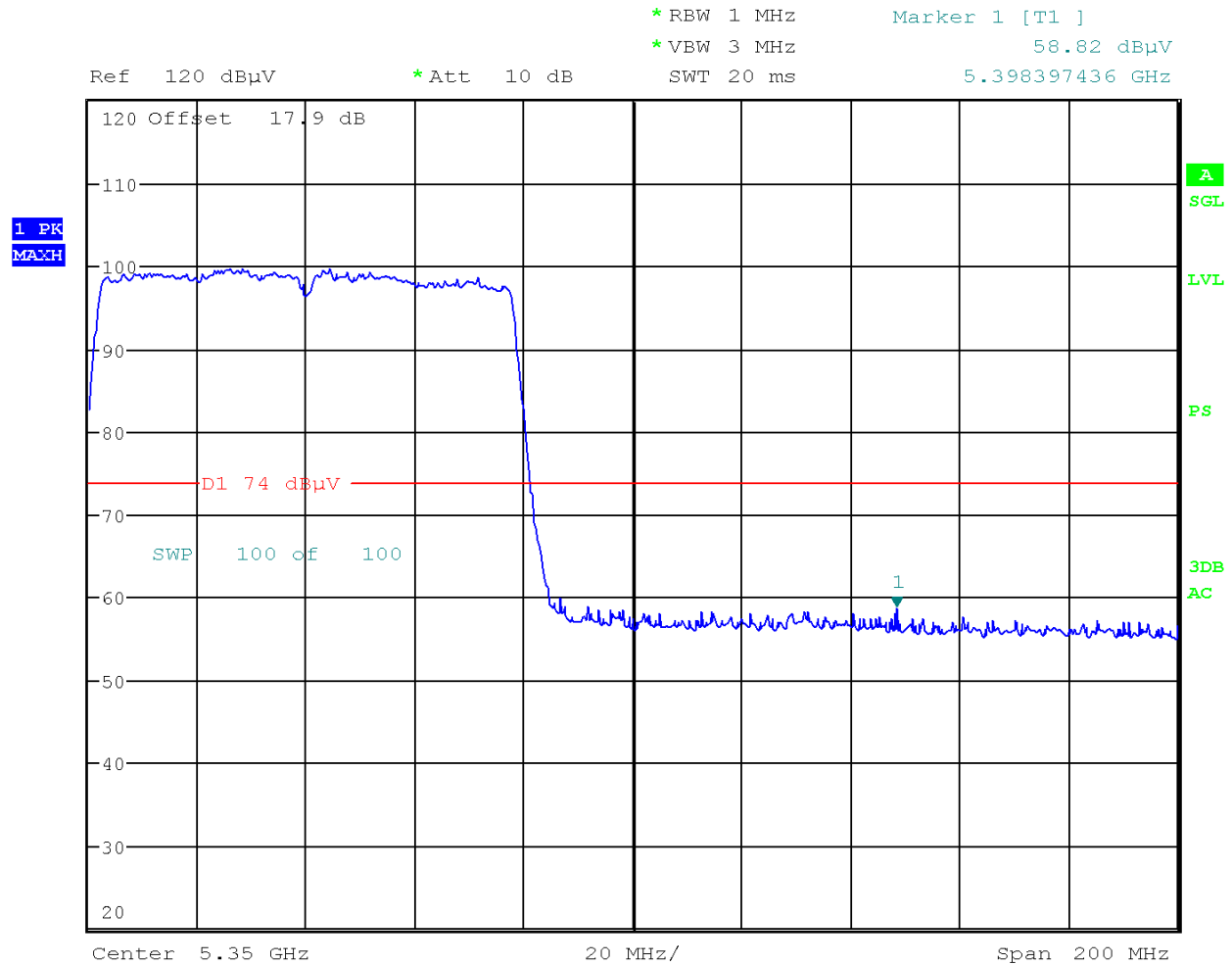
Plot 6-18. Radiated Restricted Upper Band Edge Plot (Peak – UNII Band 2A)
