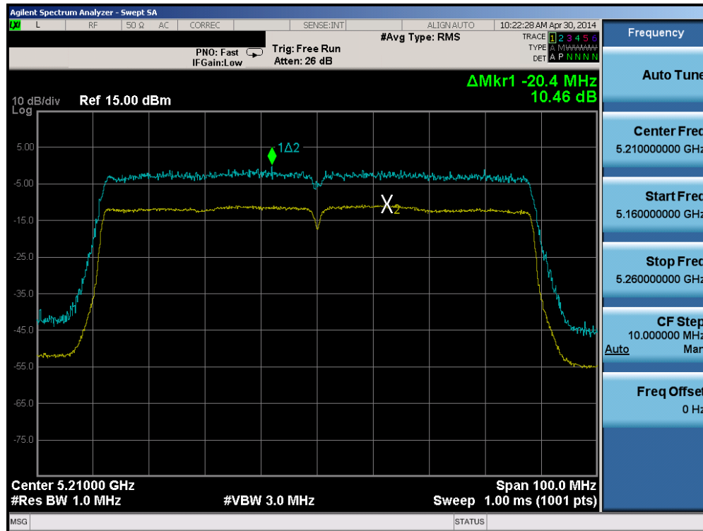
Plot 6-84. Peak Excursion Ratio Plot (80MHz BW 802.11ac (UNII Band 1) – Ch. 42)
