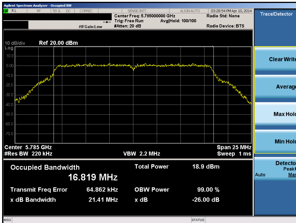
Plot 6-30. 26dB Bandwidth Plot (802.11a (UNII Band 3) – Ch. 157)
