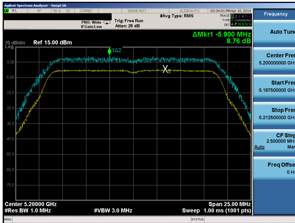
Plot 6-82. Peak Excursion Ratio Plot (20MHz BW 802.11n (UNII Band 1) – Ch. 40)
