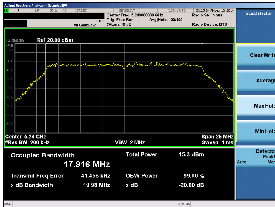
Plot 6-39. 20dB Bandwidth Plot (20MHz BW 802.11n (UNII Band 1) – Ch. 48)
