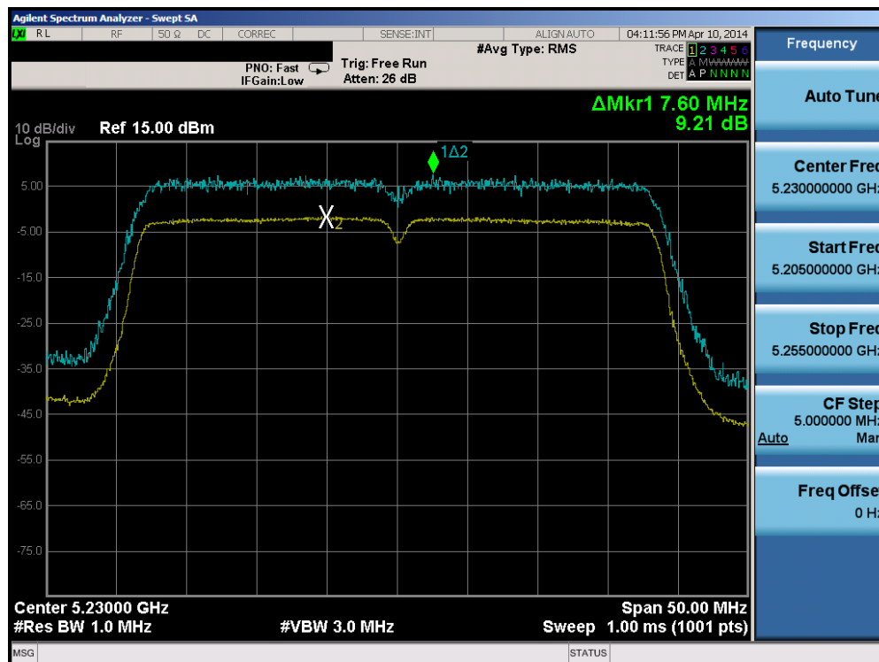
Plot 6-83. Peak Excursion Ratio Plot (40MHz BW 802.11n (UNII Band 1) – Ch. 46)
