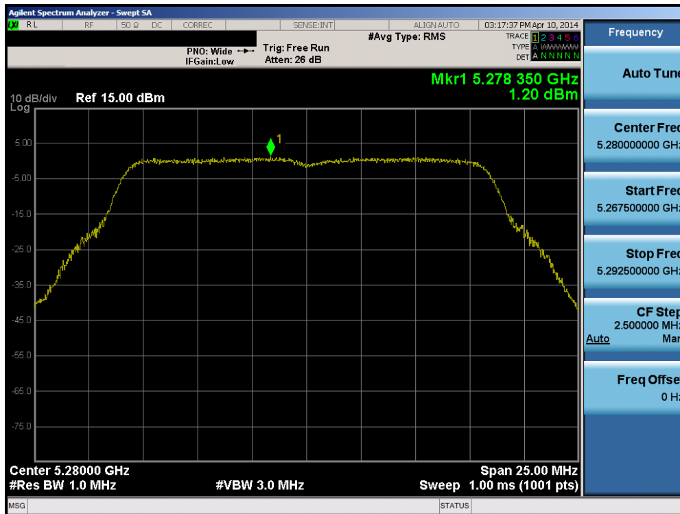
Plot 6-54. Peak Power Spectral Density Plot (802.11a (UNII Band 2A) – Ch. 56)
