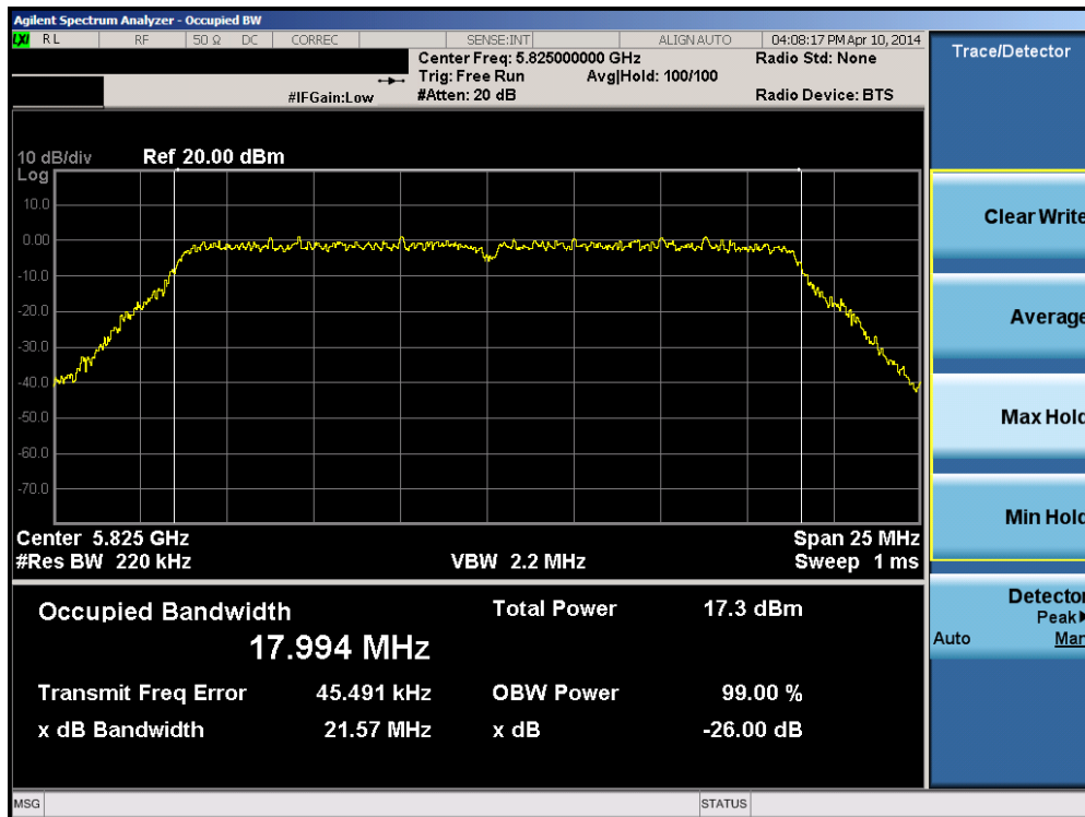
Plot 6-34. 26dB Bandwidth Plot (20MHz BW 802.11n (UNII Band 3) – Ch. 165)
