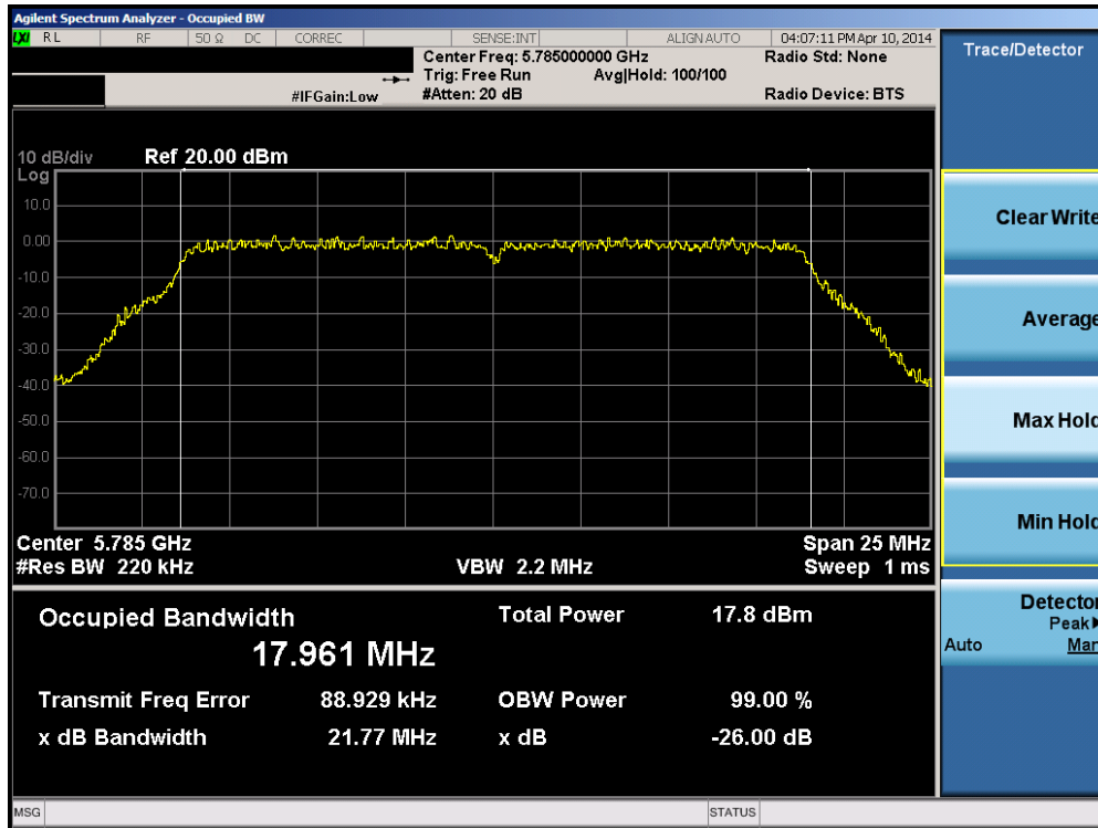
Plot 6-33. 26dB Bandwidth Plot (20MHz BW 802.11n (UNII Band 3) – Ch. 157)
