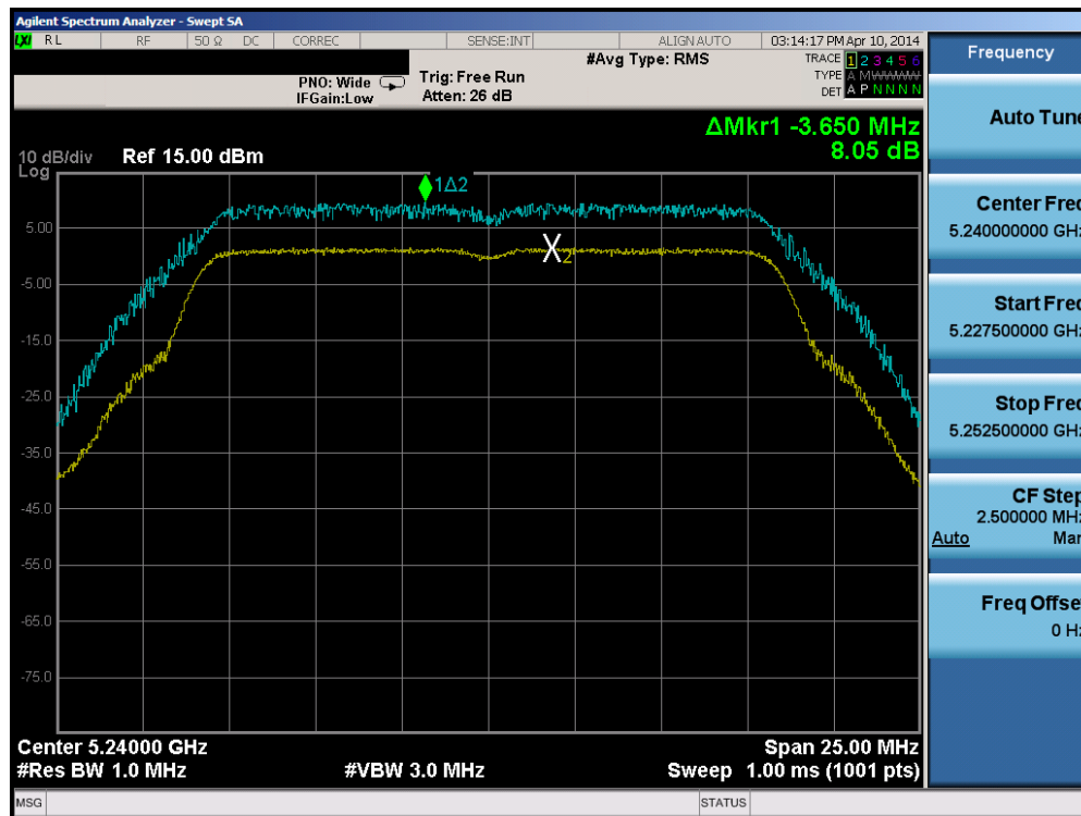
Plot 6-81. Peak Excursion Ratio Plot (802.11a (UNII Band 1) – Ch. 48)
