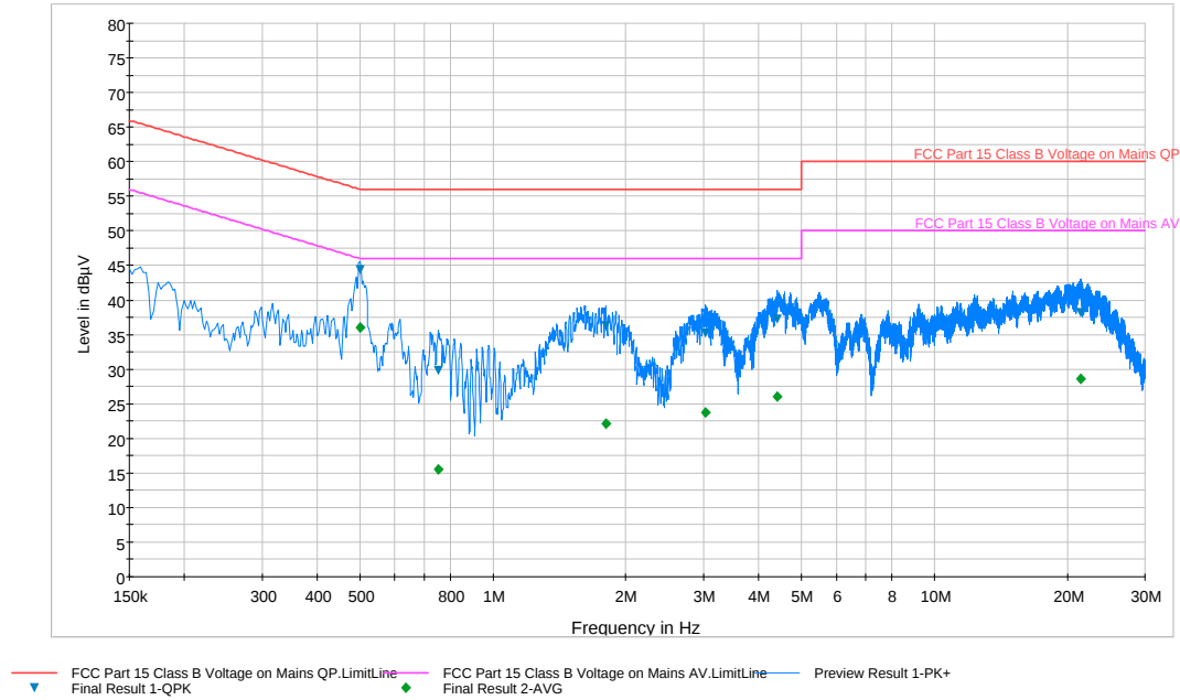
Plot 6-112. Line Conducted Plot with 802.11a UNII Band 1 (L1)
