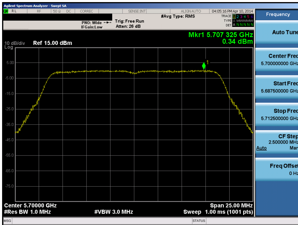
Plot 6-67. Peak Power Spectral Density Plot (20MHz BW 802.11n (UNII Band 2C) – Ch. 140)
