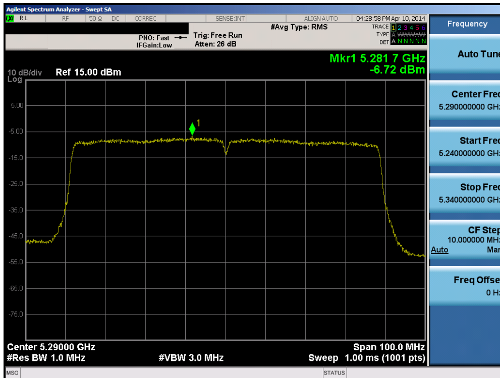
Plot 6-61. Peak Power Spectral Density Plot (80MHz BW 802.11ac (UNII Band 2A) – Ch. 58)
