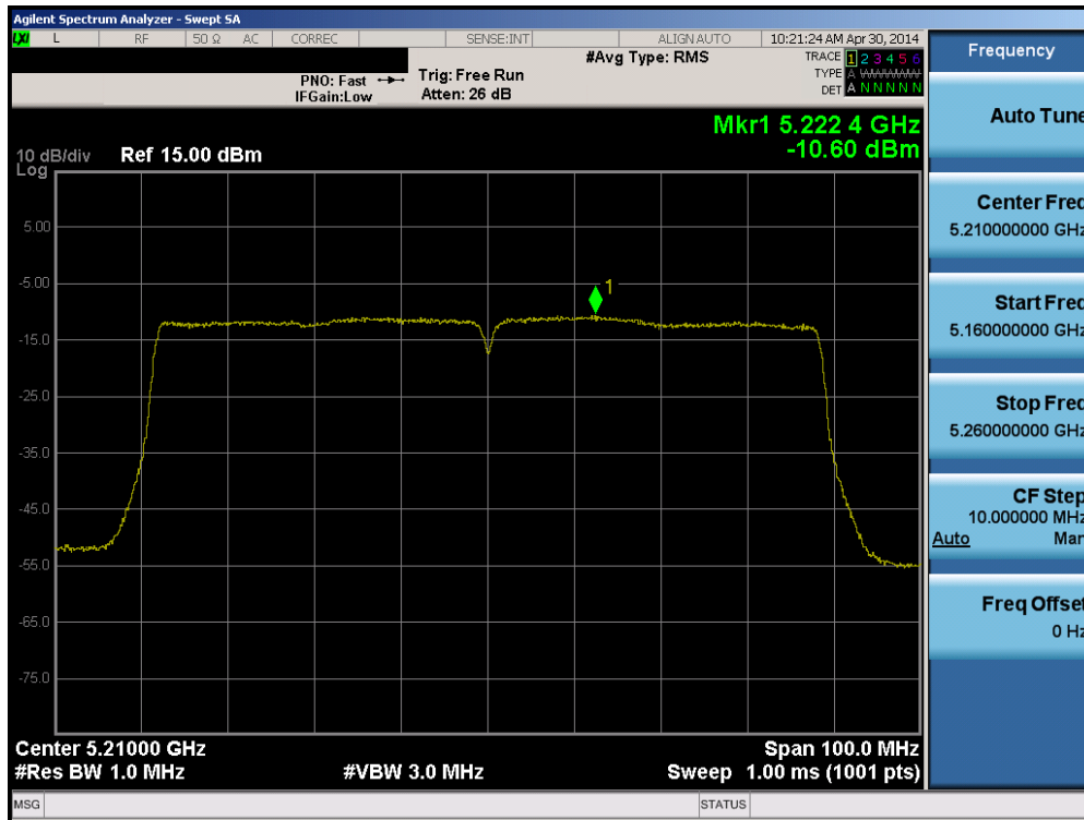
Plot 6-52. Peak Power Spectral Density Plot (80MHz BW 802.11ac (UNII Band 1) – Ch. 42)
