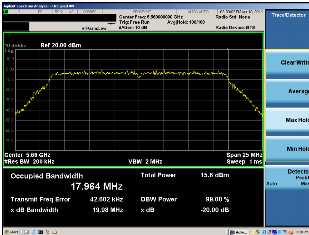
Plot 6-40. 20dB Bandwidth Plot (20MHz BW 802.11n (UNII Band 2C) – Ch. 132)
