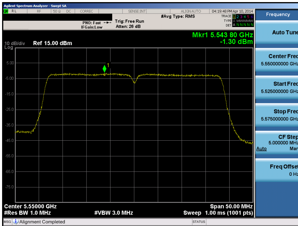
Plot 6-69. Peak Power Spectral Density Plot (40MHz BW 802.11n (UNII Band 2C) – Ch. 110)
