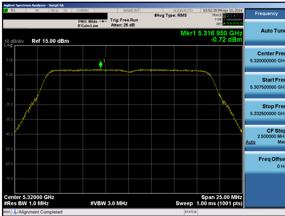
Plot 6-58. Peak Power Spectral Density Plot (20MHz BW 802.11n (UNII Band 2A) – Ch. 64)
