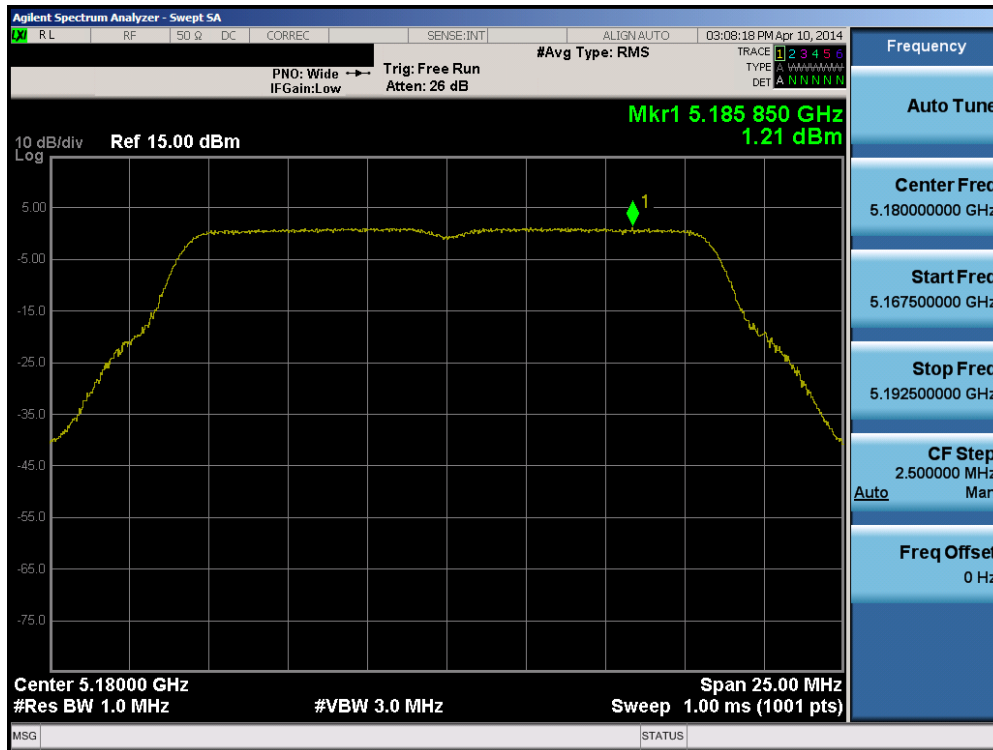
Plot 6-44. Peak Power Spectral Density Plot (802.11a (UNII Band 1) – Ch. 36)
