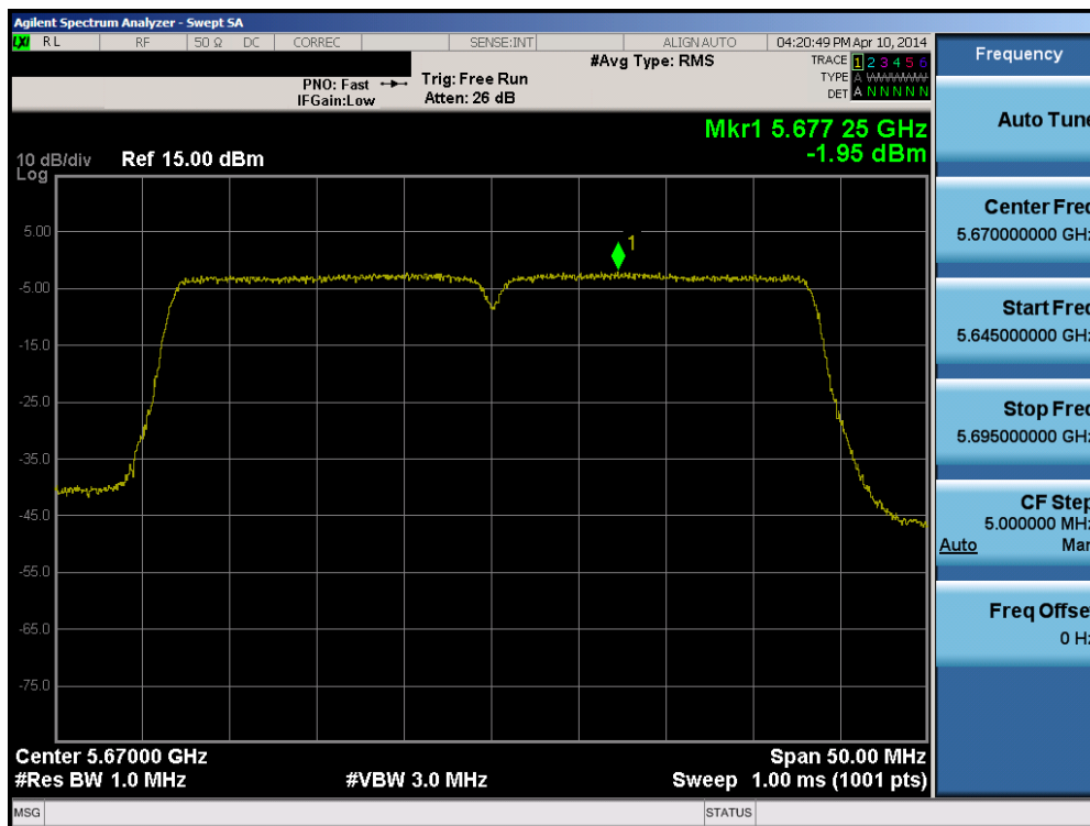
Plot 6-70. Peak Power Spectral Density Plot (40MHz BW 802.11n (UNII Band 2C) – Ch. 134)
