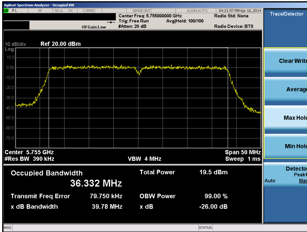
Plot 6-35. 26dB Bandwidth Plot (40MHz BW 802.11n (UNII Band 3) – Ch. 151)
