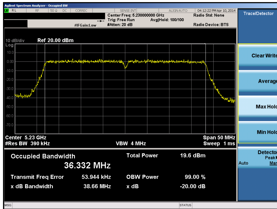
Plot 6-41. 20dB Bandwidth Plot (40MHz BW 802.11n (UNII Band 1) – Ch. 46)
