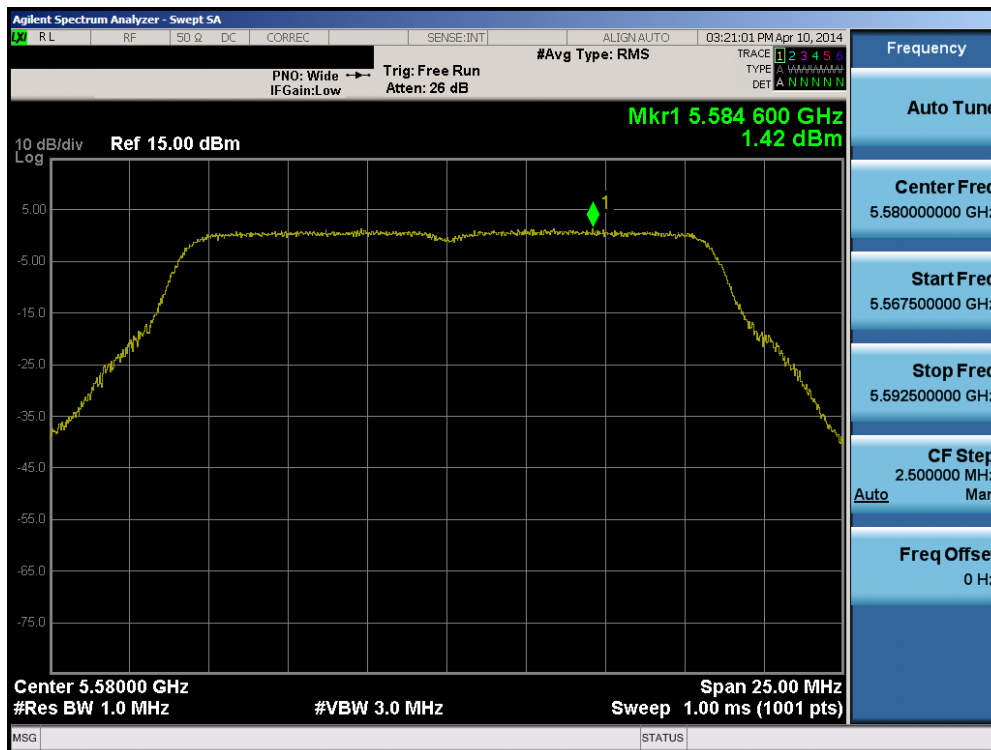
Plot 6-63. Peak Power Spectral Density Plot (802.11a (UNII Band 2C) – Ch. 116)
