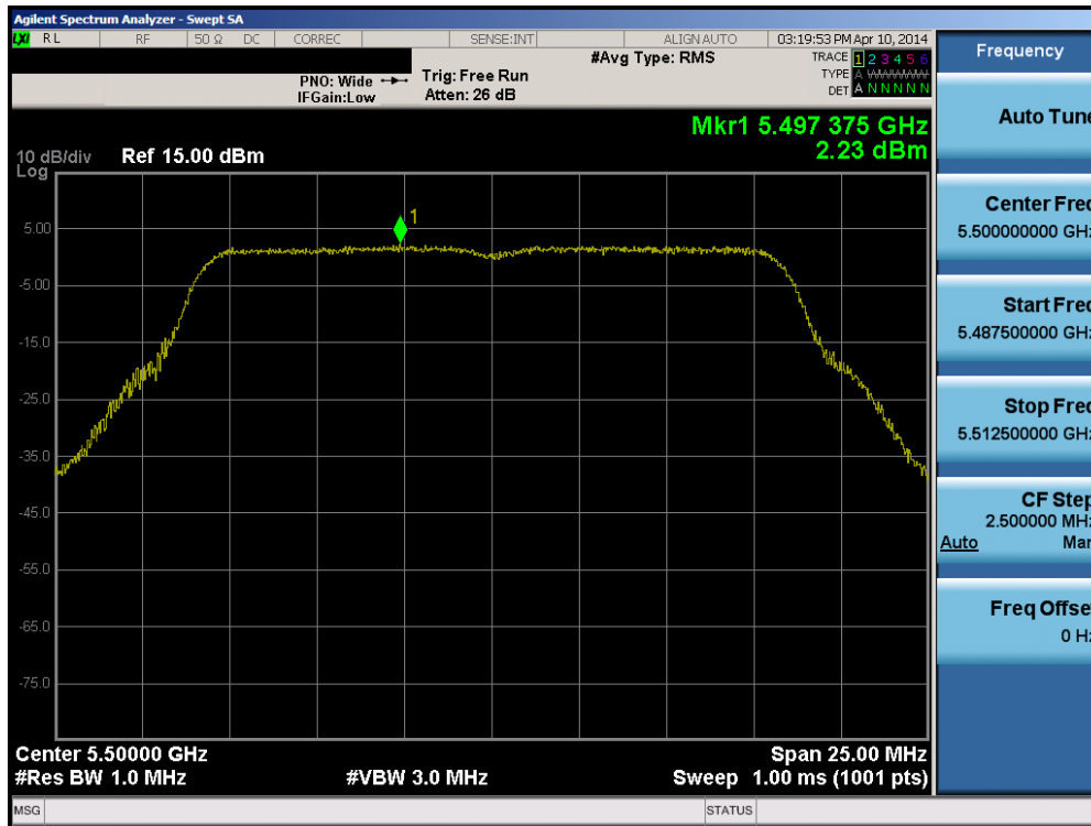
Plot 6-62. Peak Power Spectral Density Plot (802.11a (UNII Band 2C) – Ch. 100)
