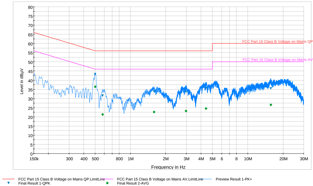
Plot 6-116. Line Conducted Plot with 802.11a UNII Band 2C (L1)
