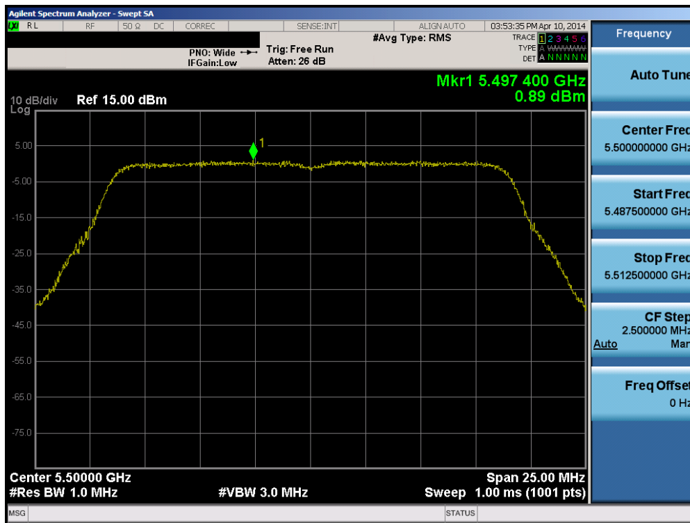
Plot 6-65. Peak Power Spectral Density Plot (20MHz BW 802.11n (UNII Band 2C) – Ch. 100)
