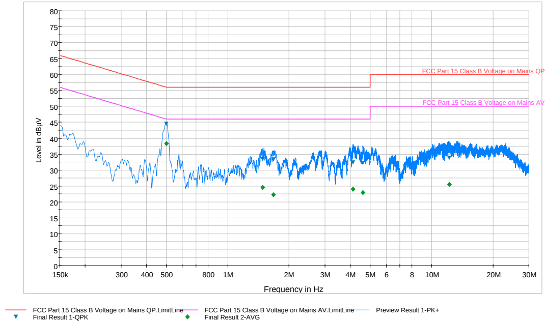
Plot 6-119. Line Conducted Plot with 802.11a UNII Band 3 (N)
