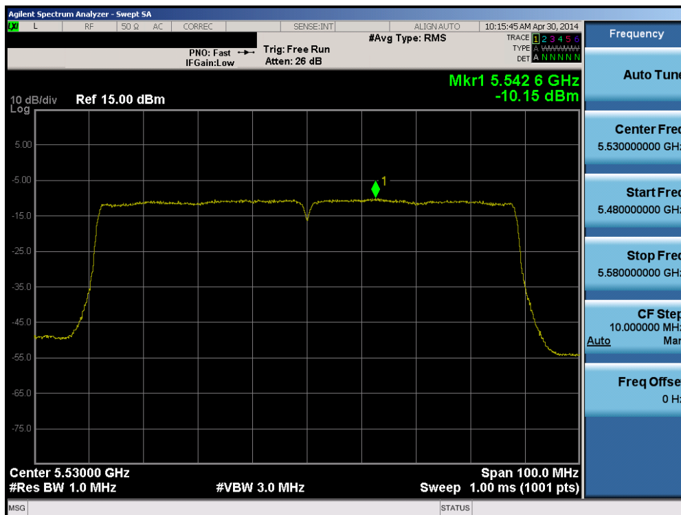
Plot 6-71. Peak Power Spectral Density Plot (80MHz BW 802.11ac (UNII Band 2C) – Ch. 106)
