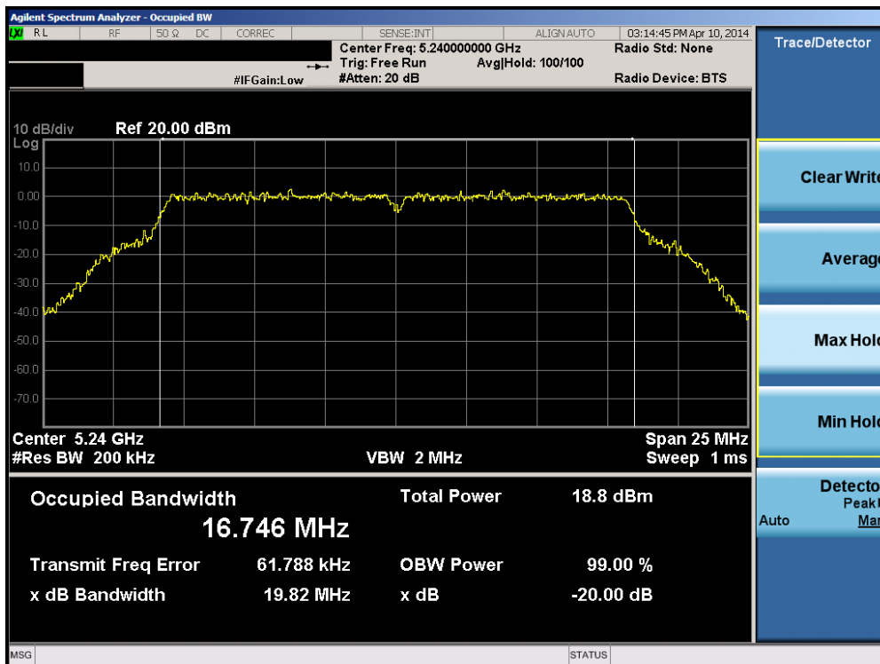
Plot 6-38. 20dB Bandwidth Plot (20MHz BW 802.11a (UNII Band 1) – Ch. 48)
