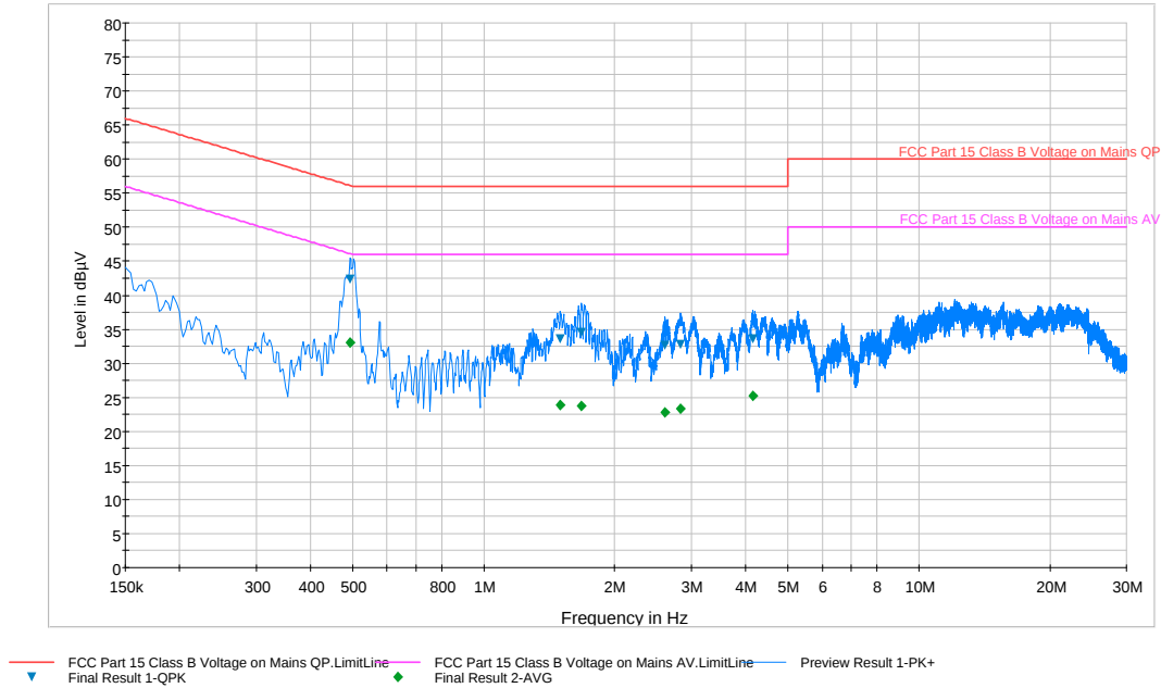
Plot 6-115. Line Conducted Plot with 802.11a UNII Band 2A (N)
