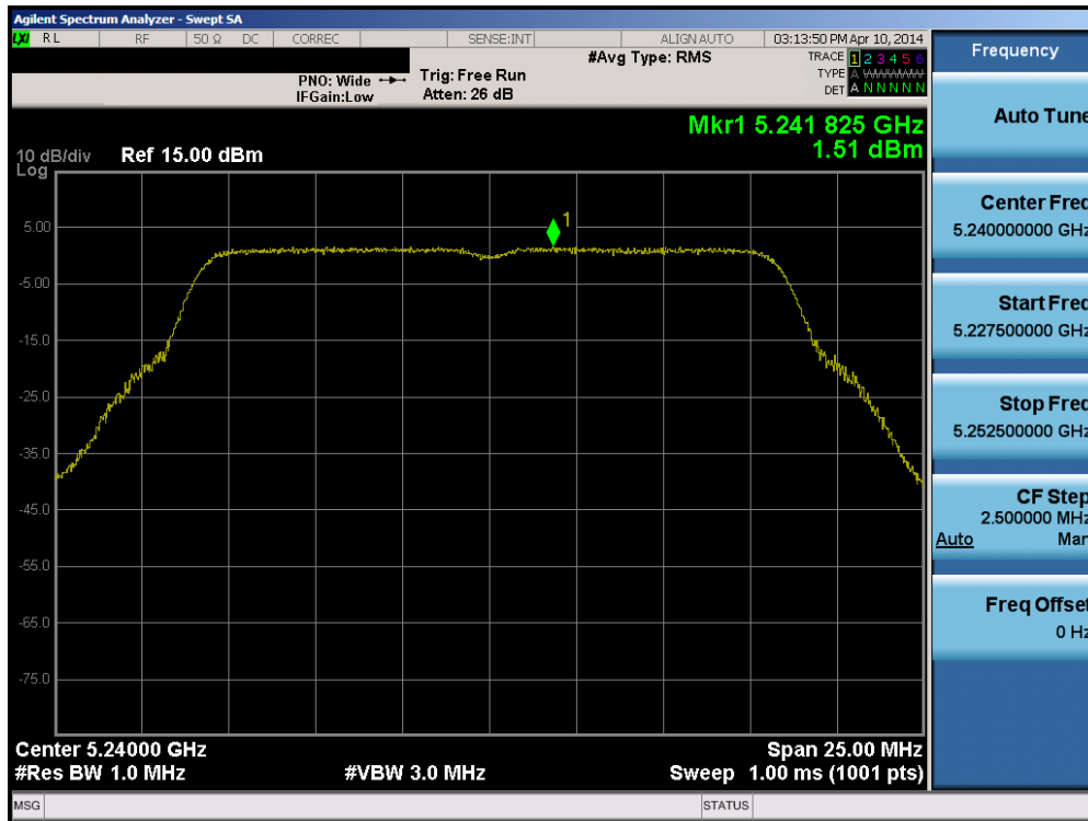
Plot 6-46. Peak Power Spectral Density Plot (802.11a (UNII Band 1) – Ch. 48)
