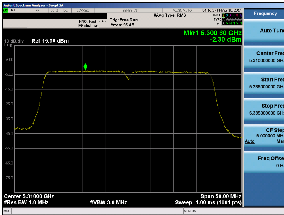
Plot 6-60. Peak Power Spectral Density Plot (40MHz BW 802.11n (UNII Band 2A) – Ch. 62)
