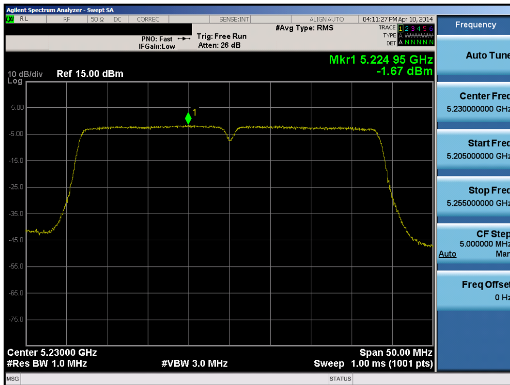
Plot 6-51. Peak Power Spectral Density Plot (40MHz BW 802.11n (UNII Band 1) – Ch. 46)
