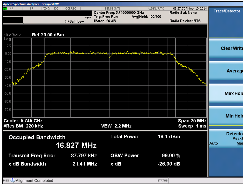
Plot 6-29. 26dB Bandwidth Plot (802.11a (UNII Band 3) – Ch. 149)
