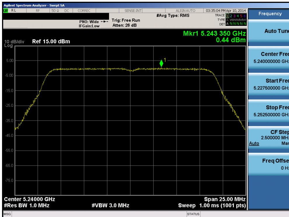
Plot 6-49. Peak Power Spectral Density Plot (20MHz BW 802.11n (UNII Band 1) – Ch. 48)
