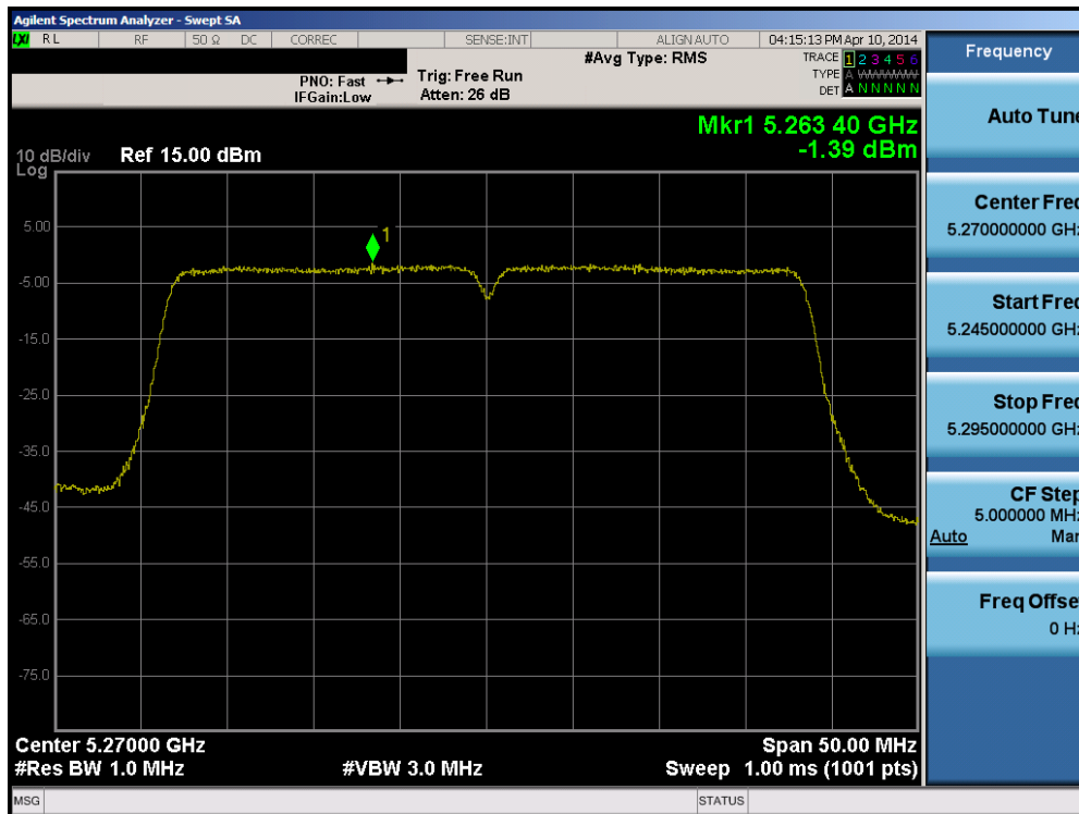
Plot 6-59. Peak Power Spectral Density Plot (40MHz BW 802.11n (UNII Band 2A) – Ch. 54)
