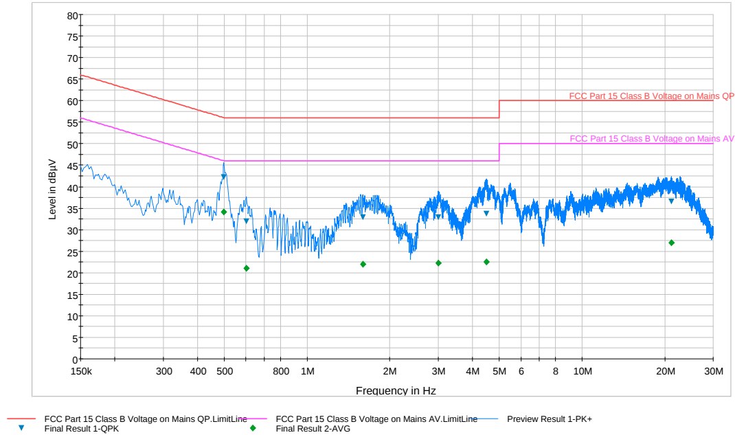
Plot 6-118. Line Conducted Plot with 802.11a UNII Band 3 (L1)
