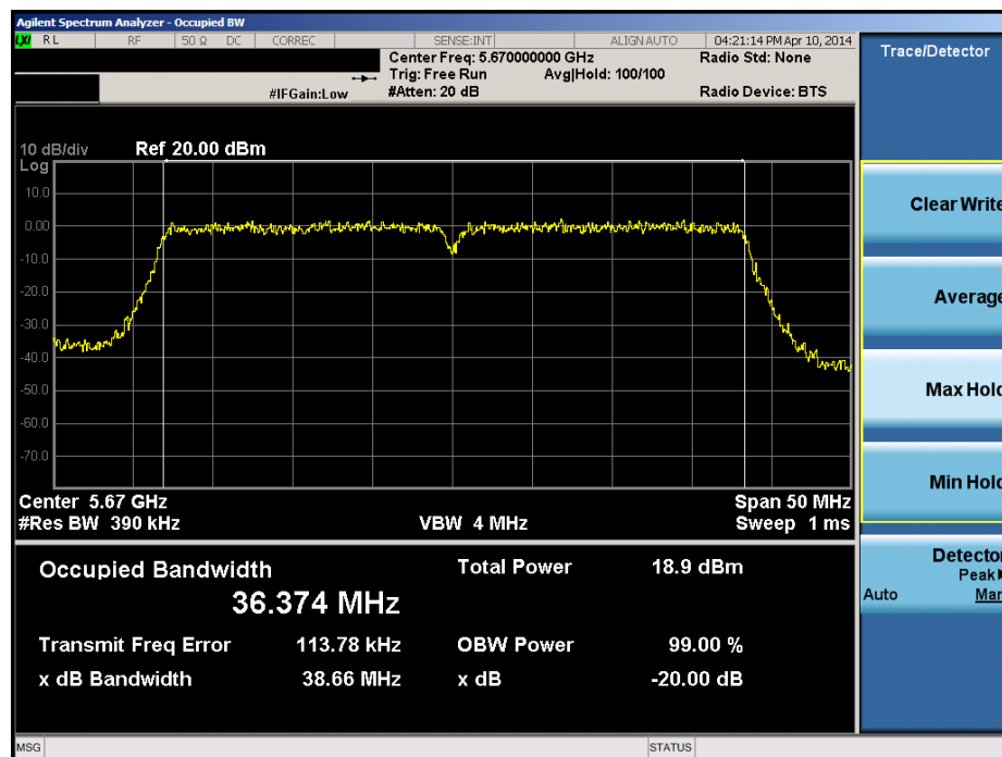
Plot 6-42. 20dB Bandwidth Plot (40MHz BW 802.11n (UNII Band 2C) – Ch. 134)
