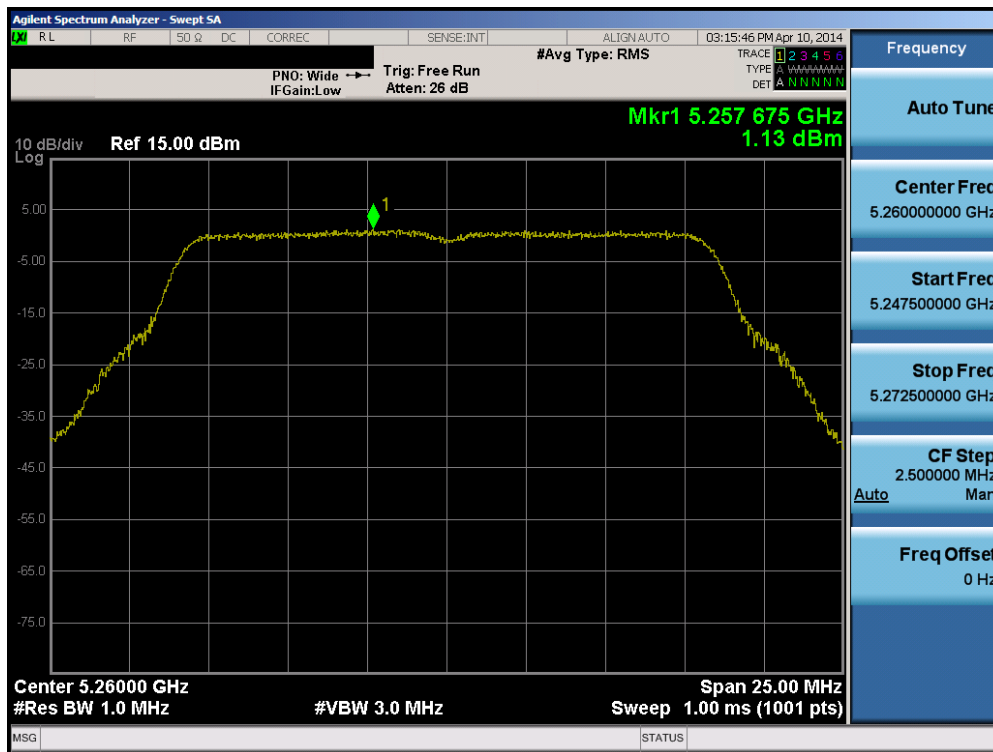
Plot 6-53. Peak Power Spectral Density Plot (802.11a (UNII Band 2A) – Ch. 52)
