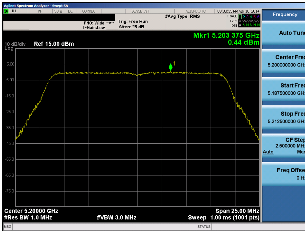
Plot 6-48. Peak Power Spectral Density Plot (20MHz BW 802.11n (UNII Band 1) – Ch. 40)
