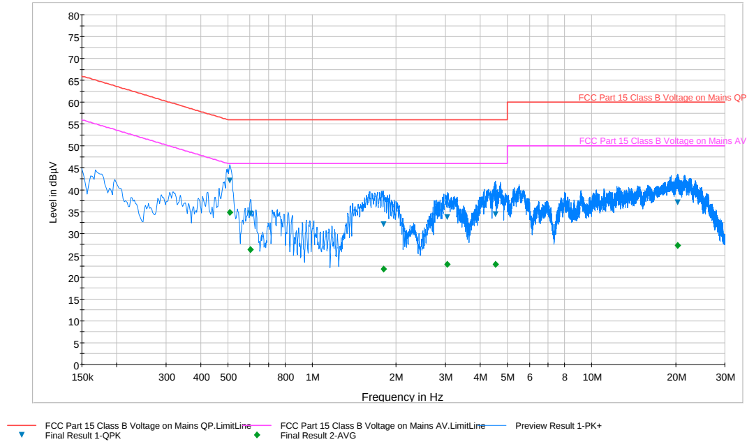
Plot 6-114. Line Conducted Plot with 802.11a UNII Band 2A (L1)
