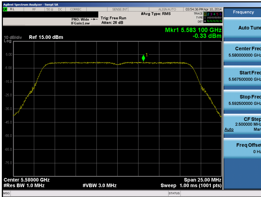
Plot 6-66. Peak Power Spectral Density Plot (20MHz BW 802.11n (UNII Band 2C) – Ch. 116)
