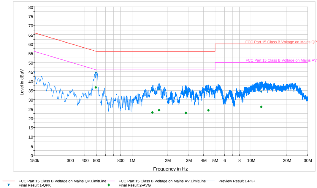
Plot 6-117. Line Conducted Plot with 802.11a UNII Band 2C (N)
