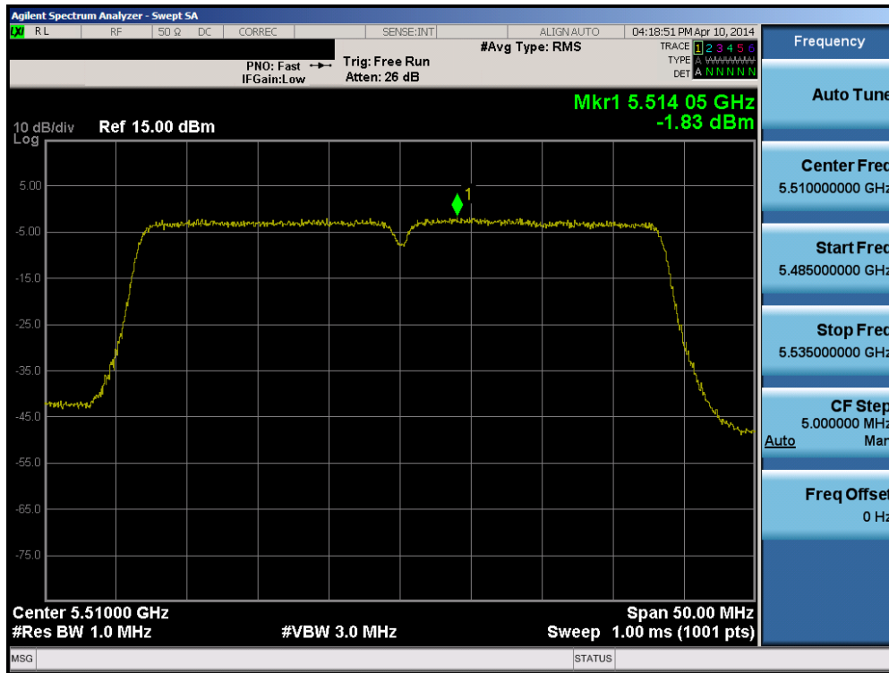
Plot 6-68. Peak Power Spectral Density Plot (40MHz BW 802.11n (UNII Band 2C) – Ch. 102)
