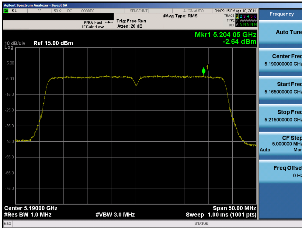
Plot 6-50. Peak Power Spectral Density Plot (40MHz BW 802.11n (UNII Band 1) – Ch. 38)
