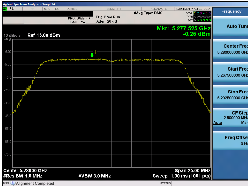
Plot 6-57. Peak Power Spectral Density Plot (20MHz BW 802.11n (UNII Band 2A) – Ch. 56)
