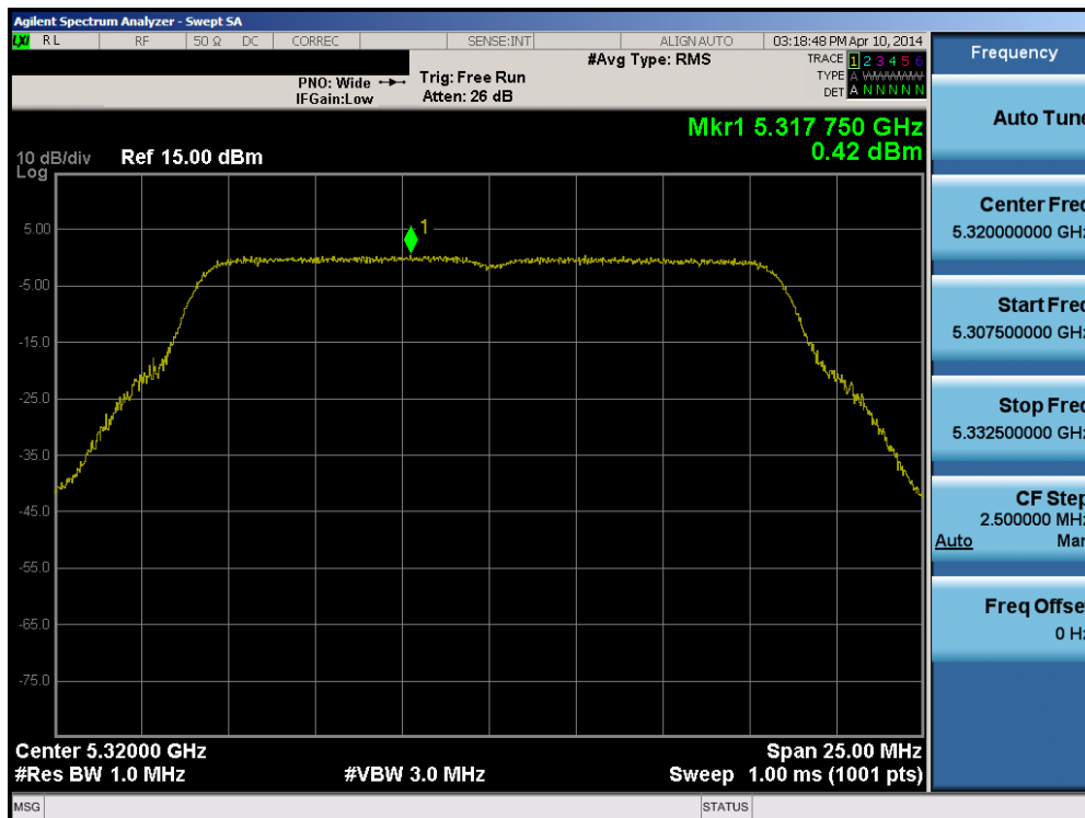
Plot 6-55. Peak Power Spectral Density Plot (802.11a (UNII Band 2A) – Ch. 64)
