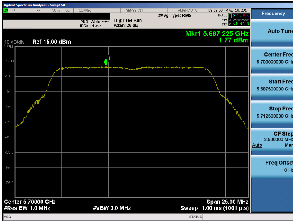
Plot 6-64. Peak Power Spectral Density Plot (802.11a (UNII Band 2C) – Ch. 140)
