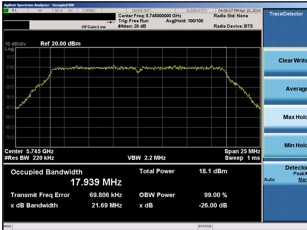
Plot 6-32. 26dB Bandwidth Plot (20MHz BW 802.11n (UNII Band 3) – Ch. 149)
