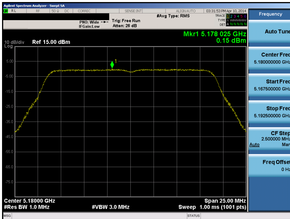
Plot 6-47. Peak Power Spectral Density Plot (20MHz BW 802.11n (UNII Band 1) – Ch. 36)
