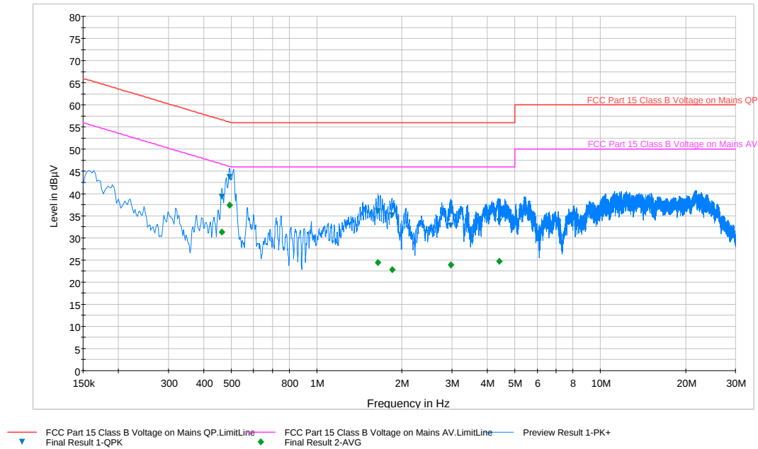
Plot 6-113. Line Conducted Plot with 802.11a UNII Band 1 (N)
