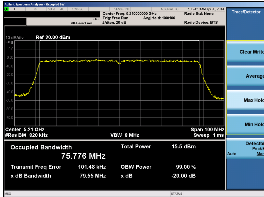
Plot 6-43. 20dB Bandwidth Plot (80MHz BW 802.11ac (UNII Band 1) – Ch. 42)
