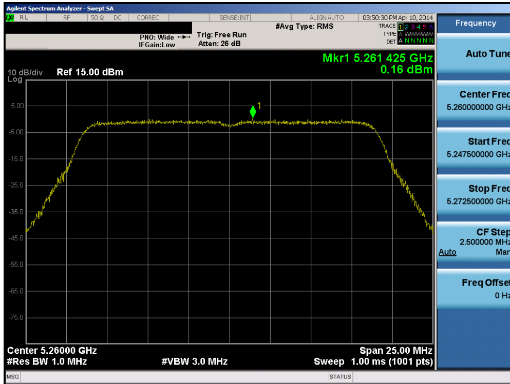
Plot 6-56. Peak Power Spectral Density Plot (20MHz BW 802.11n (UNII Band 2A) – Ch. 52)
