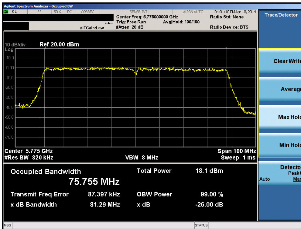
Plot 6-37. 26dB Bandwidth Plot (80MHz BW 802.11ac (UNII Band 3) – Ch. 155)
