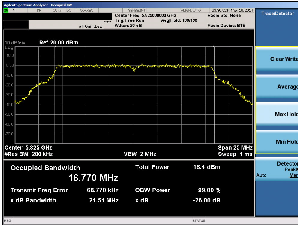
Plot 6-31. 26dB Bandwidth Plot (802.11a (UNII Band 3) – Ch. 165)
