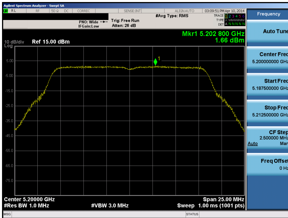
Plot 6-45. Peak Power Spectral Density Plot (802.11a (UNII Band 1) – Ch. 40)
