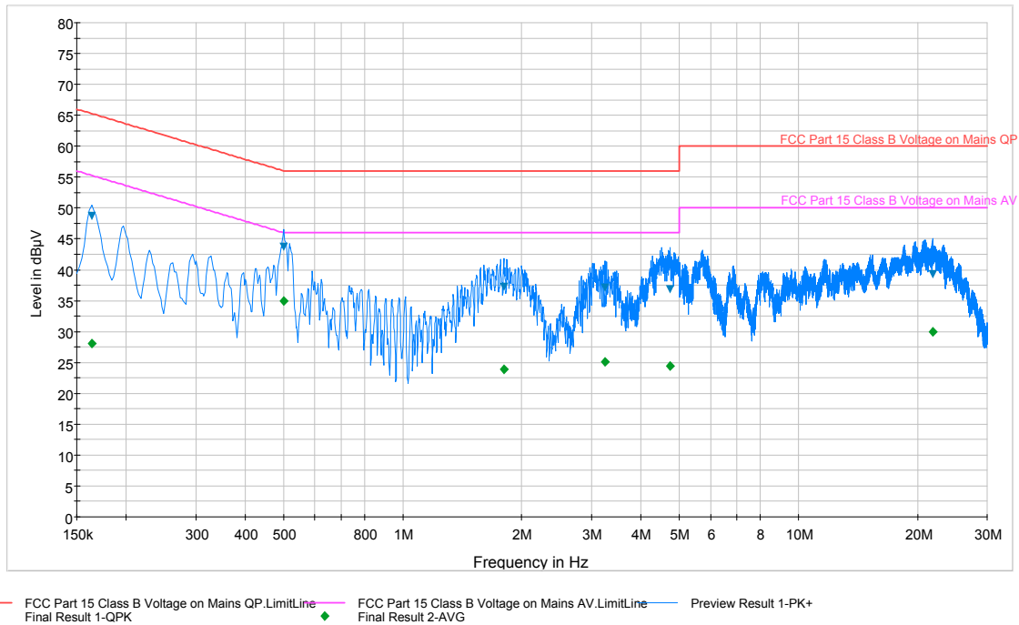
Plot 6-37. Line Conducted Plot with 802.11b (L1)
