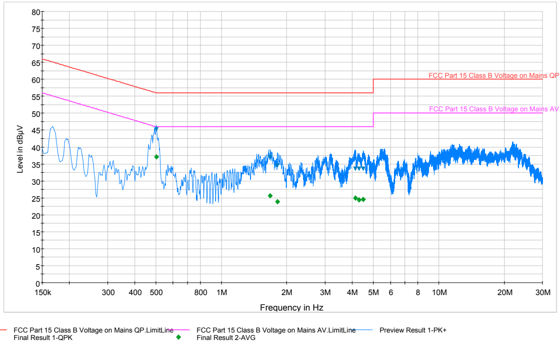
Plot 6-38. Line Conducted Plot with 802.11b (N)
