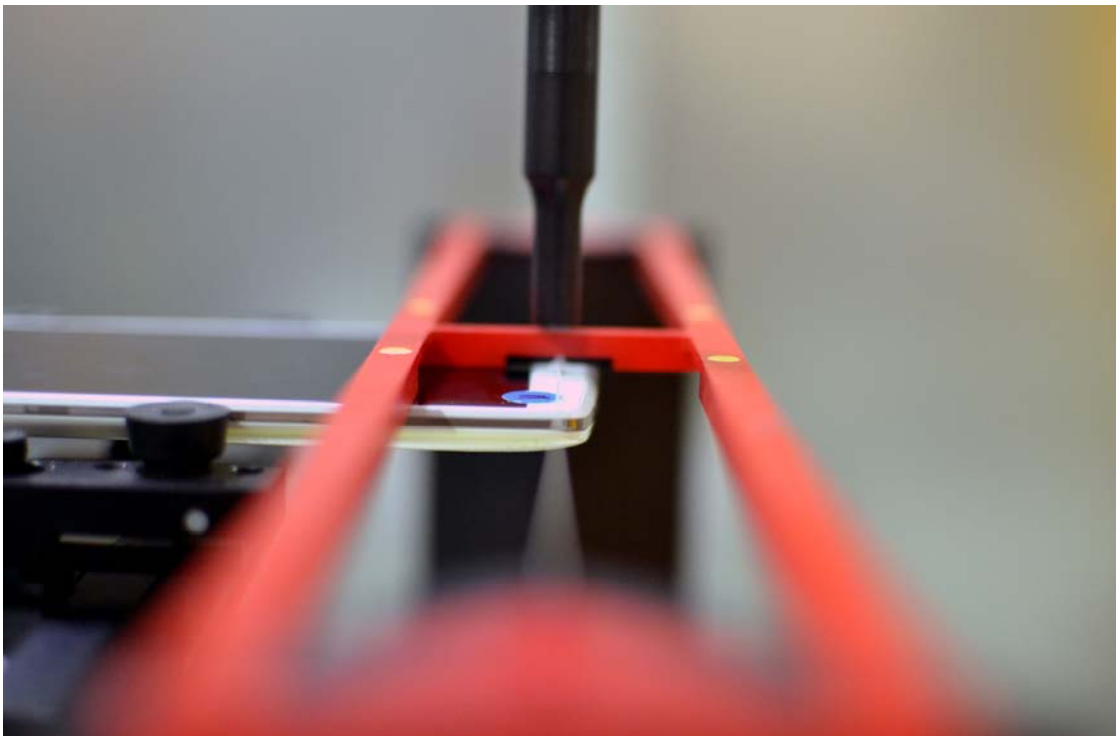
Figure 18-4 HAC Phantom Plane Alignment
