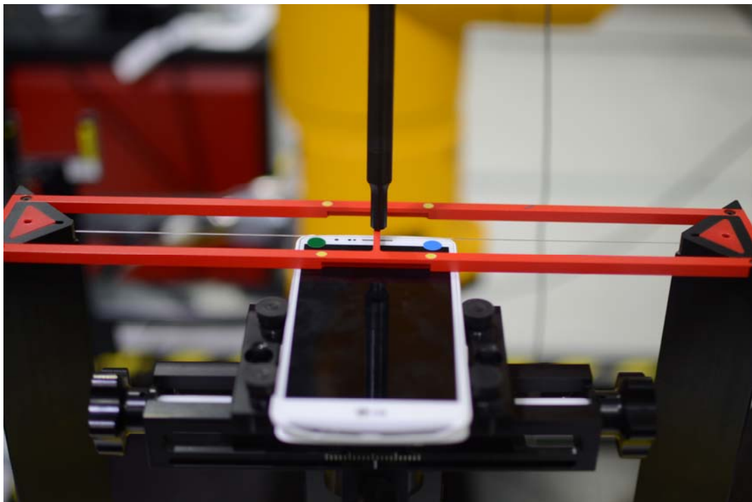
Figure 18-2 Ear Reference Point HAC Phantom Alignment, Inductive Charging Battery Cover (Cover Open)
