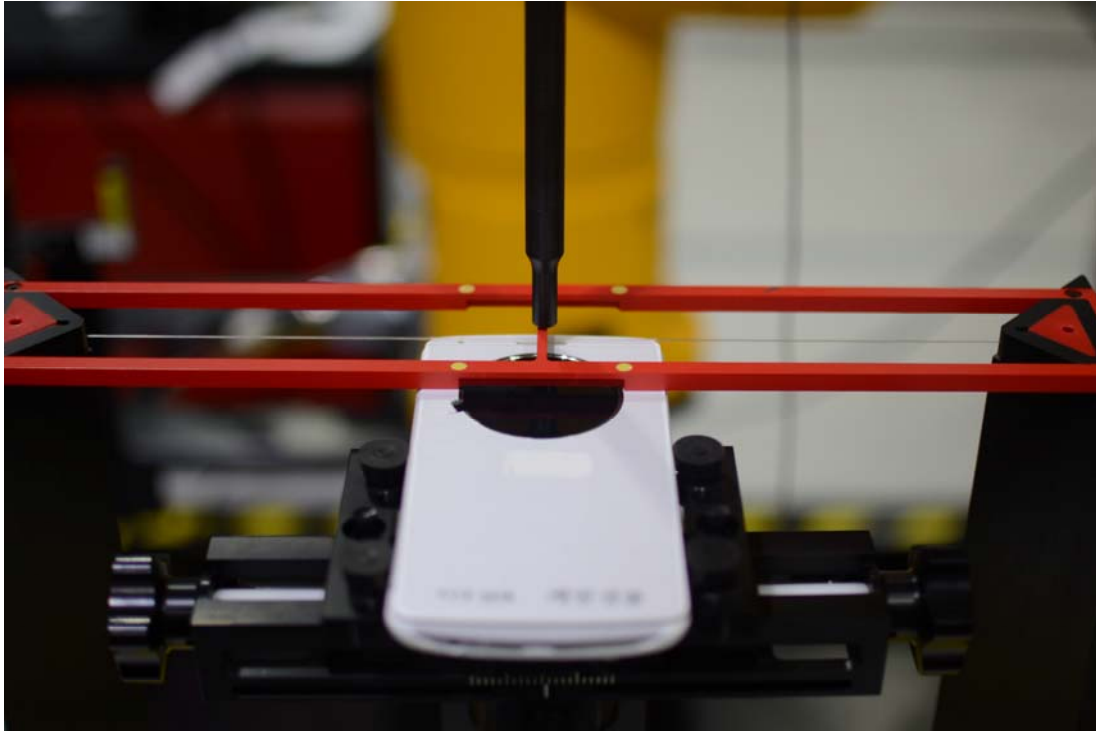
Figure 18-3 Ear Reference Point HAC Phantom Alignment, Inductive Charging Battery Cover (Cover Closed)
