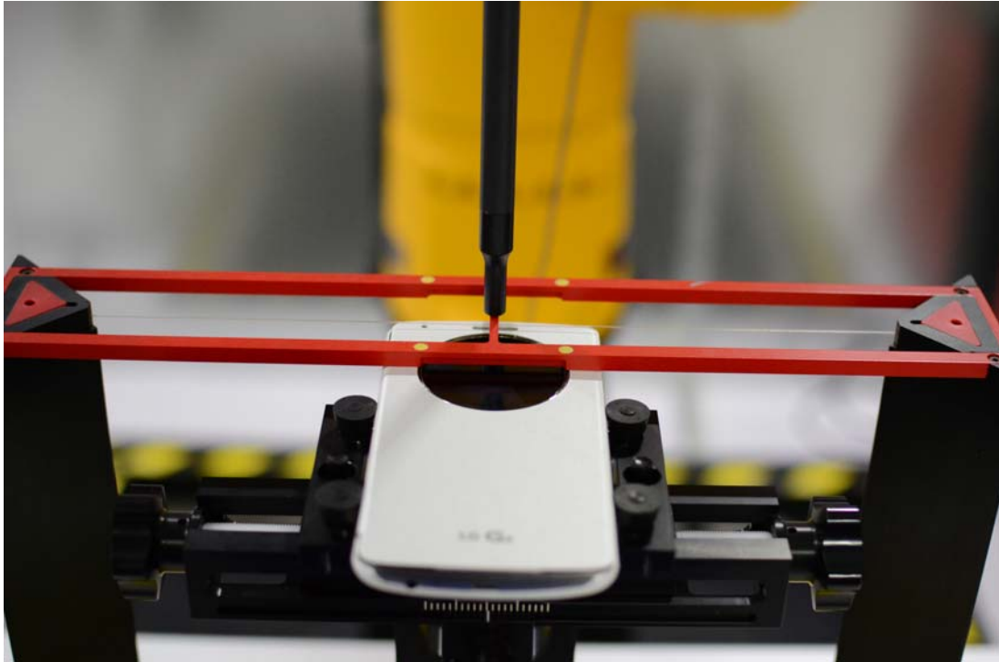
Figure 18-3 Ear Reference Point HAC Phantom Alignment (Wireless Charging Case – Closed)
