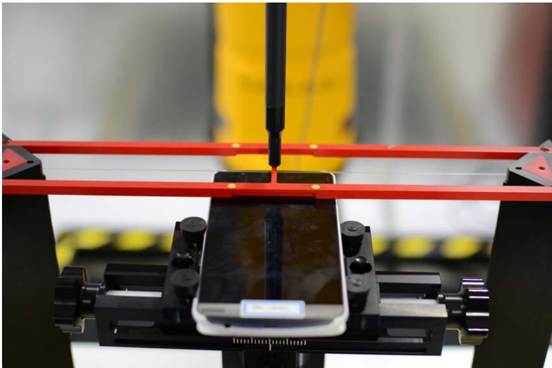
Figure 18-2 Ear Reference Point HAC Phantom Alignment (Wireless Charging Case – Open)
