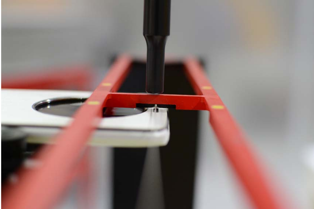
Figure 18-7 HAC Phantom Plane Alignment (Wireless Charging Case – Closed)
