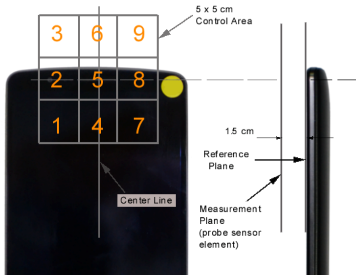
Figure 18-9 5x5 Scan grid above WD
