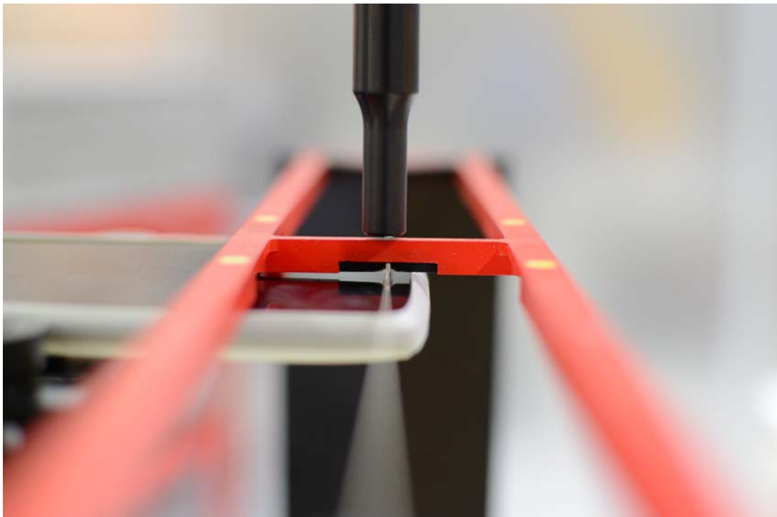
Figure 18-8 HAC Phantom Plane Alignment (Wireless Charging Cover)
