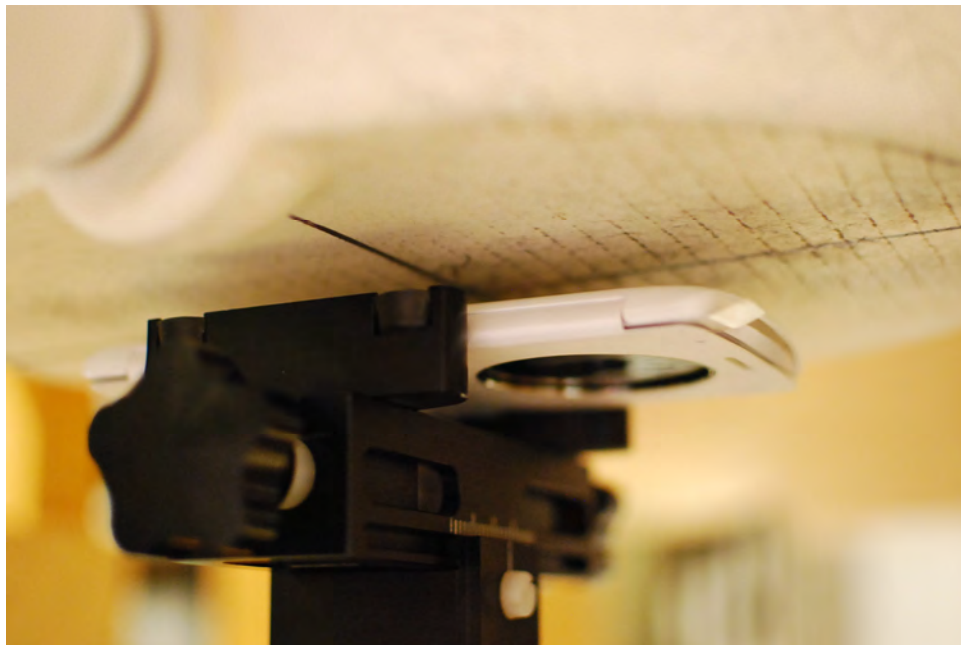
SAR Test Setup Photo 13 – Back Side, Wireless Charging Cover, Case Closed at 1.0 cm
