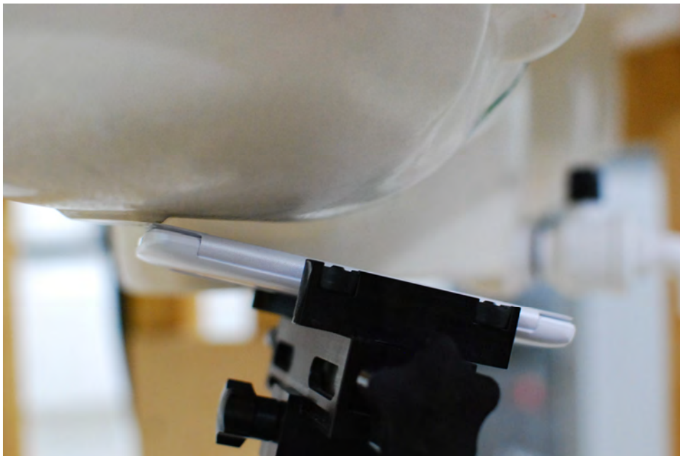
SAR Test Setup Photo 5 – Right Tilt, Wireless Charging Cover, Closed Case
