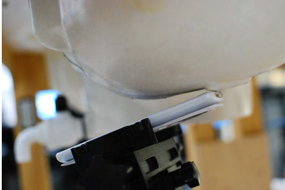
SAR Test Setup Photo 10 – Left Tilt, Wireless Charging Cover, Case Open
