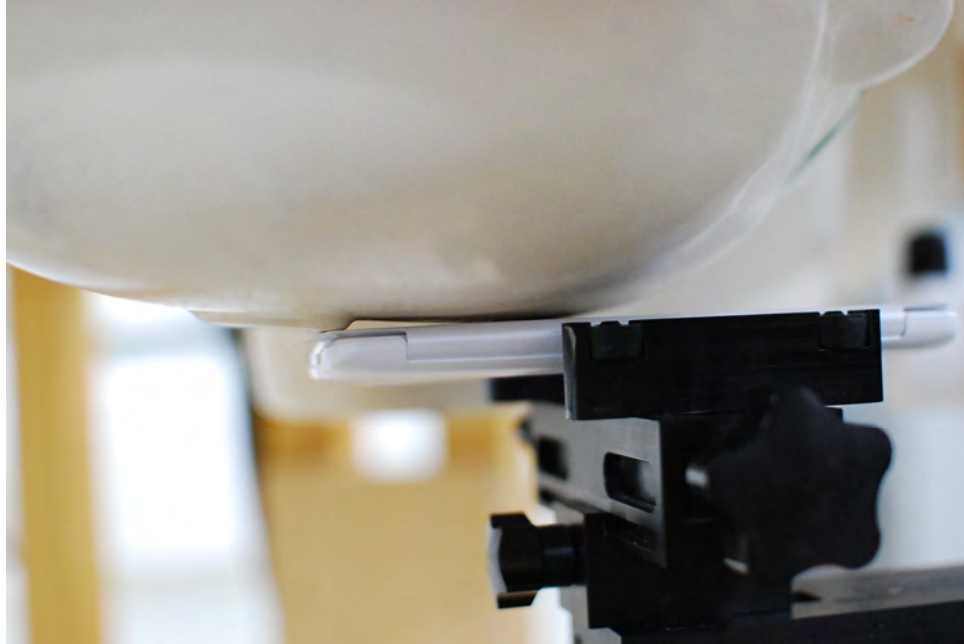
SAR Test Setup Photo 3 – Right Cheek, Wireless Charging Cover, Closed Case
