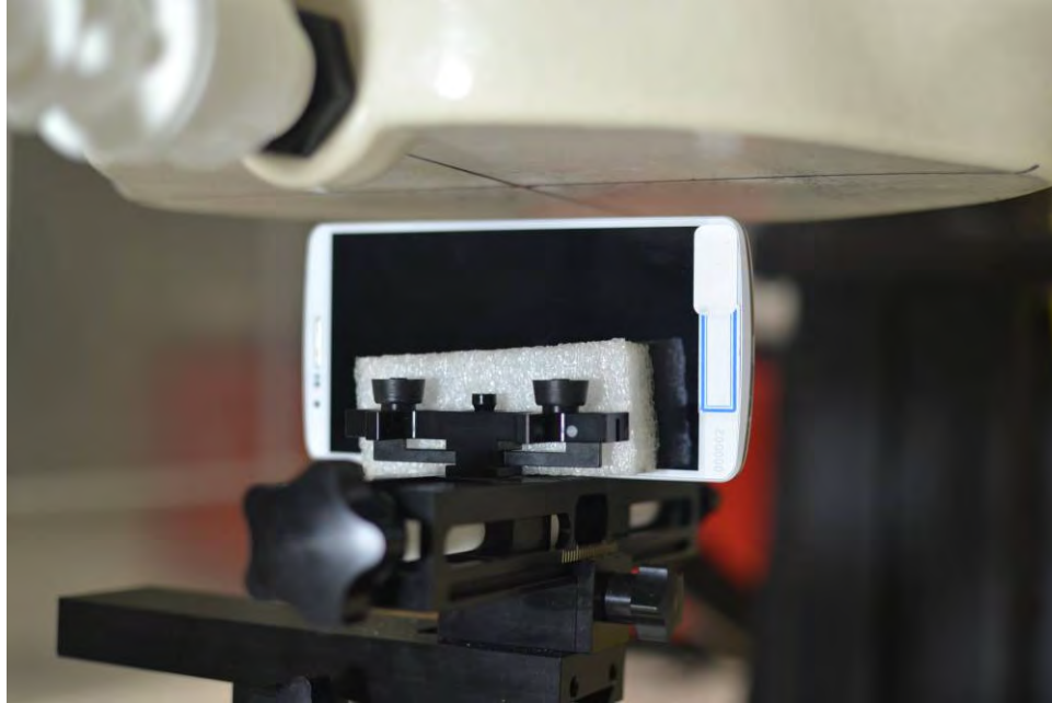
SAR Test Setup Photo 18 – Right Edge, Standard Cover at 1.0 cm
