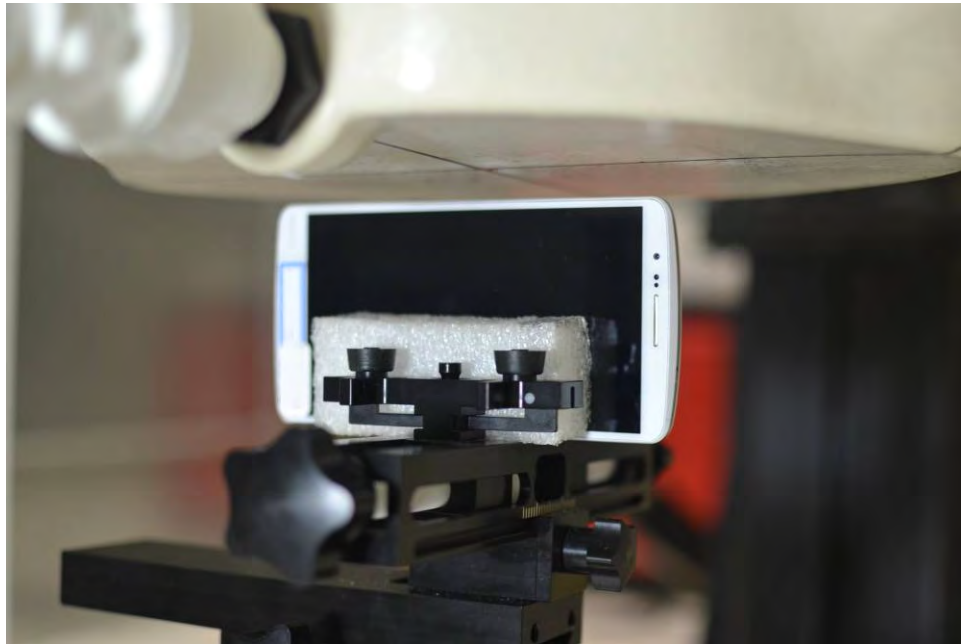
SAR Test Setup Photo 19 – Left Edge, Standard Cover at 1.0 cm
