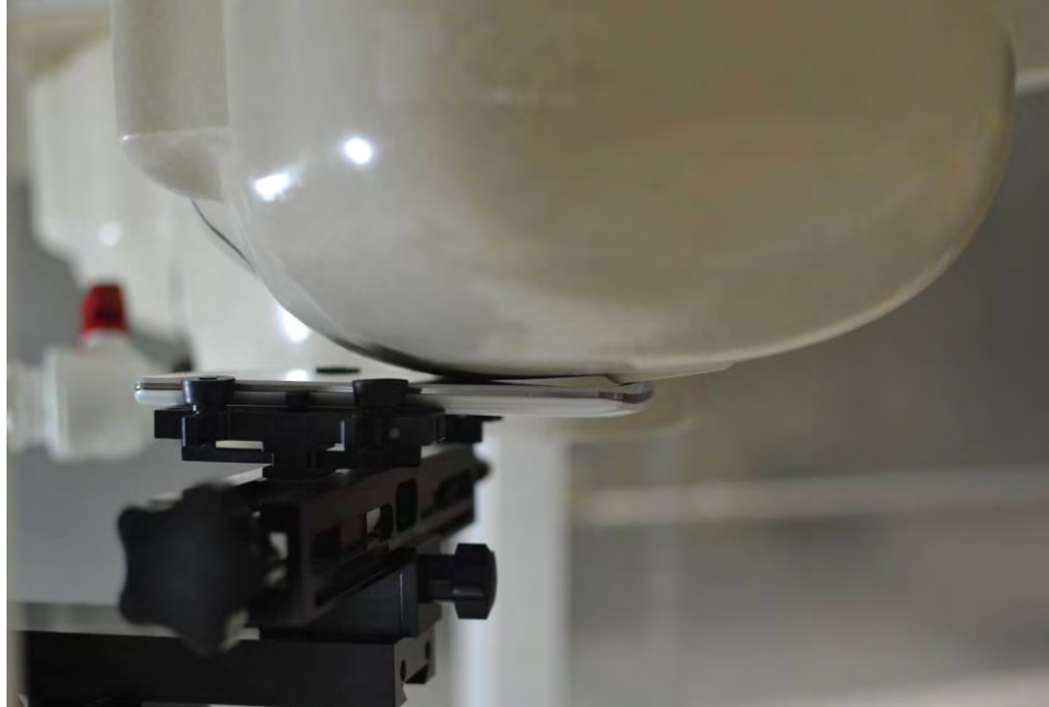
SAR Test Setup Photo 6 – Left Cheek, Standard Cover
