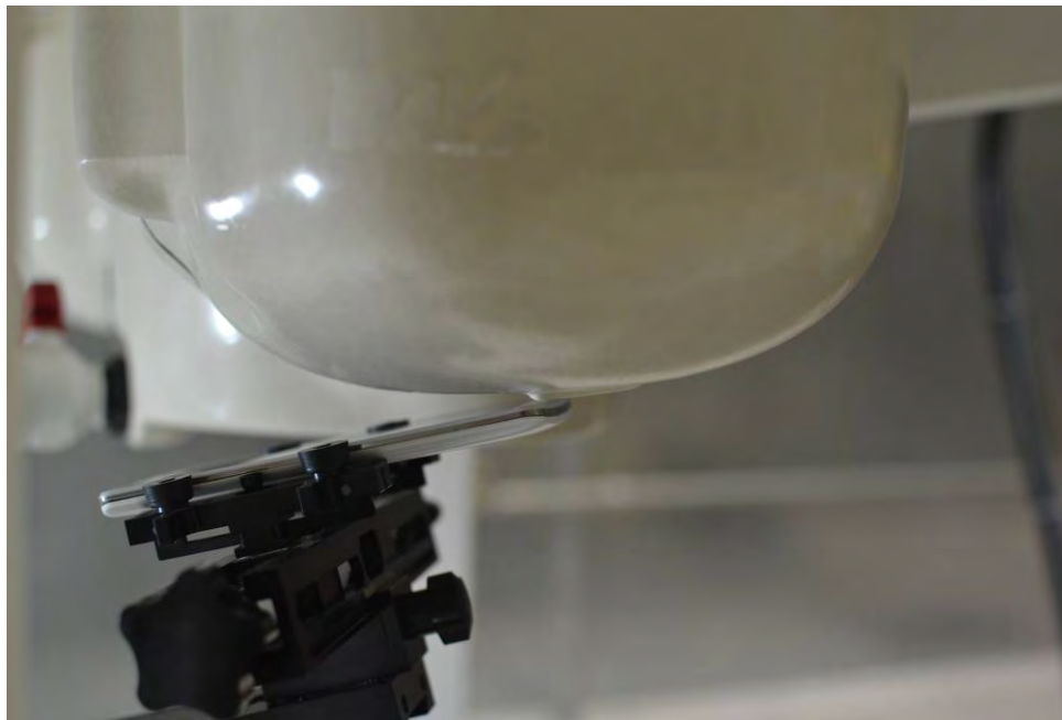
SAR Test Setup Photo 9 – Left Tilt, Standard Cover
