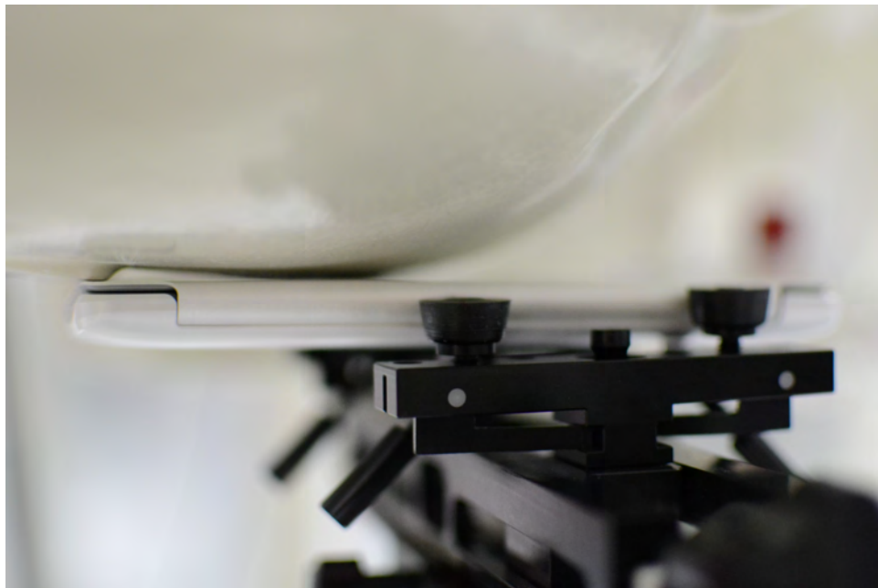
SAR Test Setup Photo 2: Right Cheek with Folio Accessory, Closed
