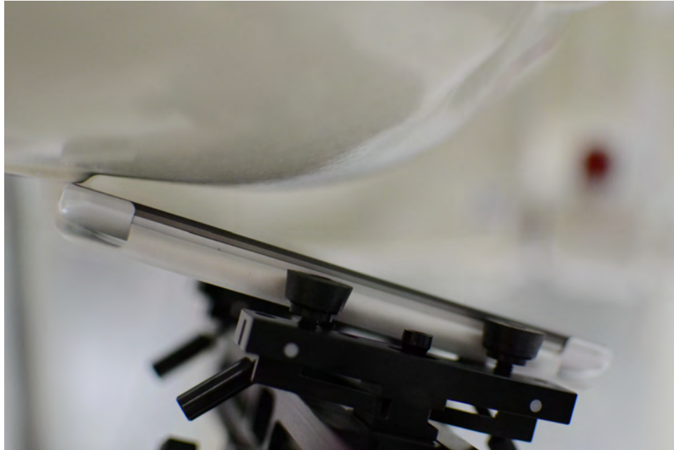
SAR Test Setup Photo 7: Right Tilt with Folio Accessory, Open
