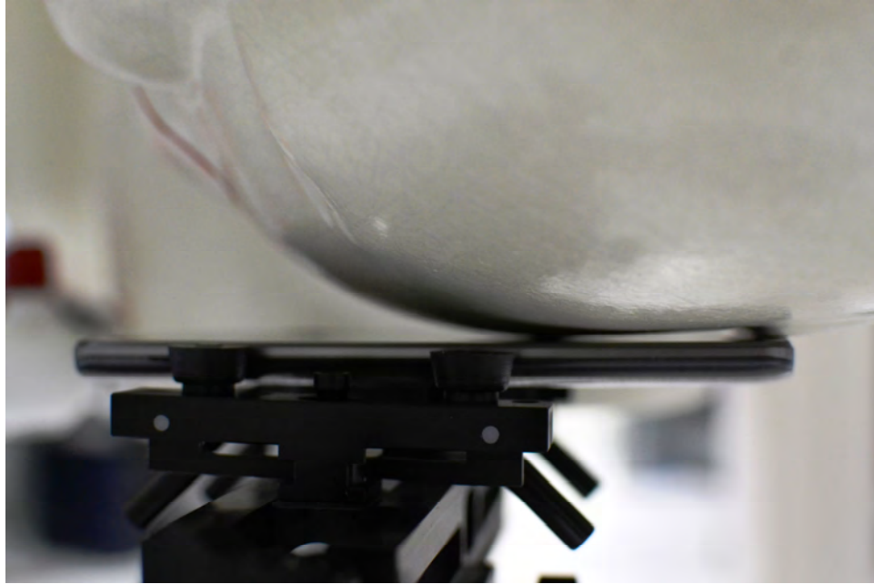
SAR Test Setup Photo 9: Left Cheek
