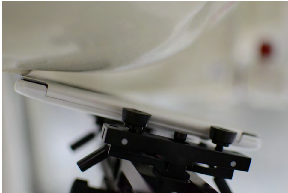
SAR Test Setup Photo 6: Right Tilt with Folio Accessory, Closed
