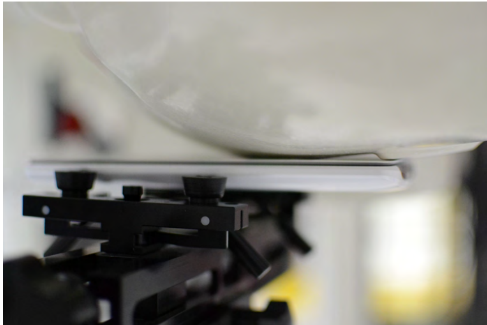
SAR Test Setup Photo 10: Left Cheek with Folio Accessory, Closed
