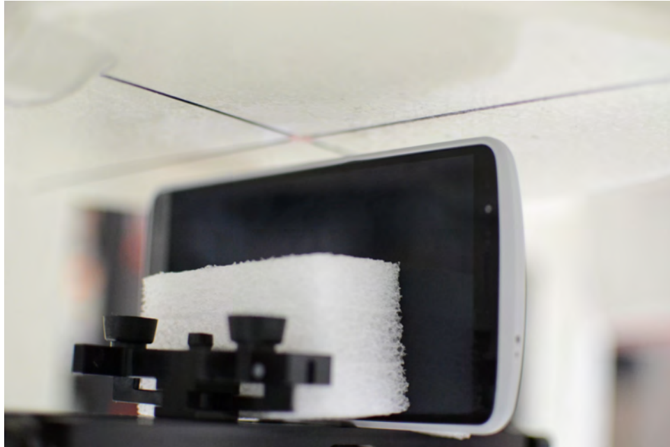
SAR Test Setup Photo 23: Left Edge with Wireless Charging Back Cover at 1.0 cm
