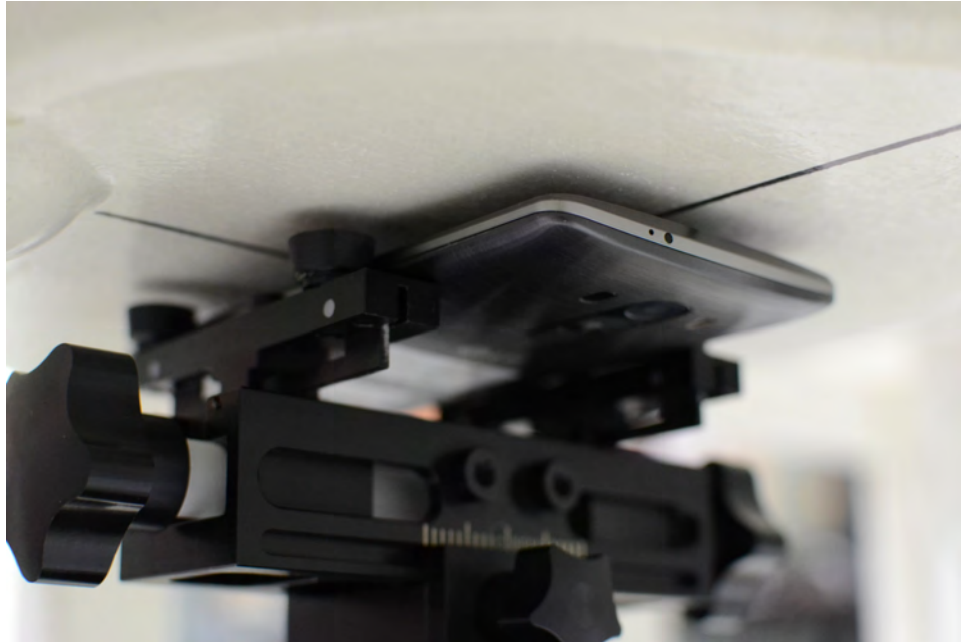
SAR Test Setup Photo 17: Front Side at 1.0 cm
