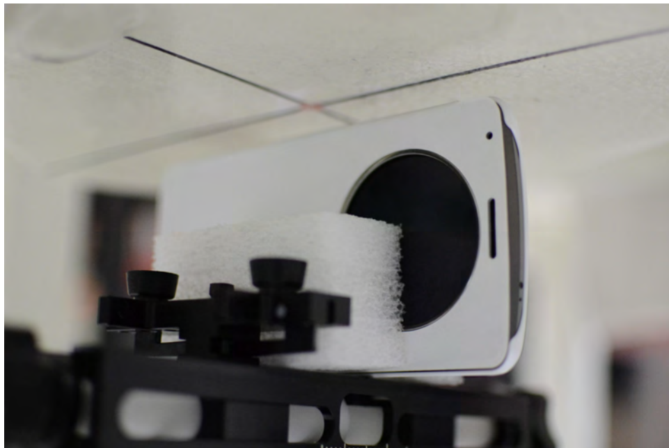
SAR Test Setup Photo 22: Left Edge with Folio Accessory, Closed at 1.0 cm
