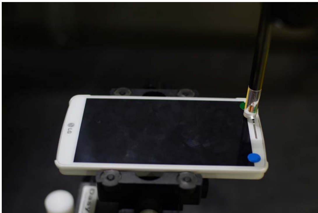
Figure 13-3 Test Setup for Wireless Device (Wireless Charging Cover Open)
