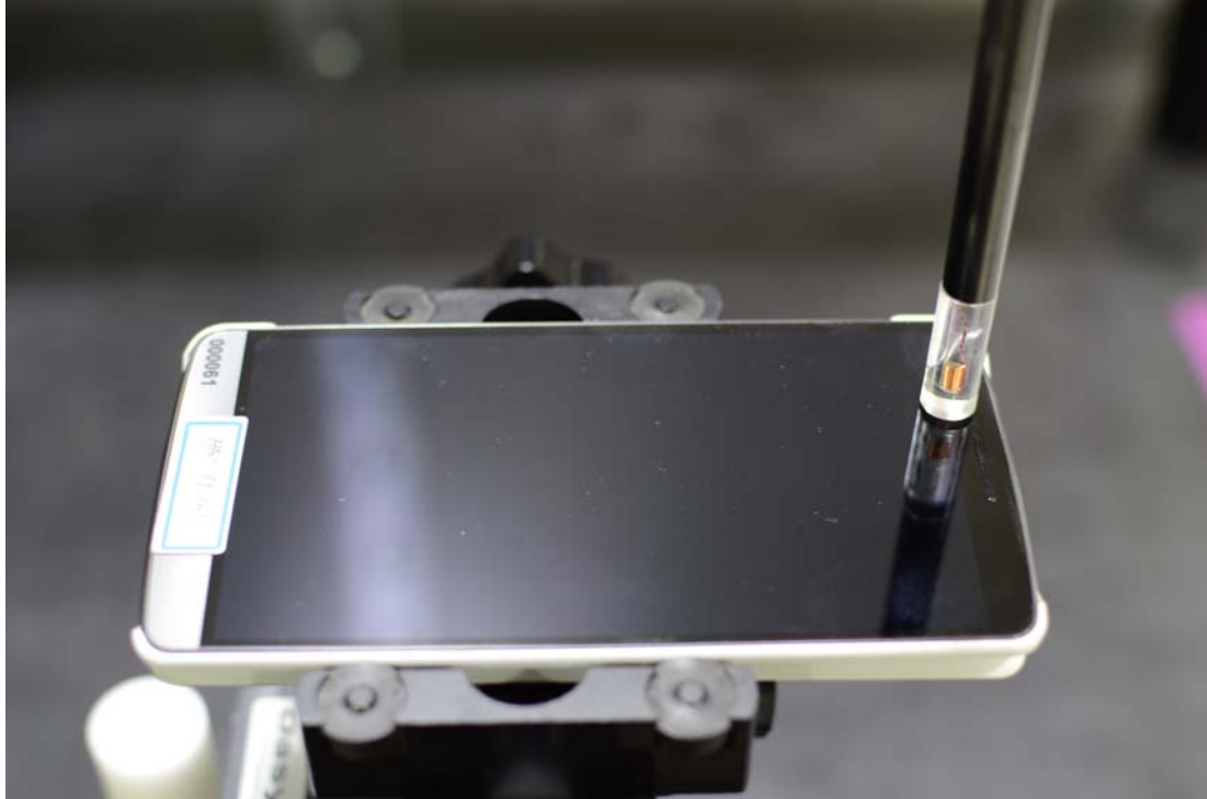
Figure 13-3 Test Setup for Wireless Device (Wireless Charging Case Open)
