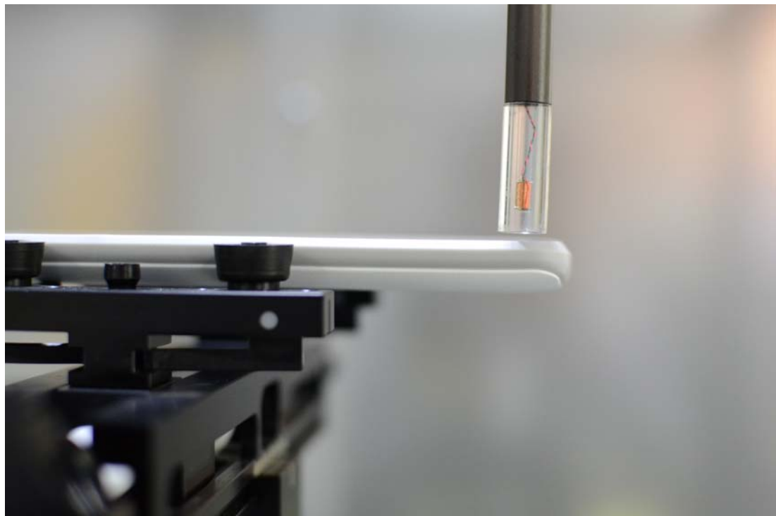
Figure 13-6 Test Setup for Wireless Device (Wireless Charging Cover)
