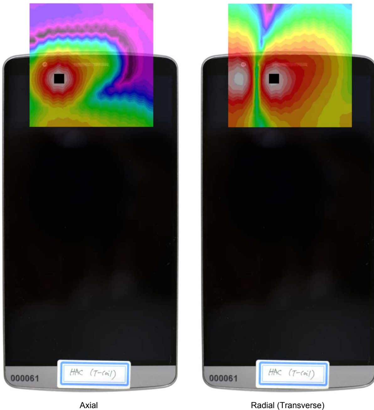
Figure 13-9 T-Coil Scan Overlay Magnetic Field Distributions
