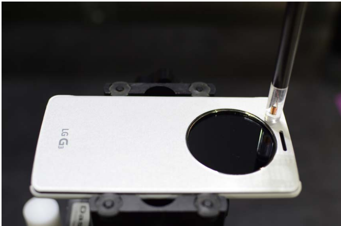
Figure 13-4 Test Setup for Wireless Device (Wireless Charging Case Closed)
