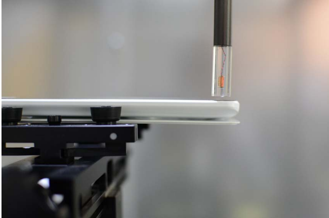
Figure 13-7 Test Setup for Wireless Device (Wireless Charging Case Open)
