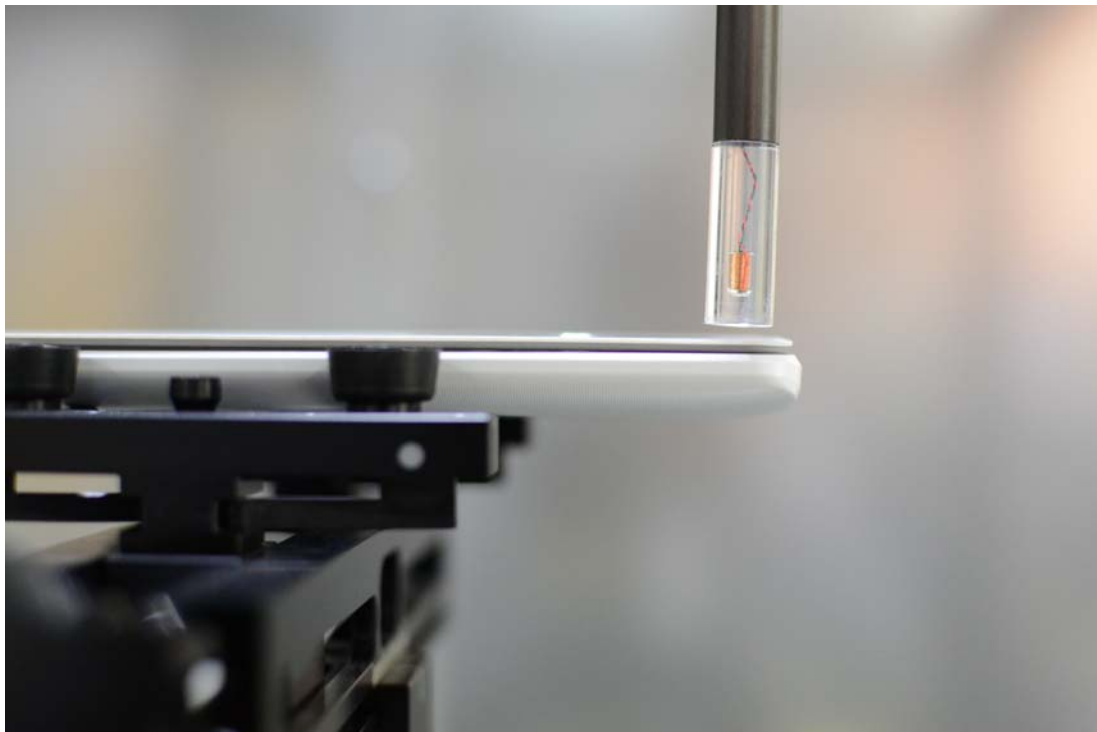
Figure 13-8 Test Setup for Wireless Device (Wireless Charging Case Closed)
