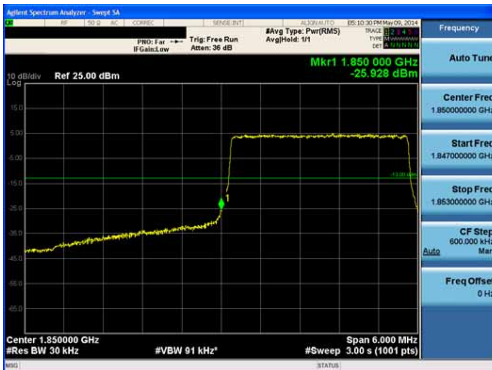
BAND 2. Lower Band Edge Plot (3M BW Ch.18615 QPSK RB 15) -2
