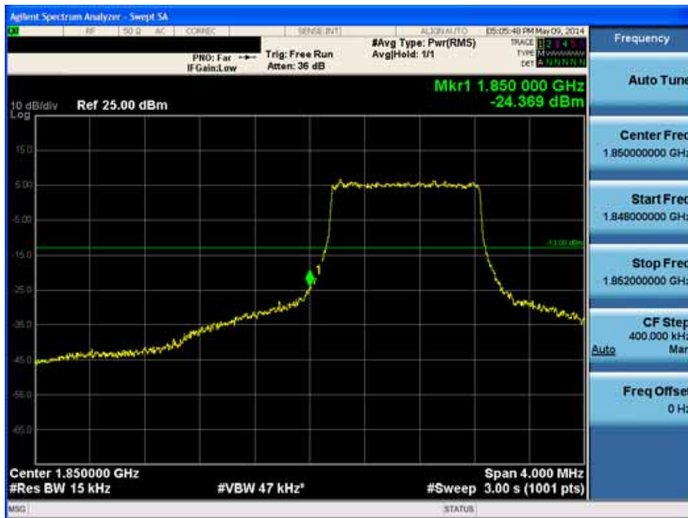
BAND 2. Lower Band Edge Plot (1.4M BW Ch.18607 QPSK RB 6) -2
