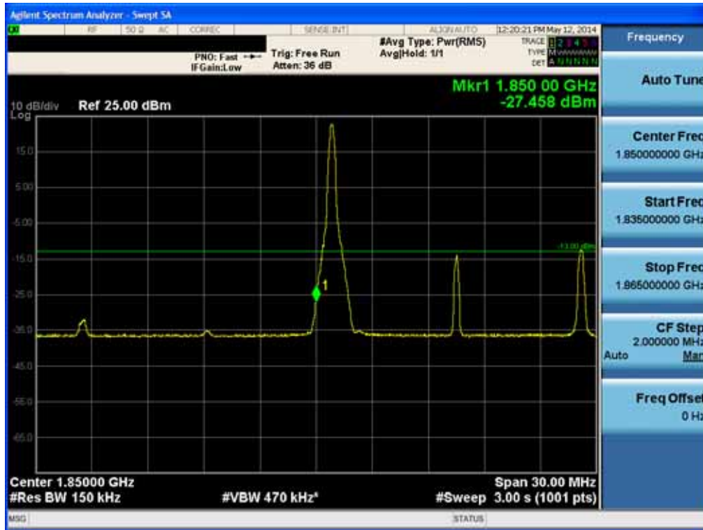
BAND 2. Lower Band Edge Plot (15M BW Ch.18675 QPSK RB 1, Offset 0) -1
