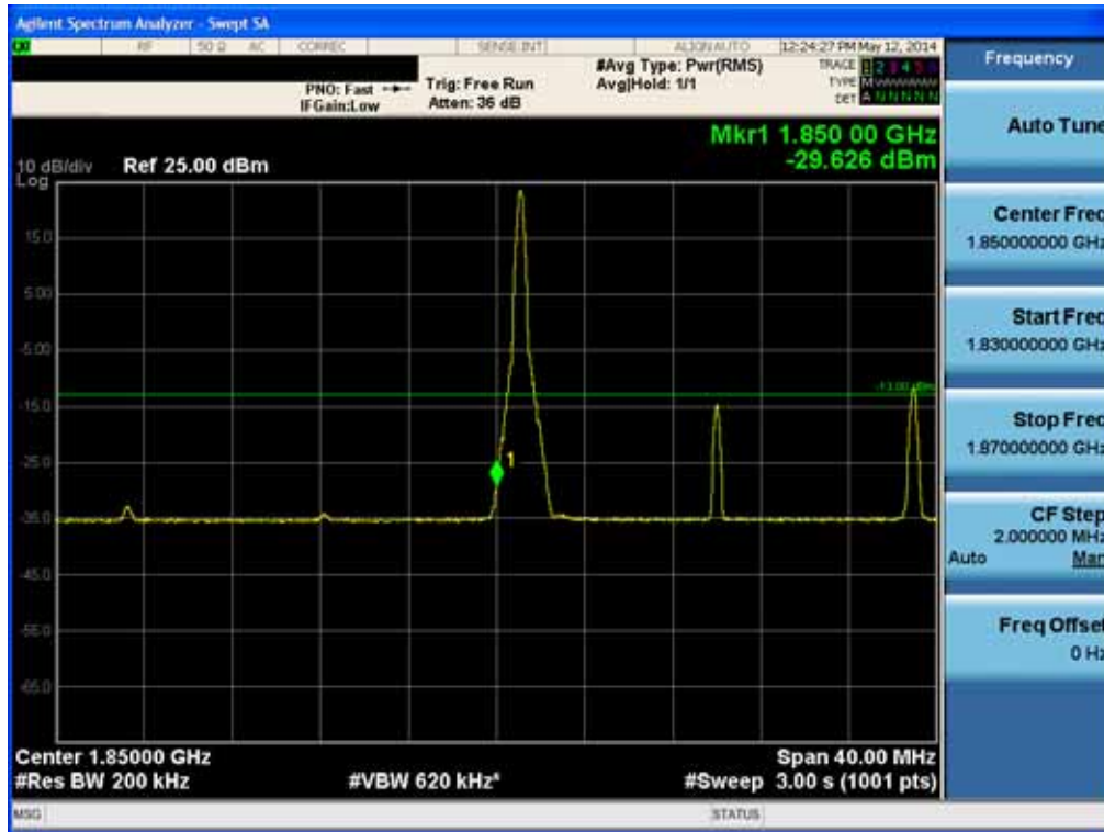
BAND 2. Lower Band Edge Plot (20M BW Ch.18700 QPSK RB 1, Offset 0) -1
