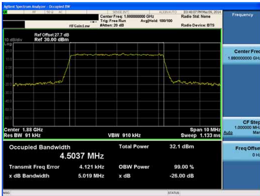
BAND 2. Occupied Bandwidth Plot (5M BW Ch.18900 16QAM RB 20_0)
