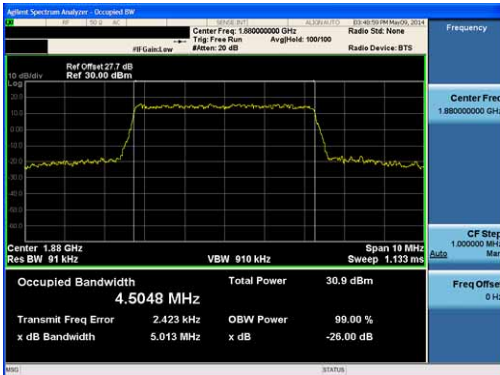
BAND 2. Occupied Bandwidth Plot (5M BW Ch.18900 QPSK RB 20_0)
