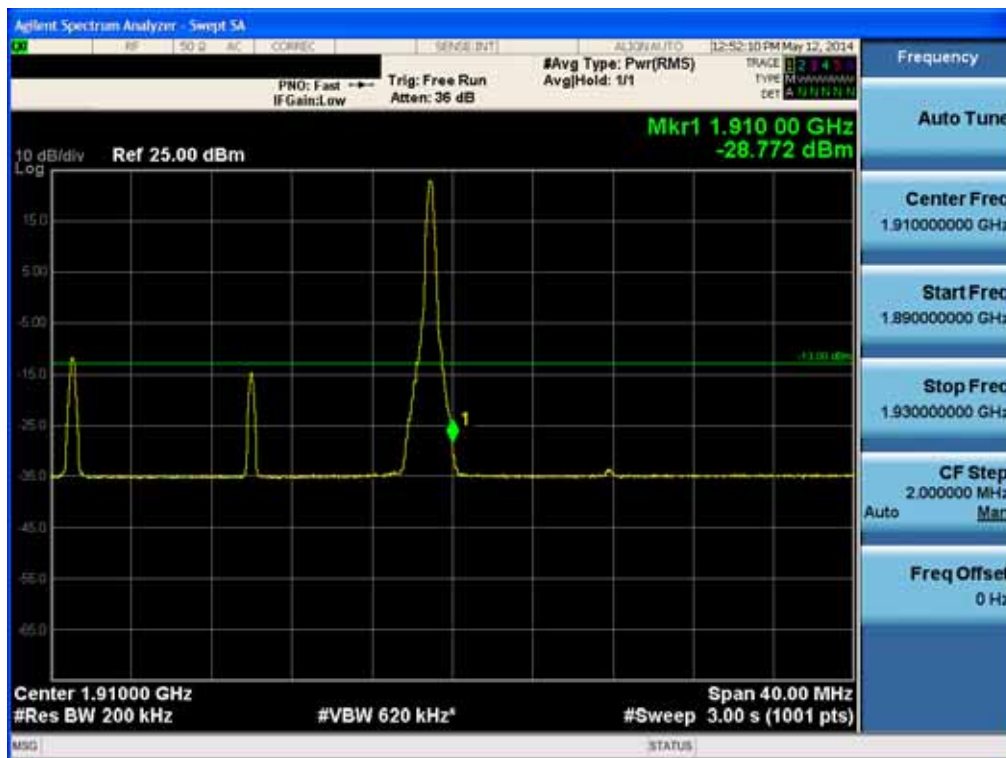
BAND 2. Upper Band Edge Plot (20M BW Ch.19100 QPSK RB 1, Offset 99) -1
