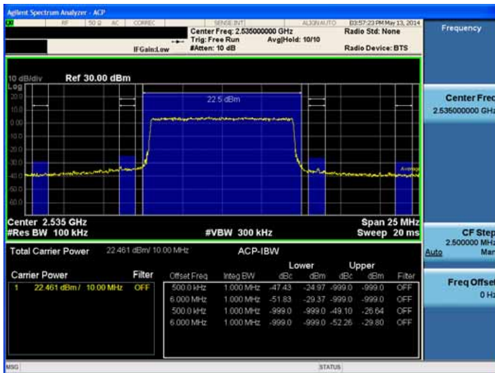
Mid Channel Edge Plot (10MHz Ch.21100 QPSK RB 50)
