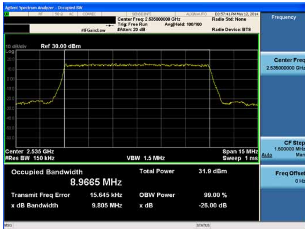
Occupied Bandwidth Plot (10MHz Ch.21100 QPSK RB 50)
