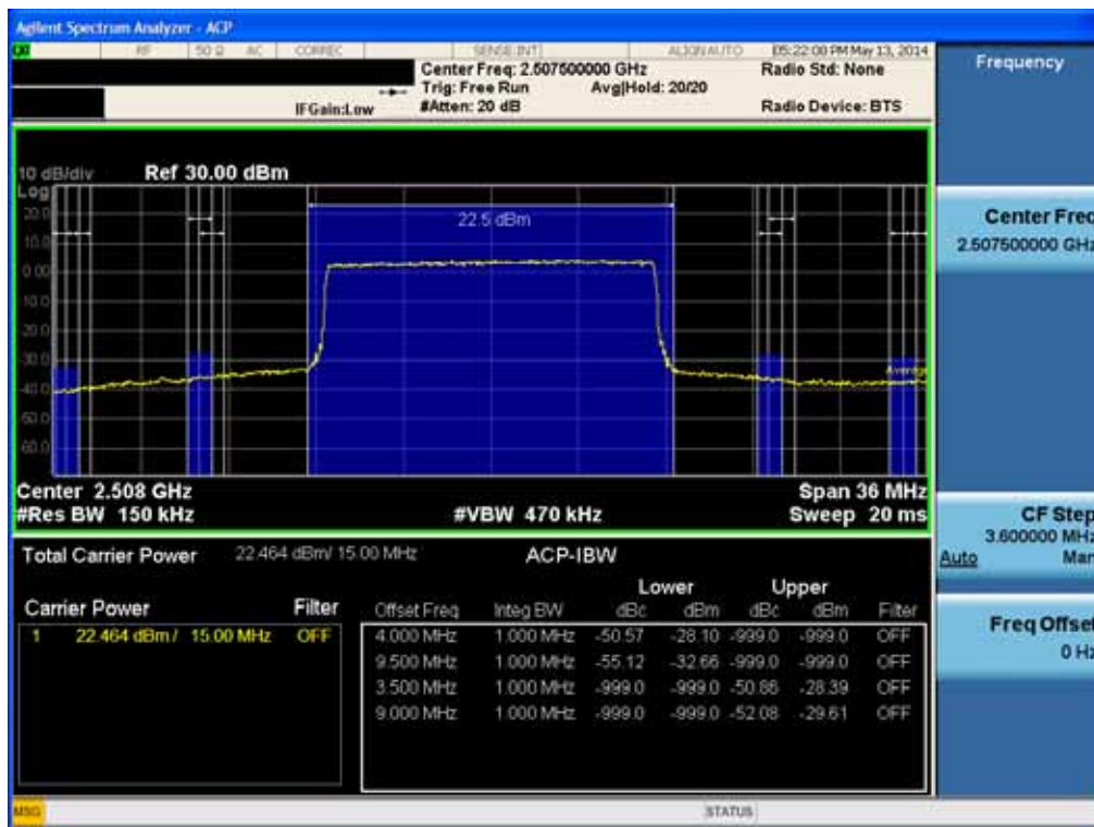
Low Channel Edge Plot (15MHz Ch.20825 QPSK RB 75)
