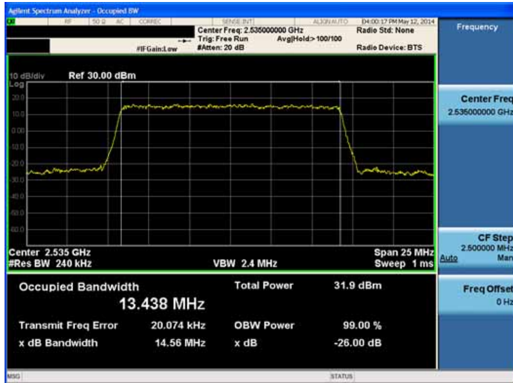
Occupied Bandwidth Plot (15MHz Ch.21100 QPSK RB 75)
