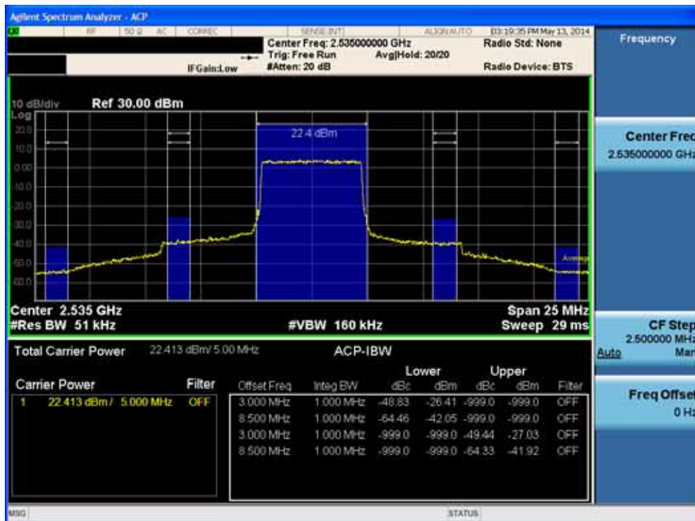
Mid Channel Edge Plot (5MHz Ch.21100 QPSK RB 25)
