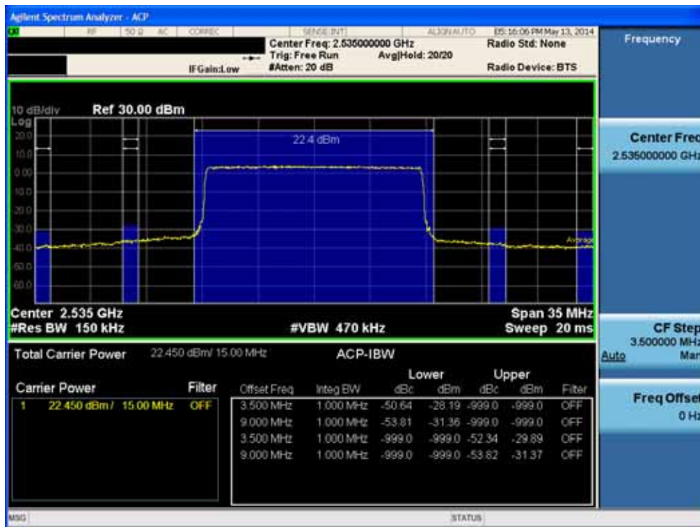
Mid Channel Edge Plot (15MHz Ch.21100 QPSK RB 75)
