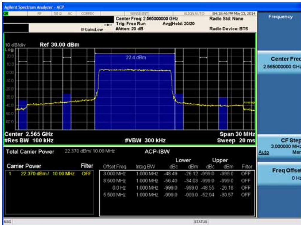
High Channel Edge Plot (10MHz Ch.21400 QPSK RB 50)
