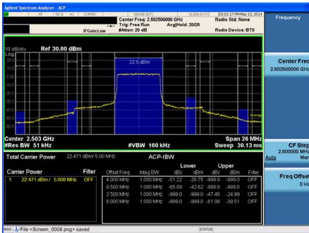
Low Channel Edge Plot (5MHz Ch.20775 QPSK RB 25)
