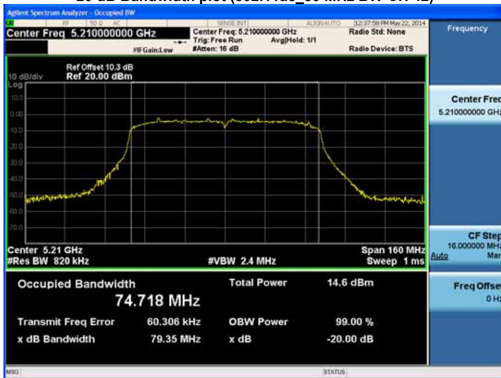
20 dB Bandwidth plot (802.11ac_80 MHz BW-CH 42)
