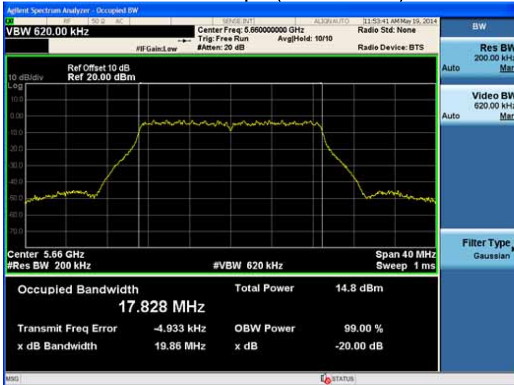
20 dB Bandwidth plot (802.11ac-CH 132)
