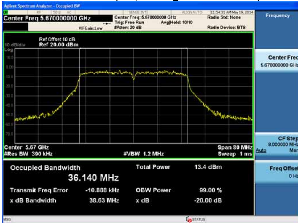
20 dB Bandwidth plot (802.11ac_40 MHz BW-CH 134)
