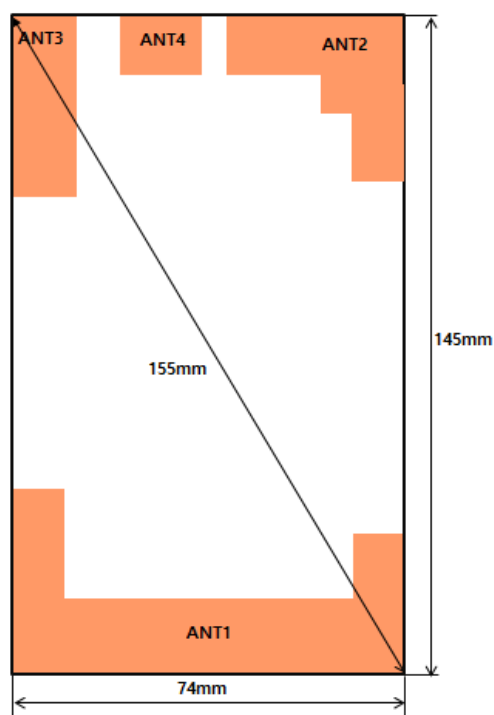
Rear View
