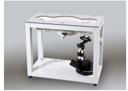
Figure 3.6 SAM Twin Phantom
