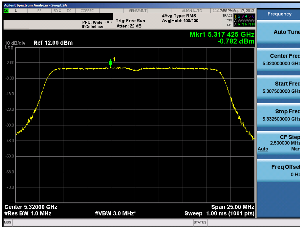
Plot 6-53. Peak Power Spectral Density Plot (20MHz BW 802.11n (UNII Band 2) – Ch. 64)
