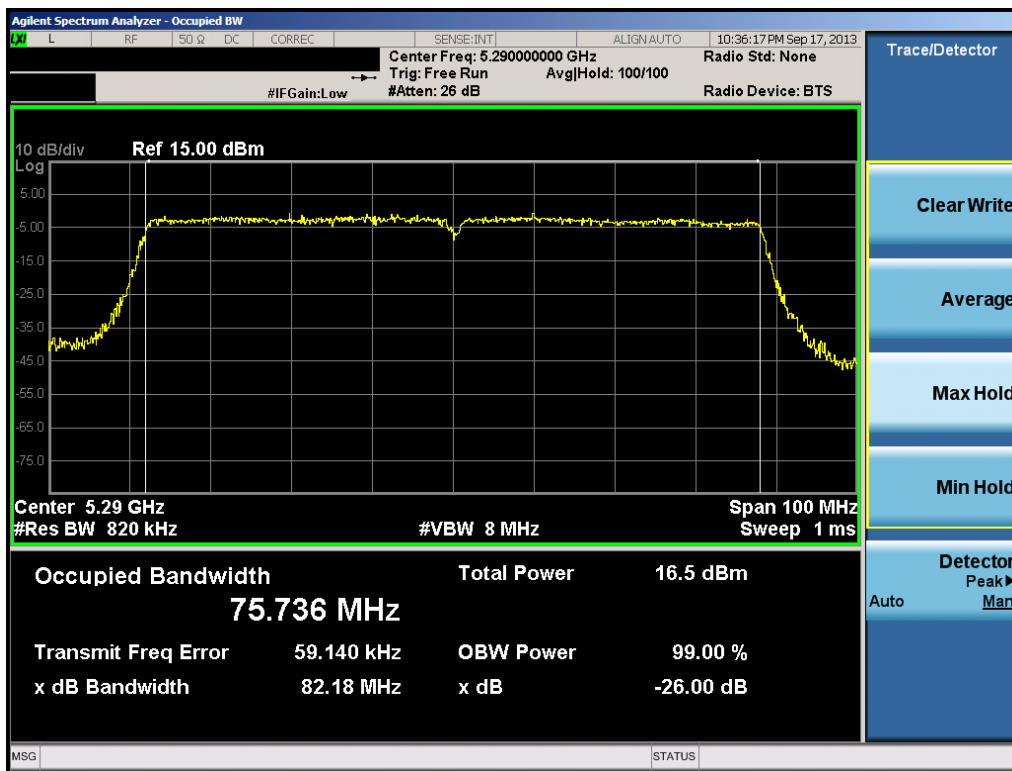
Plot 6-18. 26dB Bandwidth Plot (80MHz BW 802.11ac (UNII Band 2) – Ch. 58)
