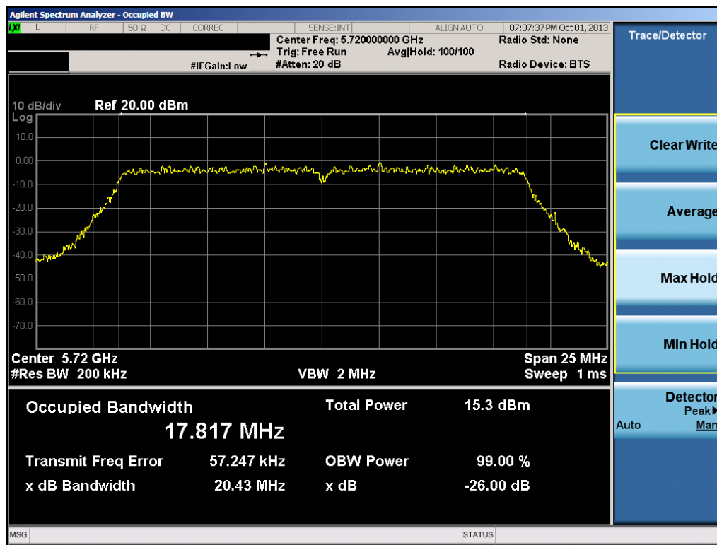
Plot 6-24. 26dB Bandwidth Plot (20MHz BW 802.11n (UNII Band 3) – Ch. 144)
