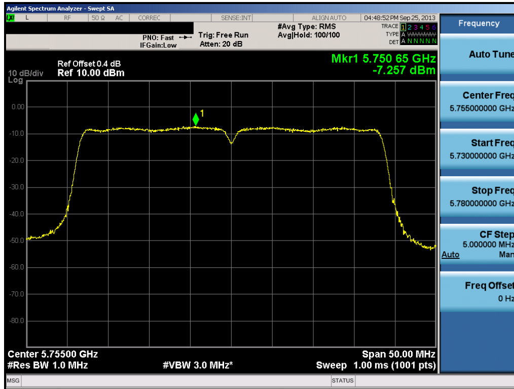
Plot 6-73. Peak Power Spectral Density Plot (40MHz BW 802.11n (UNII Band 4) – Ch. 151)
