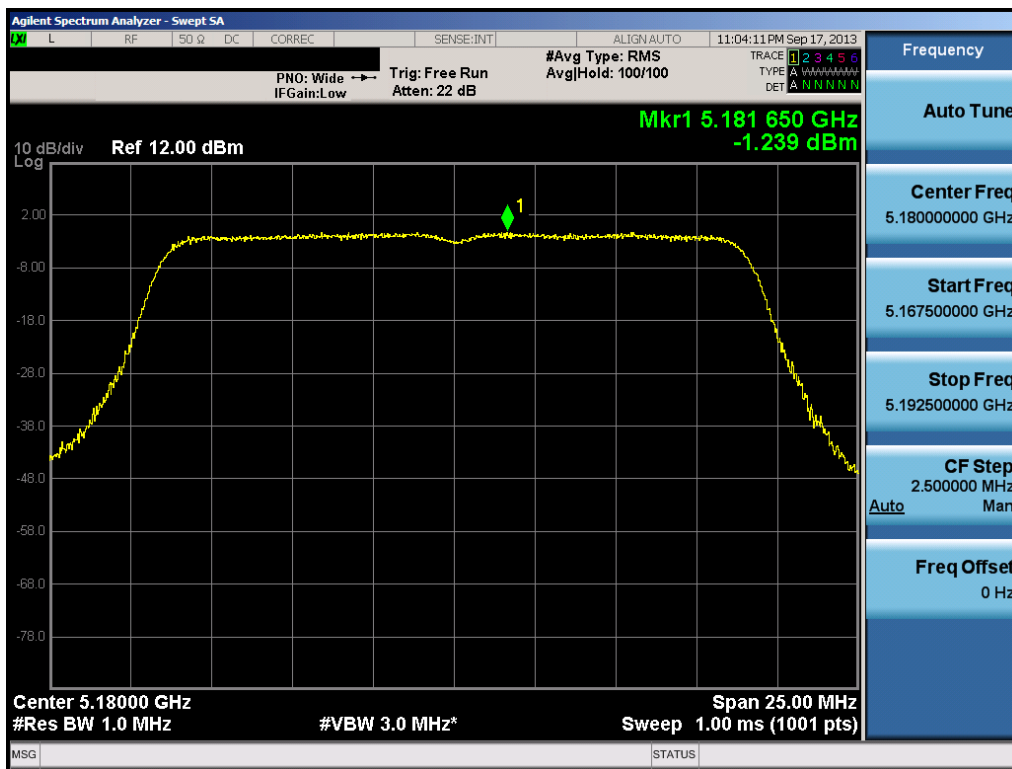
Plot 6-42. Peak Power Spectral Density Plot (20MHz BW 802.11n (UNII Band 1) – Ch. 36)
