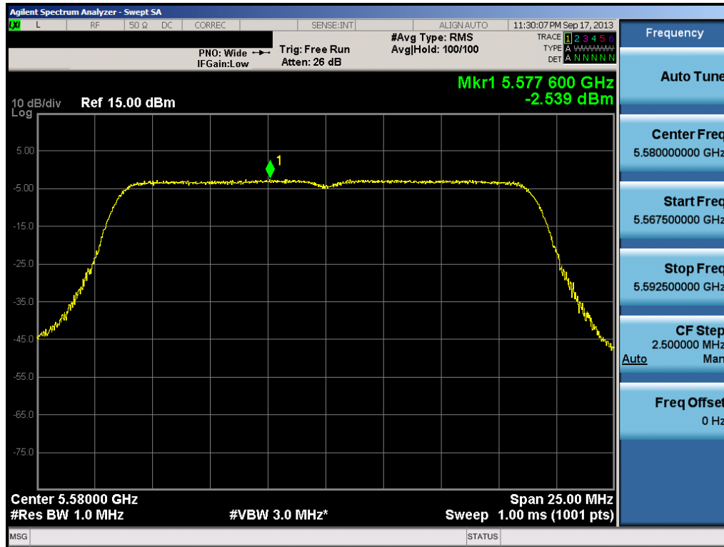
Plot 6-61. Peak Power Spectral Density Plot (20MHz BW 802.11n (UNII Band 3) – Ch. 116)
