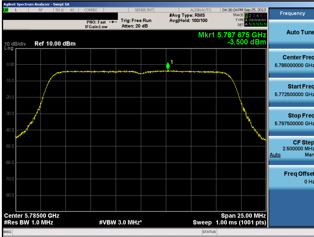
Plot 6-71. Peak Power Spectral Density Plot (20MHz BW 802.11n (UNII Band 4) – Ch. 157)
