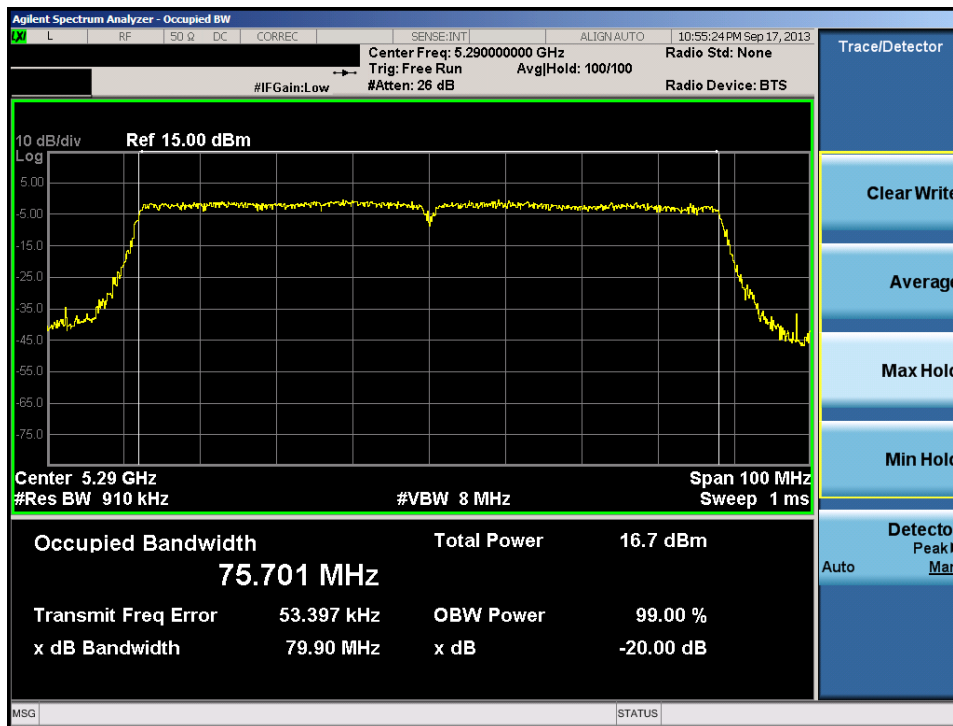
Plot 6-38. 20dB Bandwidth Plot (80MHz BW 802.11n (UNII Band 2) – Ch. 58)
