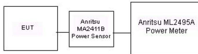
Power Measurement Setup for Signal < 50 MHz Bandwidth
