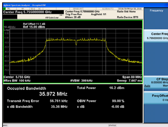
802.11n_HT40 UNII 3 BAND 6dB Bandwidth(CH.151)
