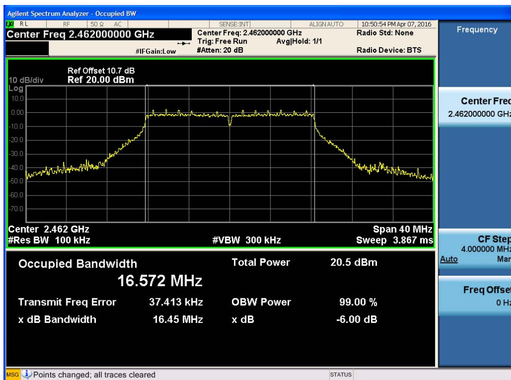
6dB Bandwidth plot (802.11g-CH 11)
