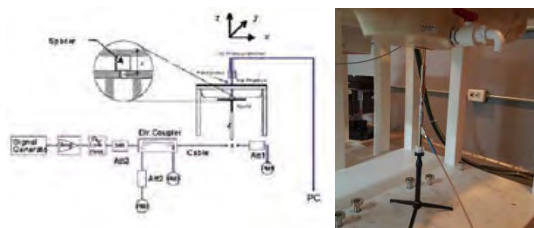
Figure 11.1 Dipole Verification Test Setup Diagram & Photo
