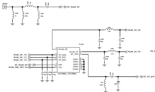
ANTENNA SWITCH MODULE LOGIC
