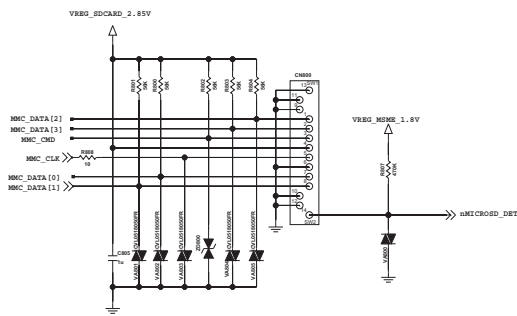
MICRO-SD
