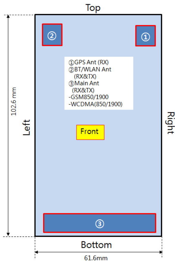
Figure 13.1 Identification of Sides for SAR Testing
