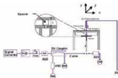
Figure 9.1 Dipole Verification Test Setup
