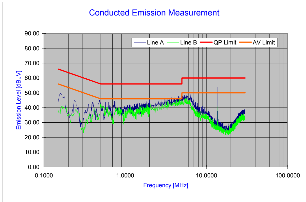
Plot 8-1. Line-Conducted Test Plot
