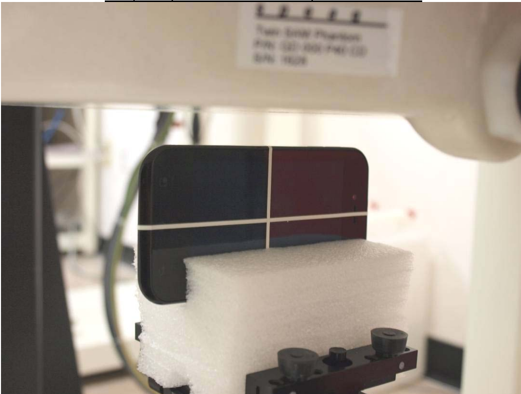
Body-hotspot: Left w/ 10 mm separation distance
