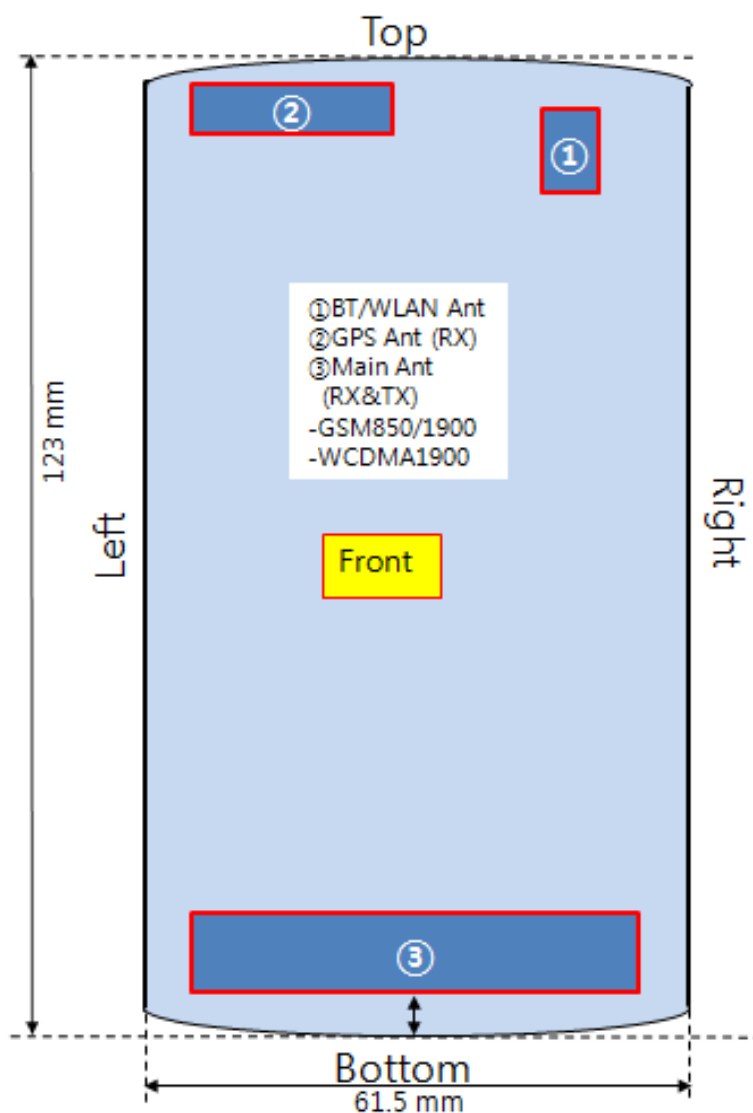
Figure 13.1 Identification of Sides for SAR Testing
