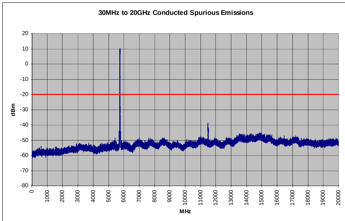
Plot 6-53. Conducted Spurious Plot (802.11a – Ch. 149)
