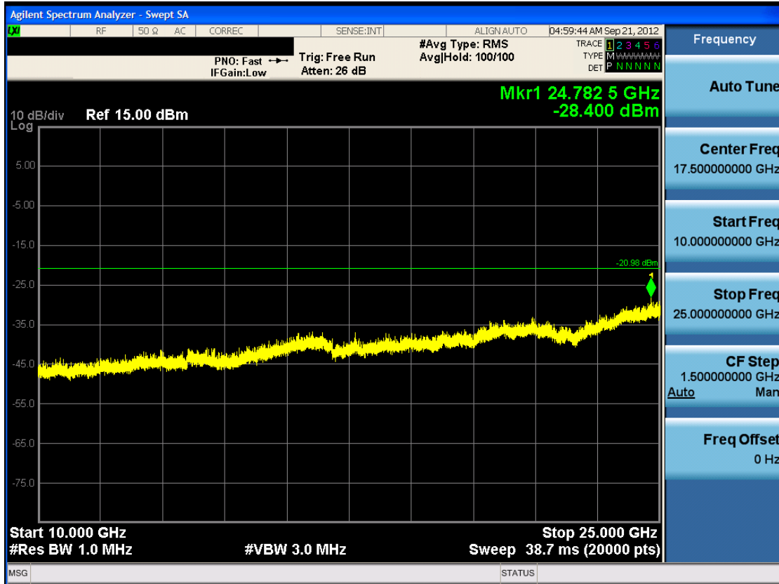
Plot 6-52. Conducted Spurious Plot (802.11b – Ch. 11)
