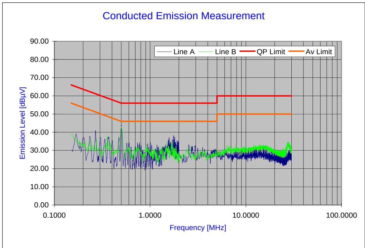
Plot 6-60. Line Conducted Plot with 802.11a
