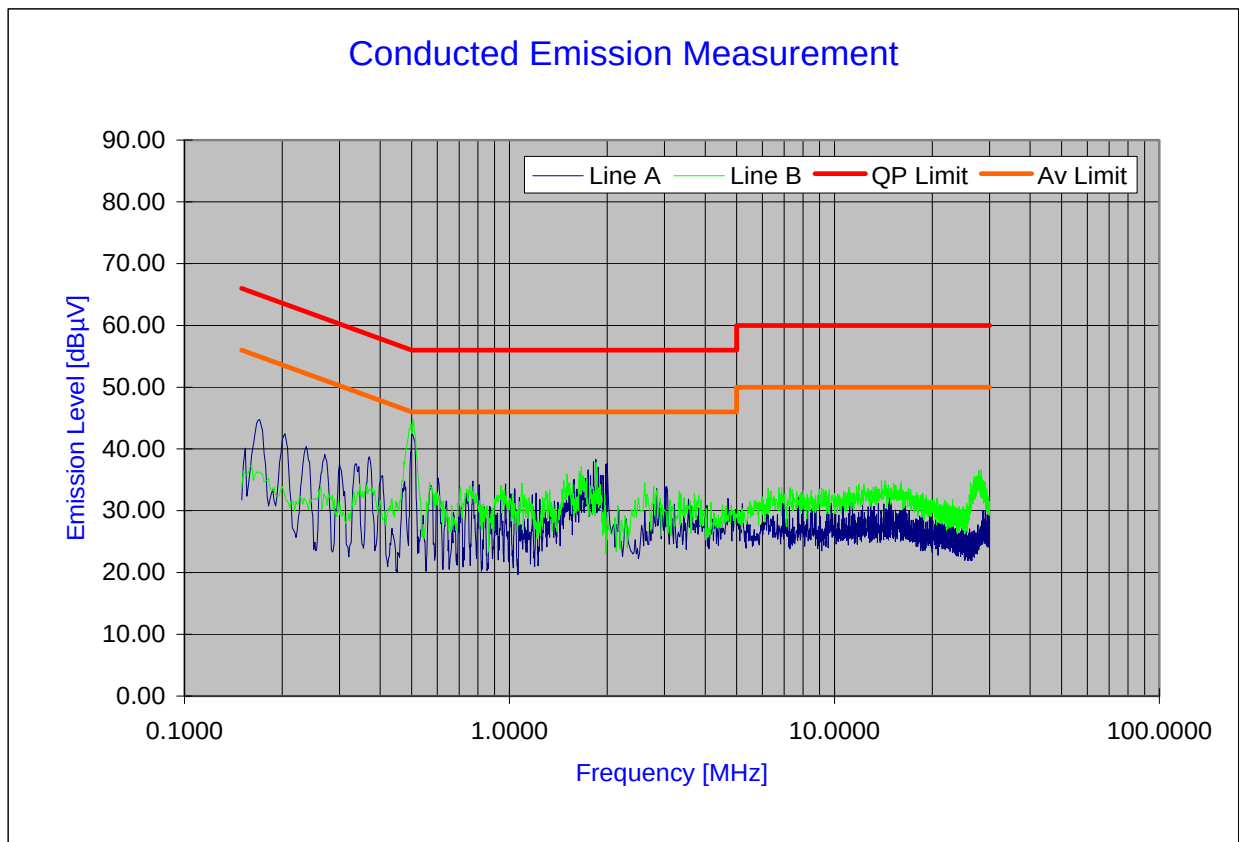
Plot 6-59. Line Conducted Plot with 802.11b
