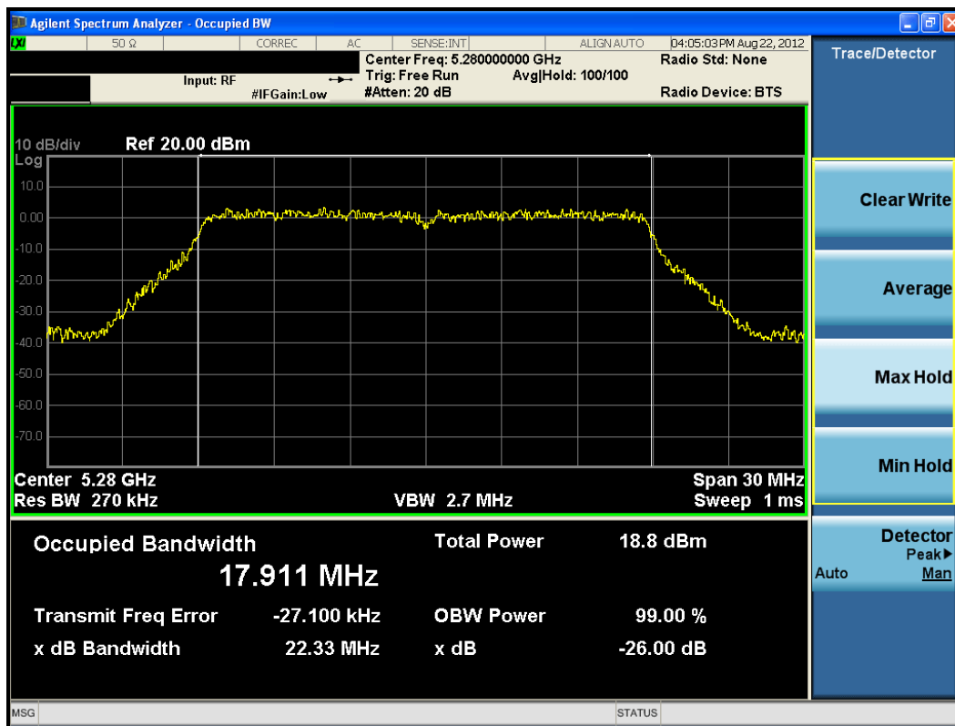
Plot 6-13. 26dB Bandwidth Plot (20MHz BW 802.11n (UNII Band 2) – Ch. 56)
