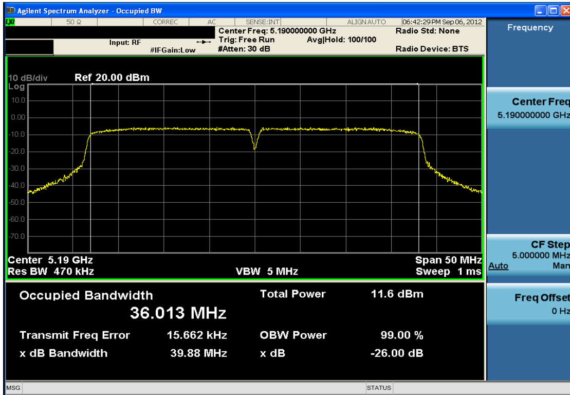
Plot 6-7. 26dB Bandwidth Plot (40MHz BW 802.11n (UNII Band 1) – Ch. 38)
