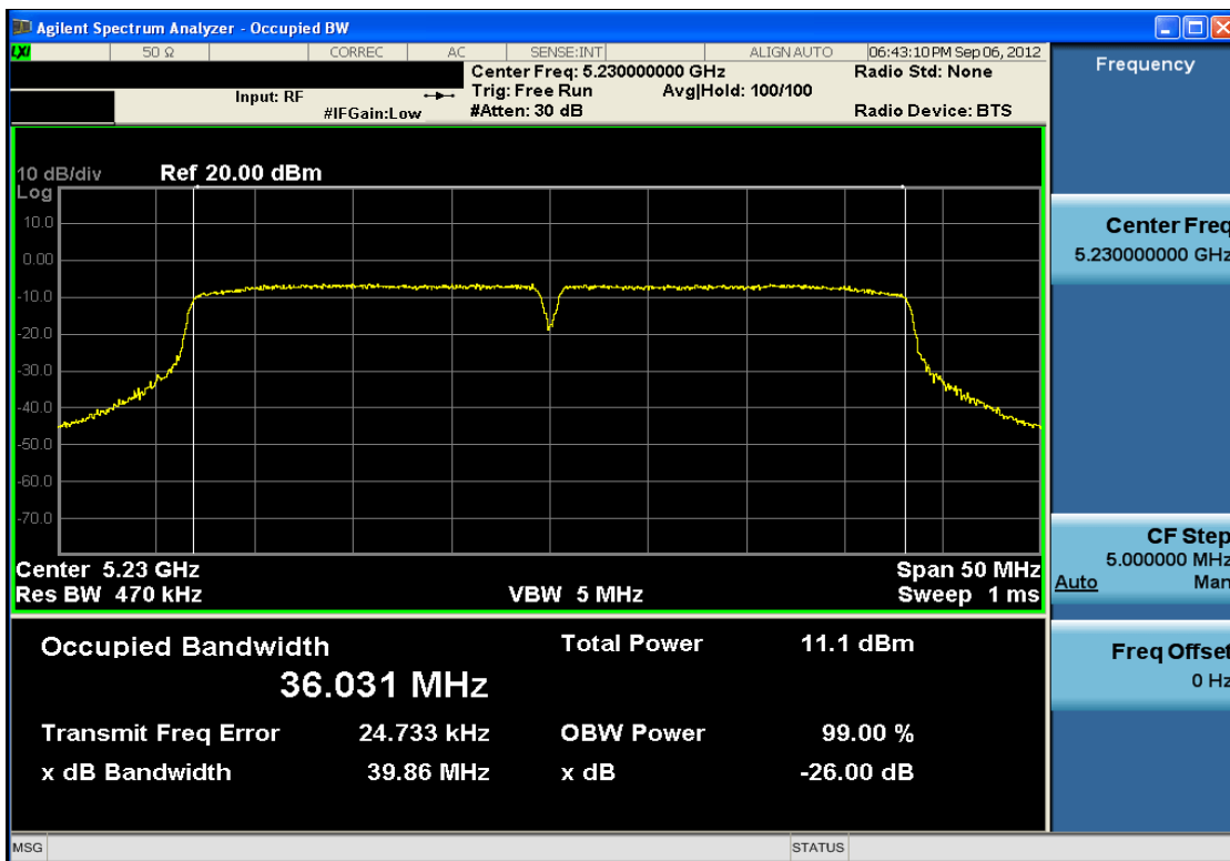
Plot 6-8. 26dB Bandwidth Plot (40MHz BW 802.11n (UNII Band 1) – Ch. 46)
