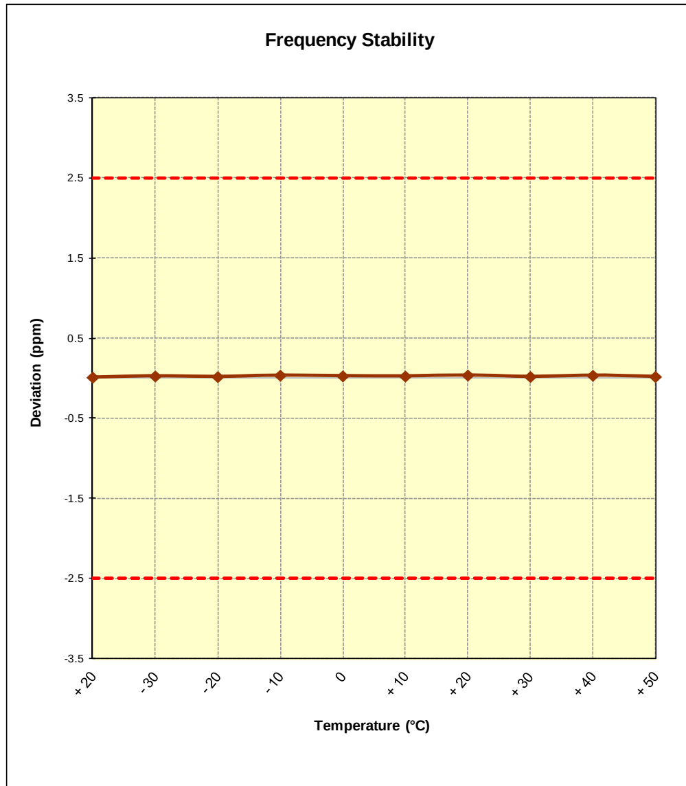
Figure 6-2. Frequency Stability Graph (Cellular WCDMA Mode – Ch. 4183)
