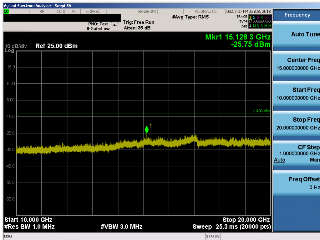
Plot 7-33. Conducted Spurious Plot (PCS WCDMA Mode – Ch. 9262)
