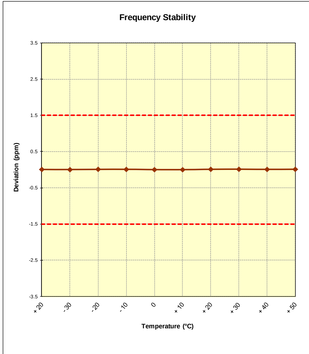
Figure 6-3. Frequency Stability Graph (PCS GSM Mode – Ch. 661)
