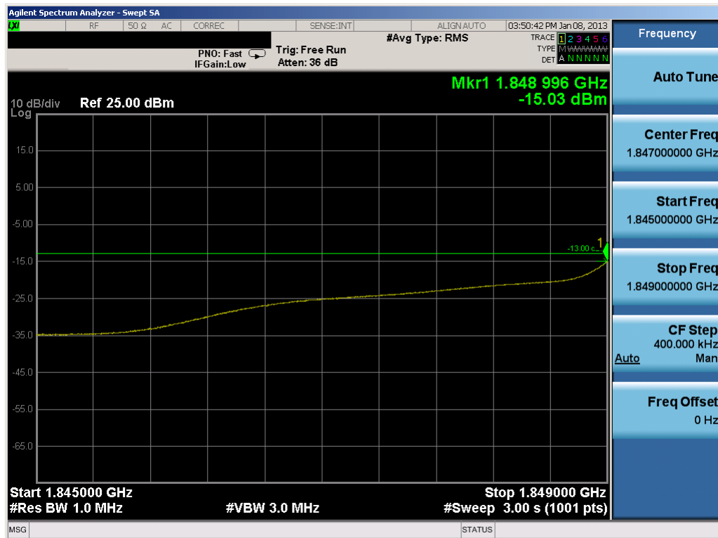
Plot 7-35. 4MHz Span Plot (PCS WCDMA Mode – Ch. 9262)
