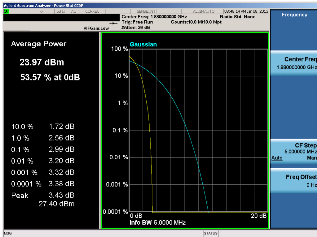
Plot 7-39. Peak-Average Ratio Plot (PCS WCDMA Mode – Ch. 9400)
