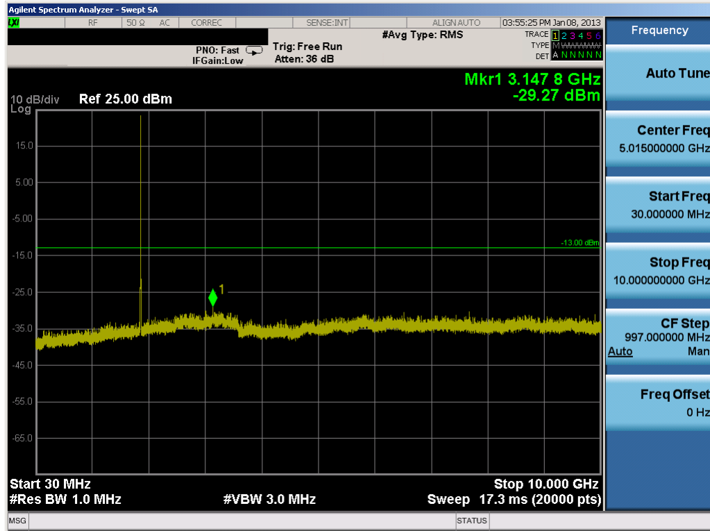
Plot 7-36. Conducted Spurious Plot (PCS WCDMA Mode – Ch. 9400)
