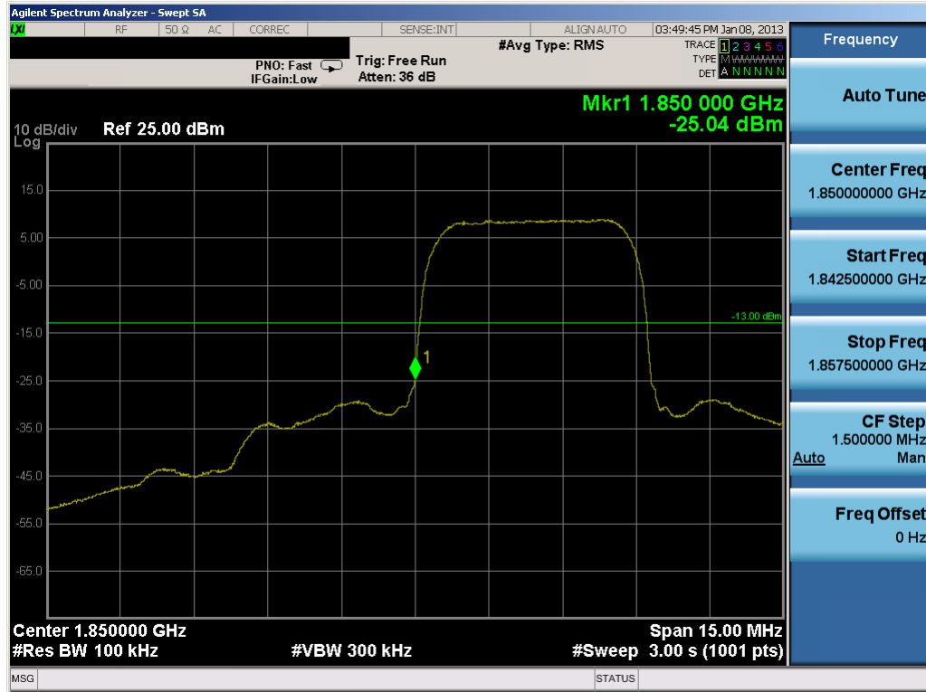
Plot 7-34. Band Edge Plot (PCS WCDMA Mode – Ch. 9262)
