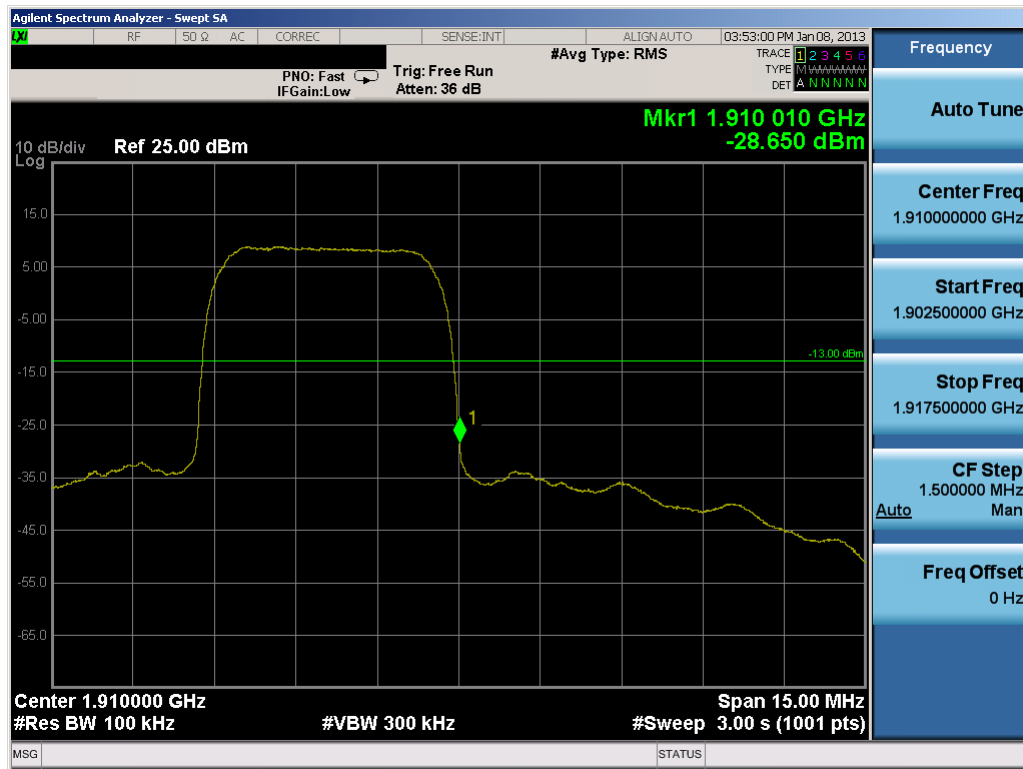
Plot 7-42. Band Edge Plot (PCS WCDMA Mode – Ch. 9538)
