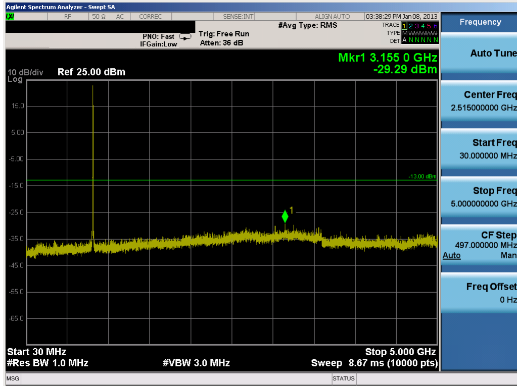
Plot 7-26. Conducted Spurious Plot (Cellular WCDMA Mode – Ch. 4183)
