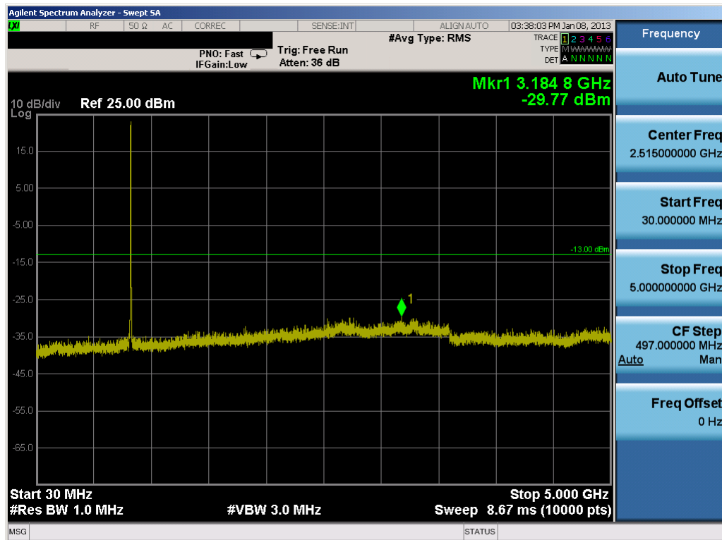
Plot 7-29. Conducted Spurious Plot (Cellular WCDMA Mode – Ch. 4233)
