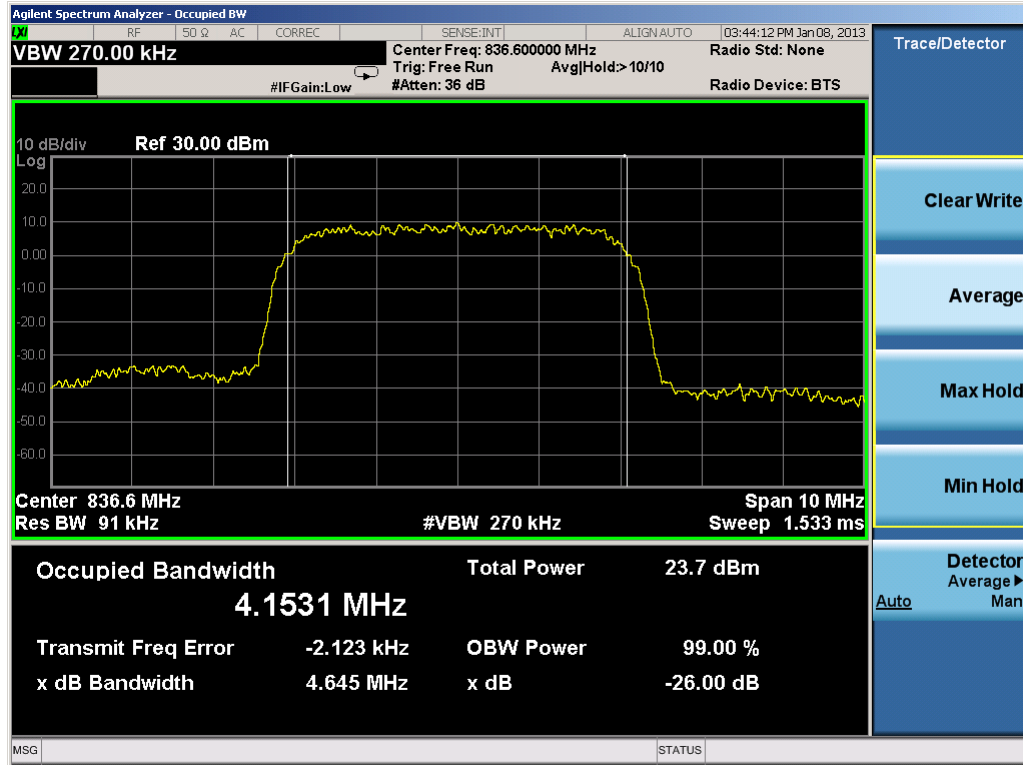
Plot 7-28. Occupied Bandwidth Plot (Cellular WCDMA Mode – Ch. 4183)
