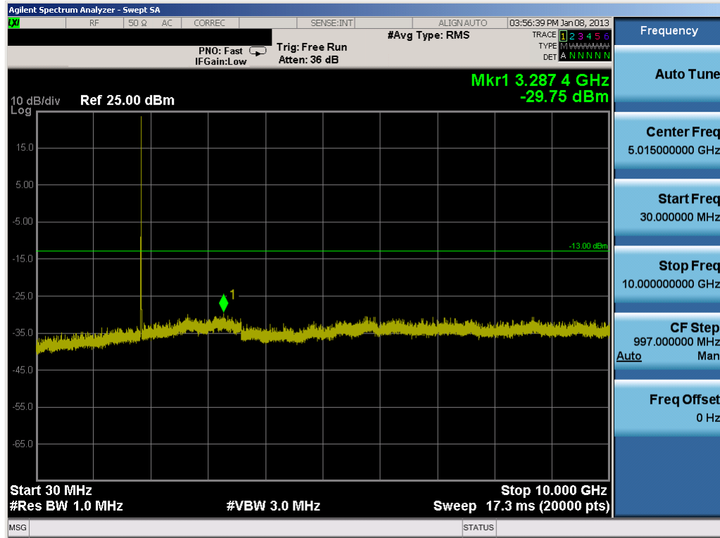
Plot 7-32. Conducted Spurious Plot (PCS WCDMA Mode – Ch. 9262)
