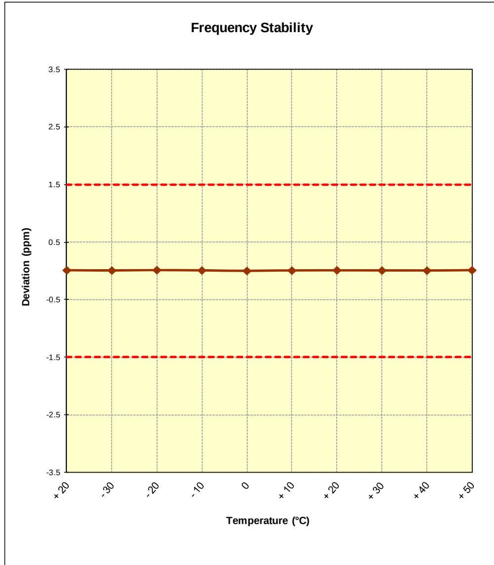
Figure 6-4. Frequency Stability Graph (PCS WCDMA Mode – Ch. 9400)
