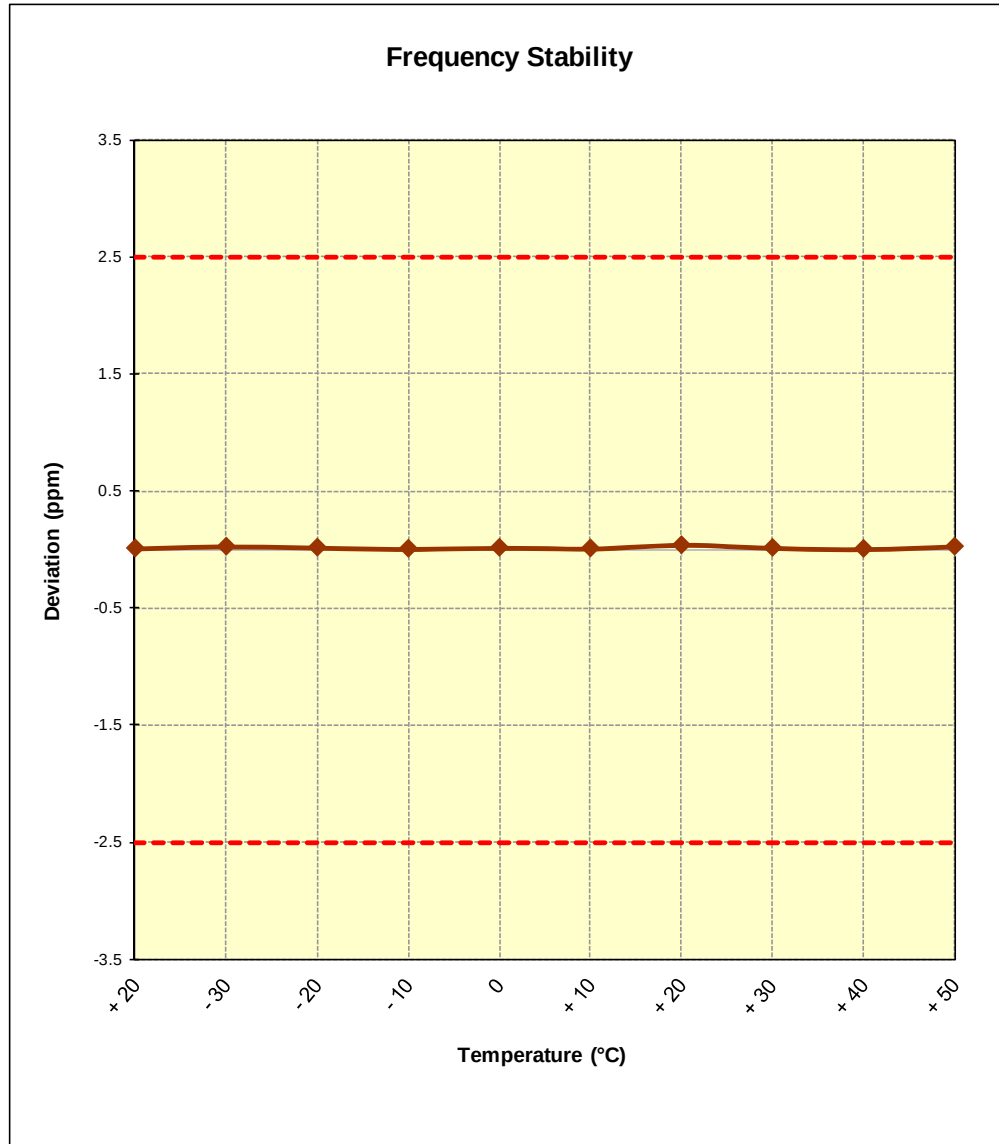
Figure 6-1. Frequency Stability Graph (Cellular GSM Mode – Ch. 190)
