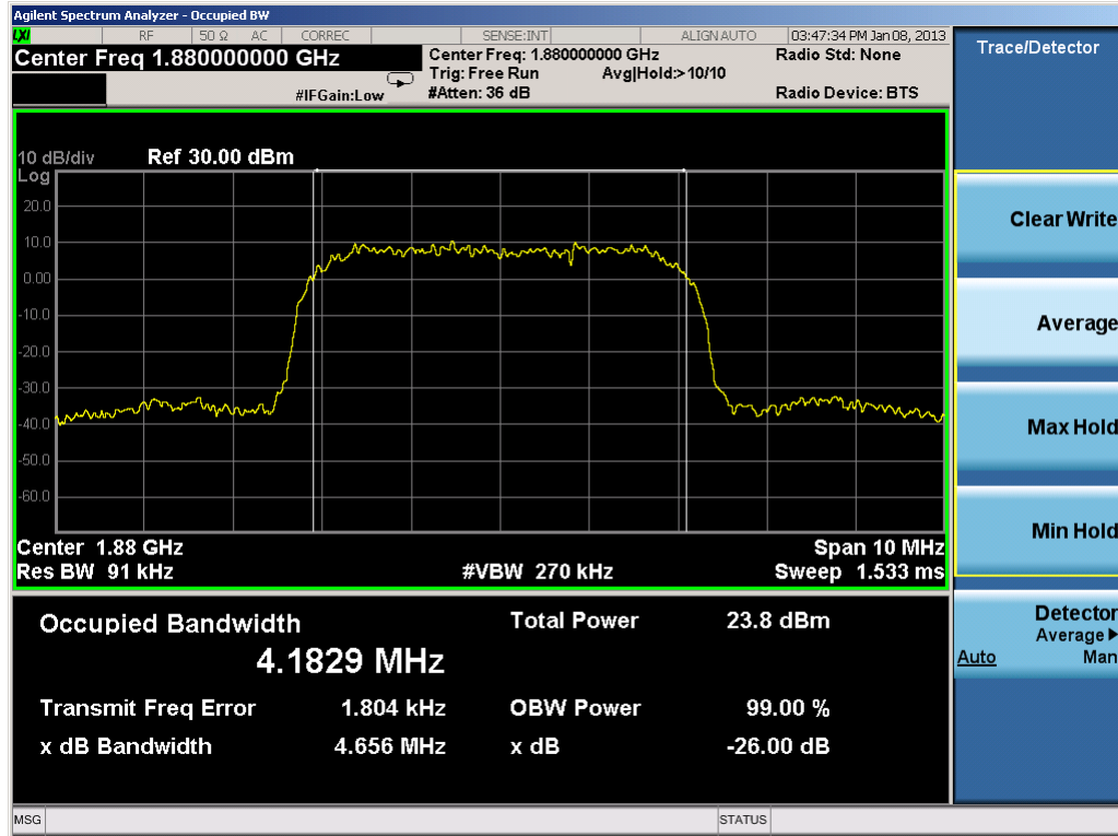
Plot 7-38. Occupied Bandwidth Plot (PCS WCDMA Mode – Ch. 9400)
