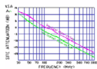
Figure 3-4. Normalized Site Attenuation Curves (H&V)
