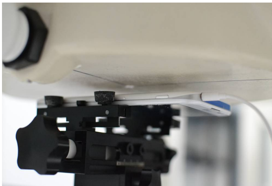
SAR Test Setup Photo 10 – Back side with Headset Cable at 1.0 cm
