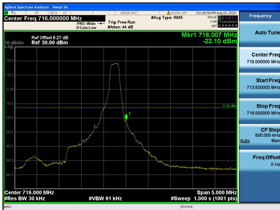
LTE Band 12 / 1.4 MHz / QPSK - RB Size/Offset (1/5)
