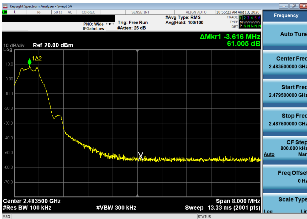
Plot 7-5. Band Edge Plot (Bluetooth (LE), 1Mbps – Ch. 39)
