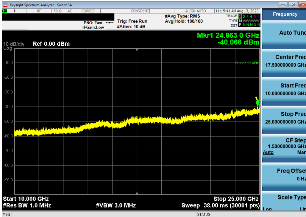
Plot 7-11. Conducted Spurious Plot (Bluetooth (LE), 1Mbps – Ch. 39)
