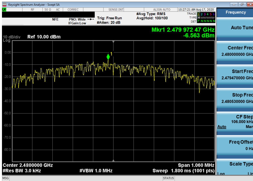
Plot 7-33. Power Spectral Density Plot (Bluetooth (LE), 1Mbps – Ch. 39)
