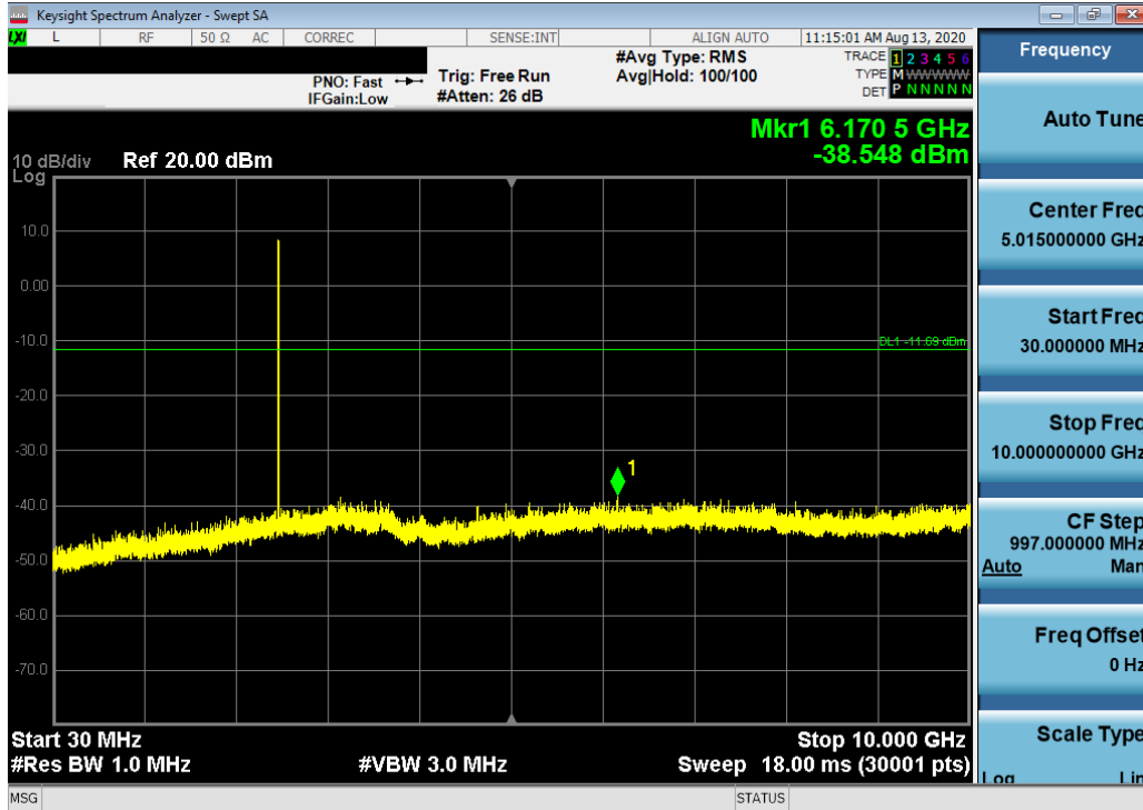
Plot 7-10. Conducted Spurious Plot (Bluetooth (LE), 1Mbps – Ch. 39)
