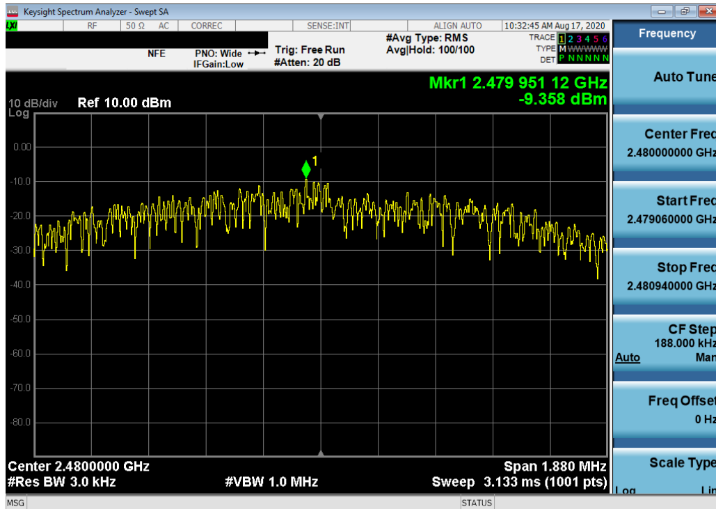
Plot 7-36. Power Spectral Density Plot (Bluetooth (LE), 2Mbps – Ch. 39)
