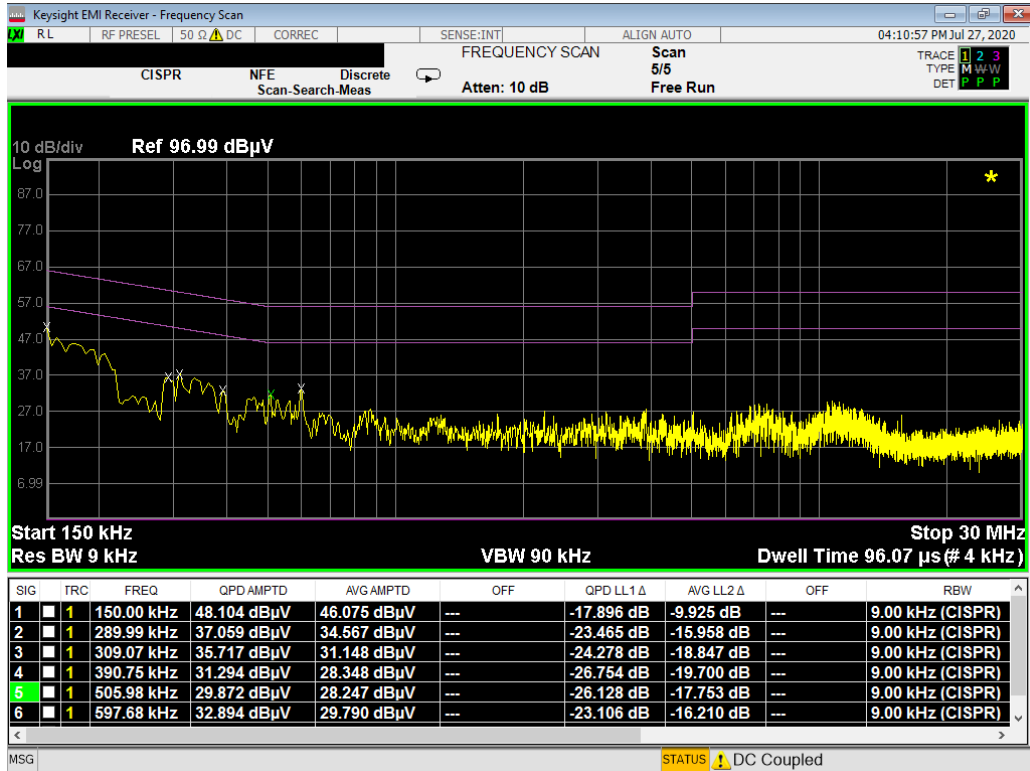
Plot 7-14. Line Conducted Plot with Bluetooth LE (L1)
