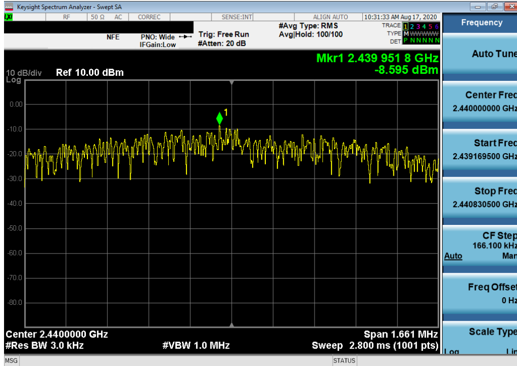
Plot 7-35. Power Spectral Density Plot (Bluetooth (LE), 2Mbps – Ch. 19)
