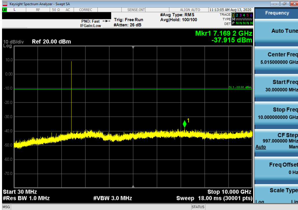
Plot 7-8. Conducted Spurious Plot (Bluetooth (LE), 1Mbps – Ch. 19)
