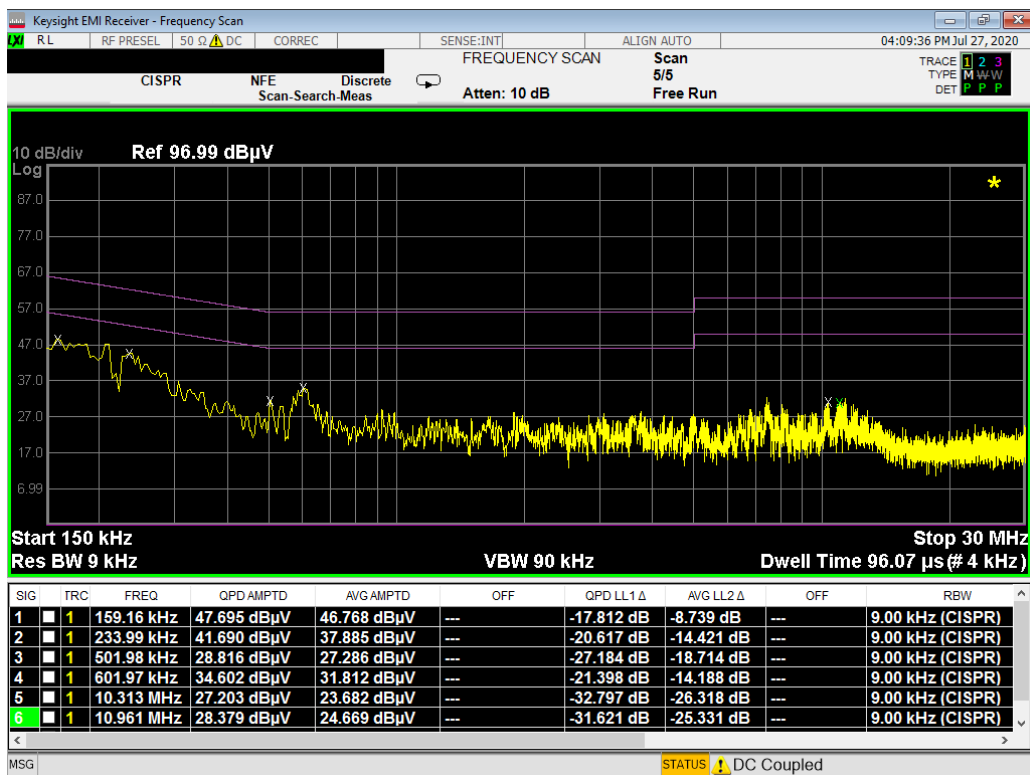
Plot 7-15. Line Conducted Plot with Bluetooth LE (N)
