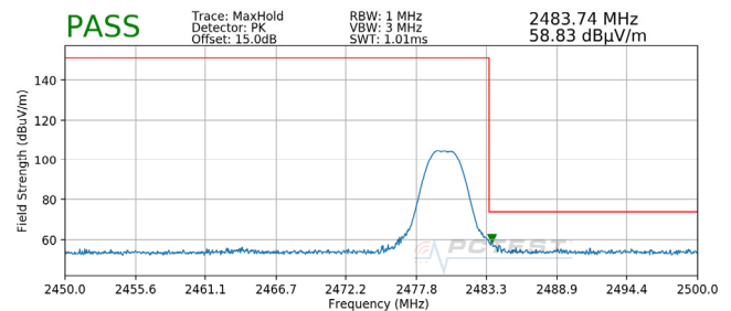
Plot 7-13. Radiated Restricted Upper Band Edge Measurement (Peak)
