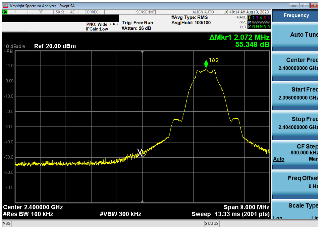
Plot 7-4. Band Edge Plot (Bluetooth (LE), 1Mbps – Ch. 0)
