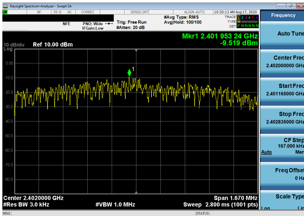
Plot 7-34. Power Spectral Density Plot (Bluetooth (LE), 2Mbps – Ch. 0)
