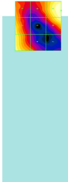
Figure 11-1 Sample E-field Scan Overlay (T-Coil centered scan area pictured. See Test Setup Photographs for acoustic centered scan area and actual WD overlay)
