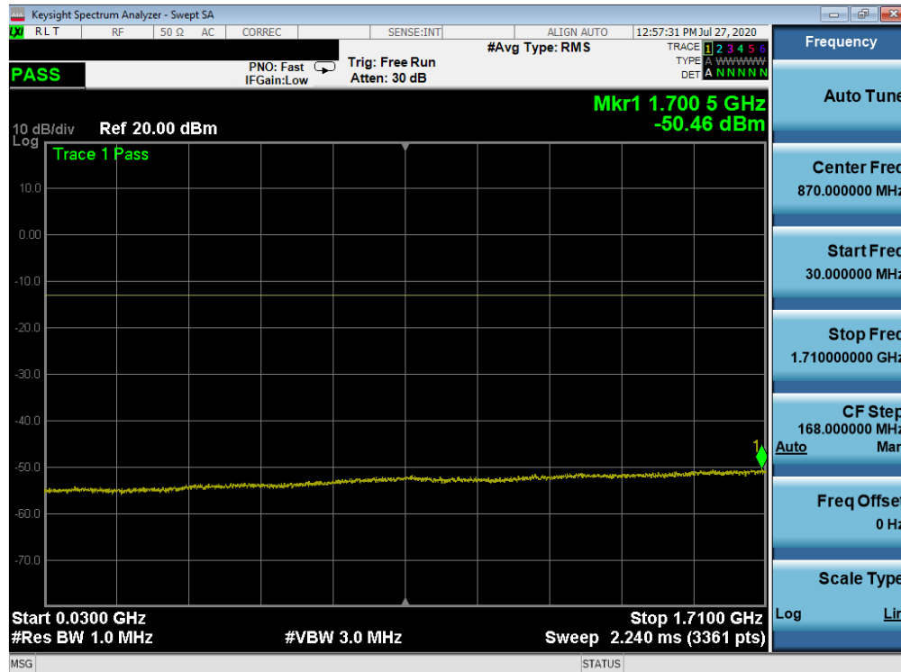
Plot 7-275. Conducted Spurious Plot (NR Band n66 - 20.0MHz - RB Size 1, RB Offset 0 - High Channel)
