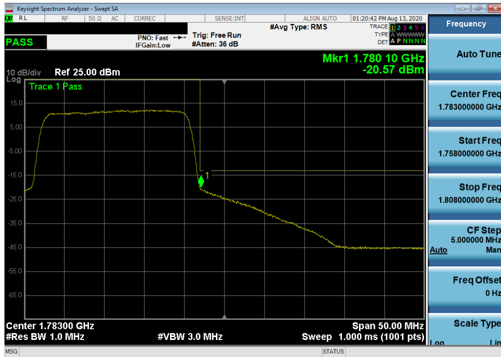
Plot 7-417. Upper Extended Band Edge Plot (NR Band n66 – 20.0MHz - Full RB)
