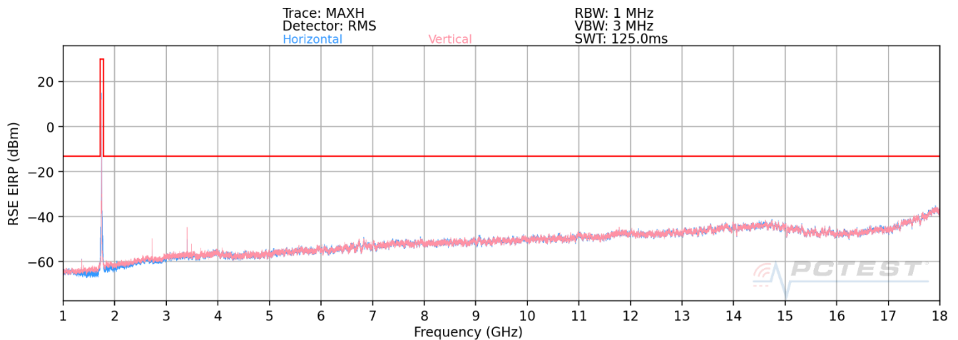
Plot 7-575. Radiated Spurious Plot above 1GHz (n71 + B66)
