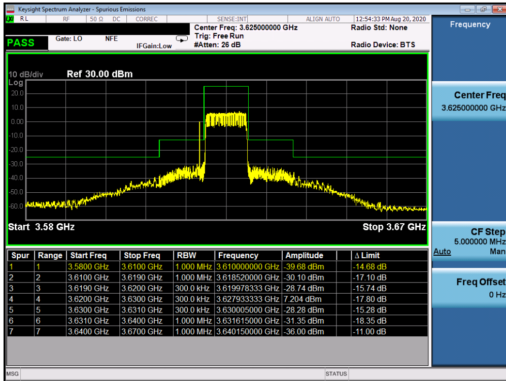
Plot 7-29. Mid ACP Plot (LTE Band 48 - 10.0MHz QPSK - Full RB Configuration)
