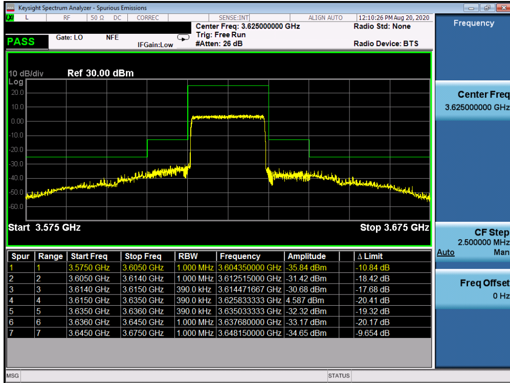
Plot 7-35. Mid ACP Plot (LTE Band 48 - 20.0MHz QPSK - Full RB Configuration)
