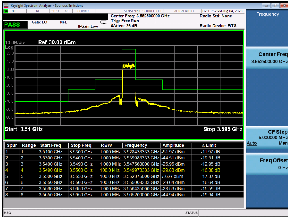
Plot 7-25. Lower ACP Plot (LTE Band 48 - 5.0MHz QPSK - Full RB Configuration)
