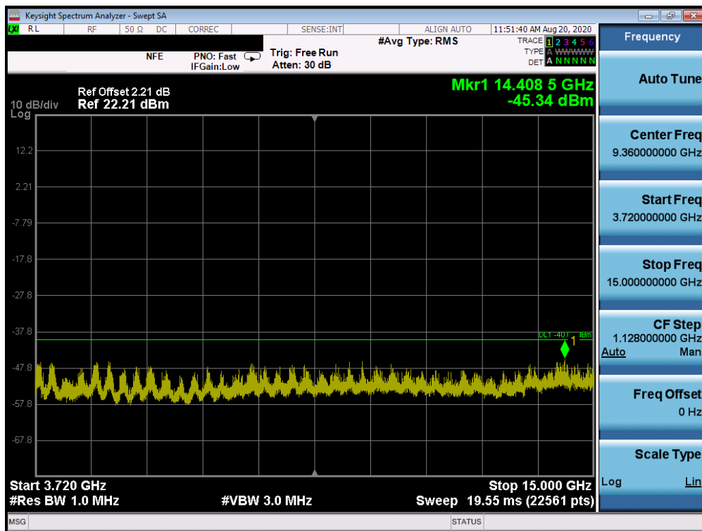
Plot 7-22. Conducted Spurious Plot (LTE Band 48 - 20.0MHz QPSK - RB Size 1, RB Offset 0 - High Channel)
