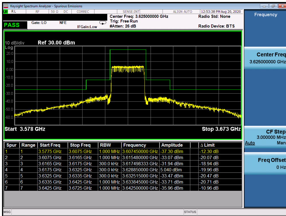
Plot 7-32. Mid ACP Plot (LTE Band 48 - 15.0MHz QPSK - Full RB Configuration)
