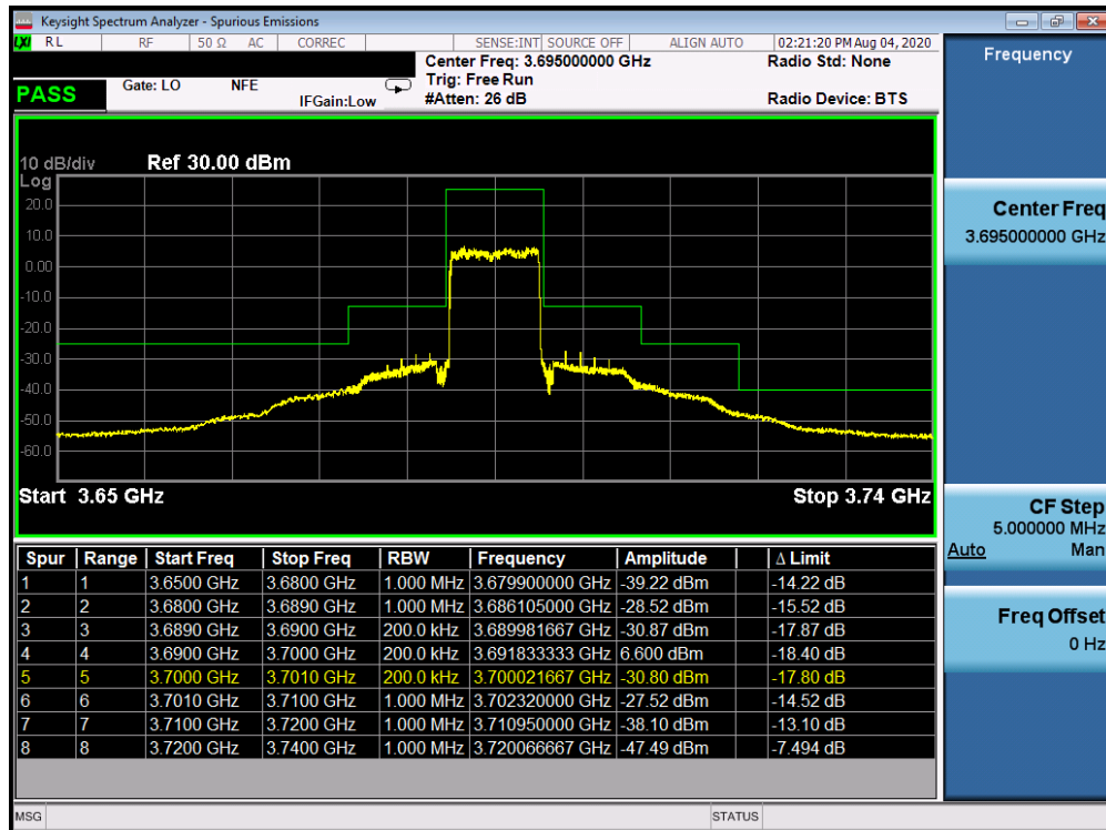
Plot 7-30. Upper ACP Plot (LTE Band 48 - 10.0MHz QPSK - Full RB Configuration)
