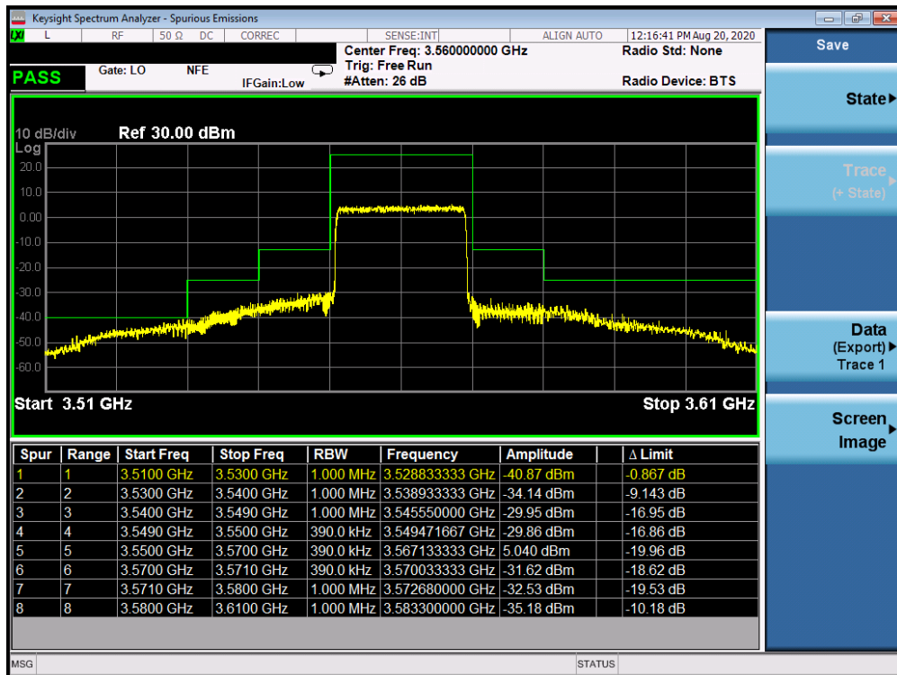
Plot 7-34. Lower ACP Plot (LTE Band 48 - 20.0MHz QPSK - Full RB Configuration)
