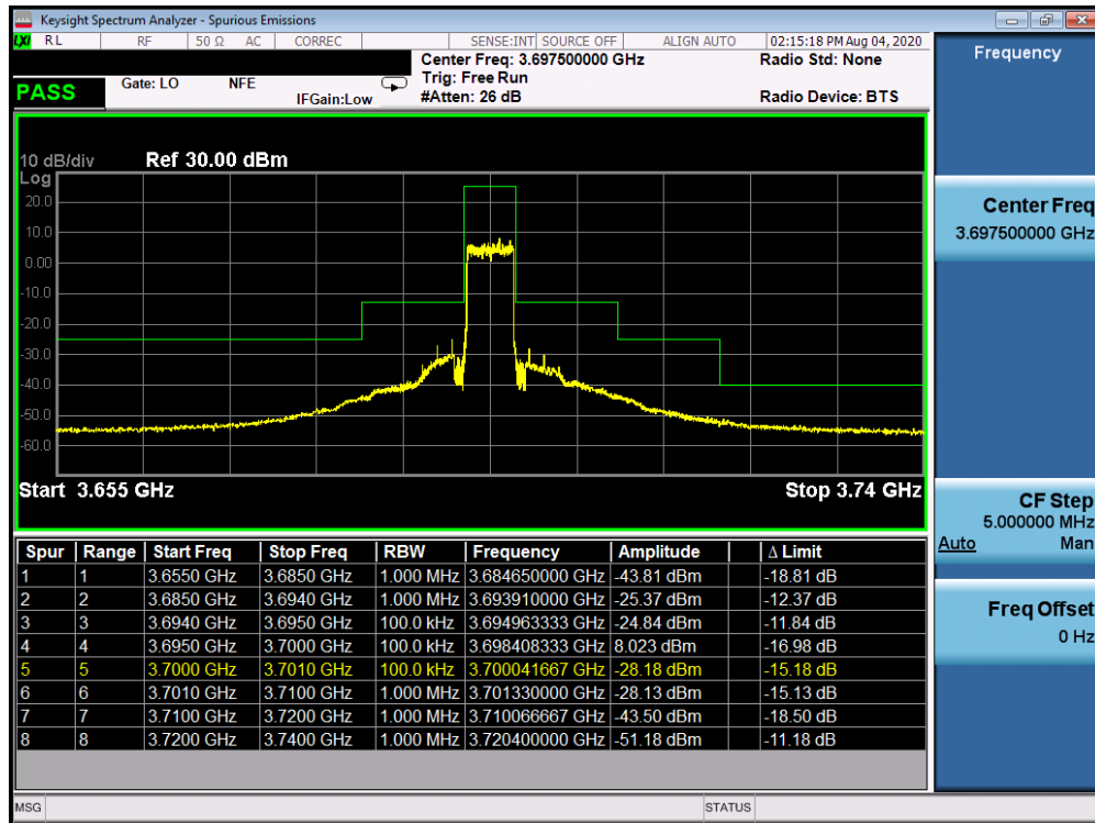
Plot 7-27. Upper ACP Plot (LTE Band 48 - 5.0MHz QPSK - Full RB Configuration)
