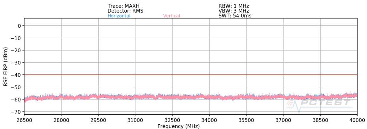
Plot 7-39. Radiated Spurious Plot 26.5 - 40GHz (Band 48)
