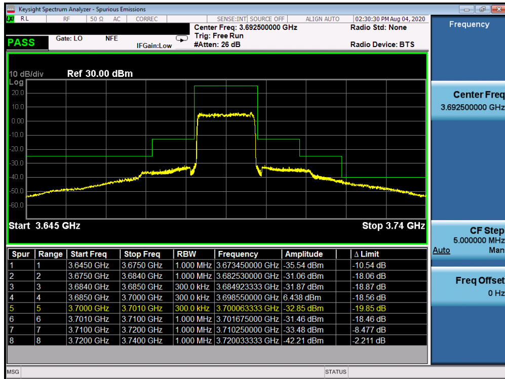
Plot 7-33. Upper ACP Plot (LTE Band 48 - 15.0MHz QPSK - Full RB Configuration)
