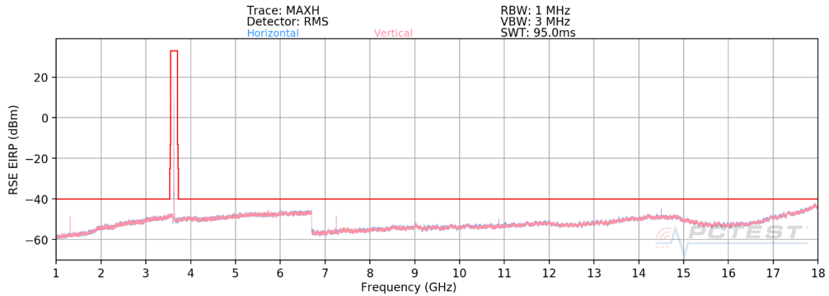
Plot 7-37. Radiated Spurious Plot 1 - 18GHz (Band 48)
