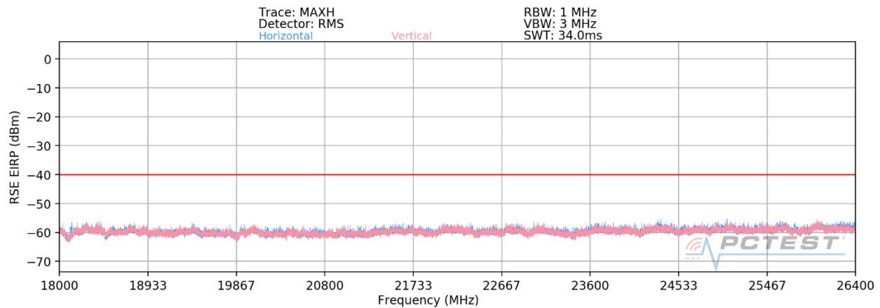
Plot 7-38. Radiated Spurious Plot 18 - 26.5GHz (Band 48)
