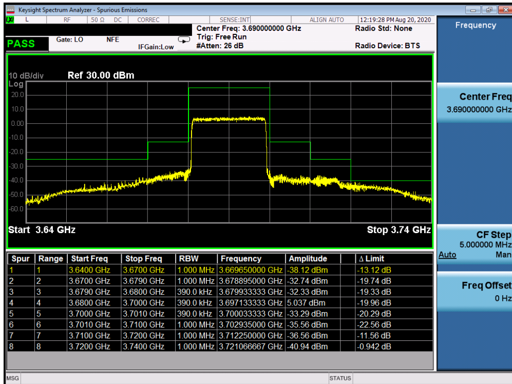
Plot 7-36. Upper ACP Plot (LTE Band 48 - 20.0MHz QPSK - Full RB Configuration)
