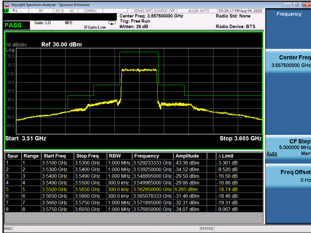
Plot 7-31. Lower ACP Plot (LTE Band 48 - 15.0MHz QPSK - Full RB Configuration)
