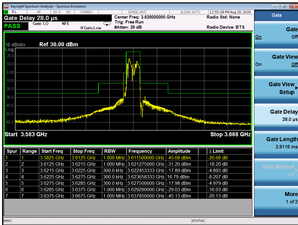
Plot 7-26. Mid ACP Plot (LTE Band 48 - 5.0MHz QPSK - Full RB Configuration)
