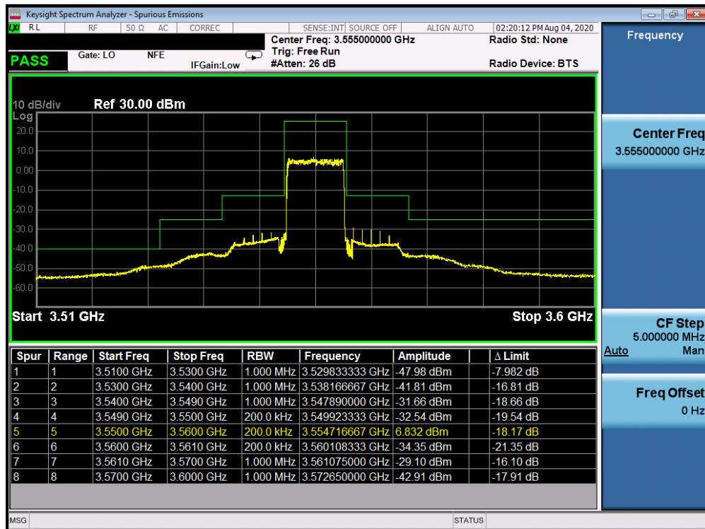
Plot 7-28. Lower ACP Plot (LTE Band 48 - 10.0MHz QPSK - Full RB Configuration)
