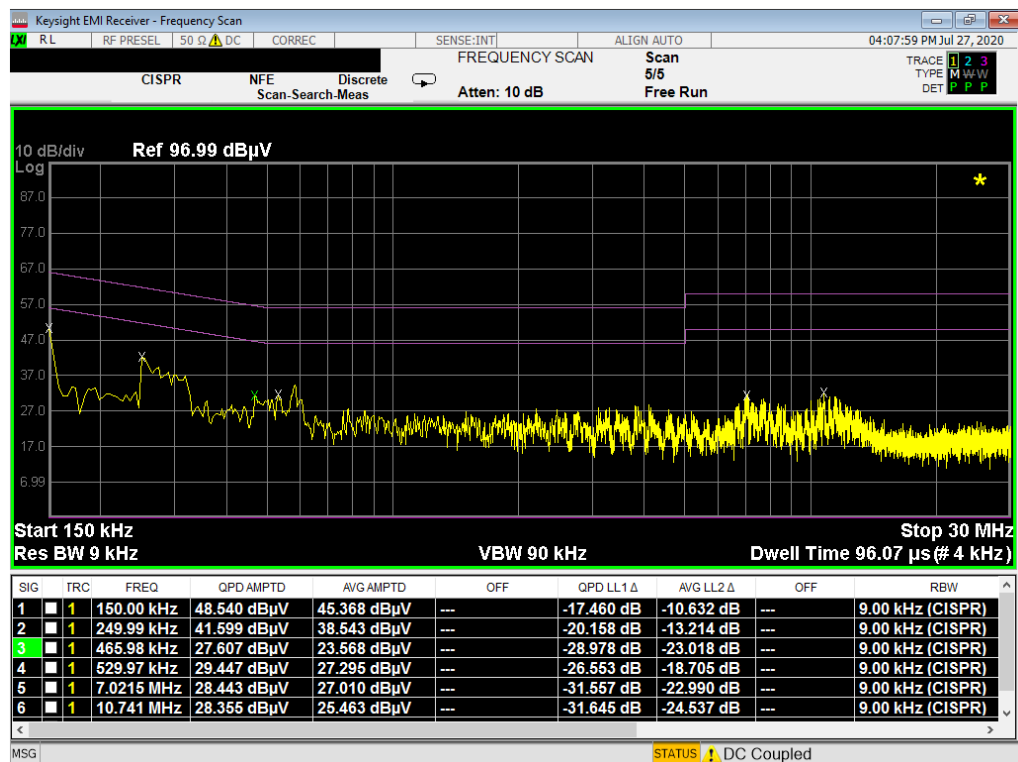
Plot 7-52. Line-Conducted Test Plot (N)
