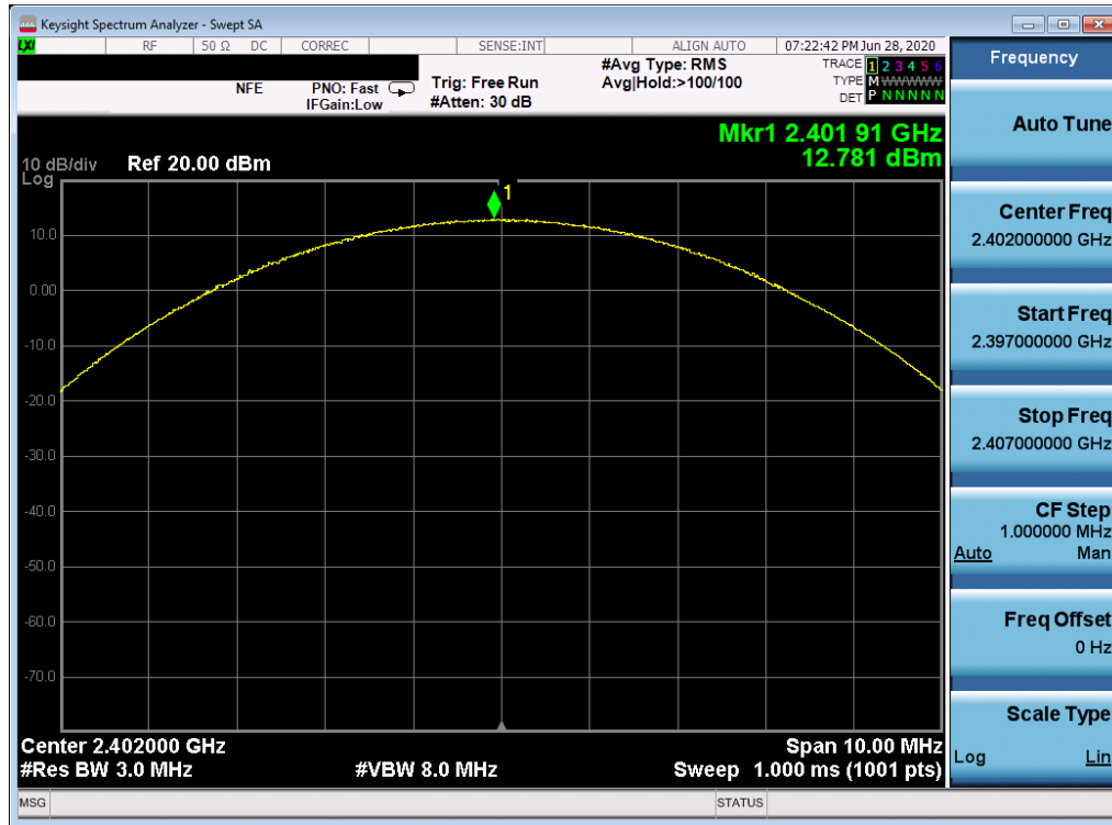
Plot 7-16. Peak Conducted Power (3Mbps – Ch. 0)
