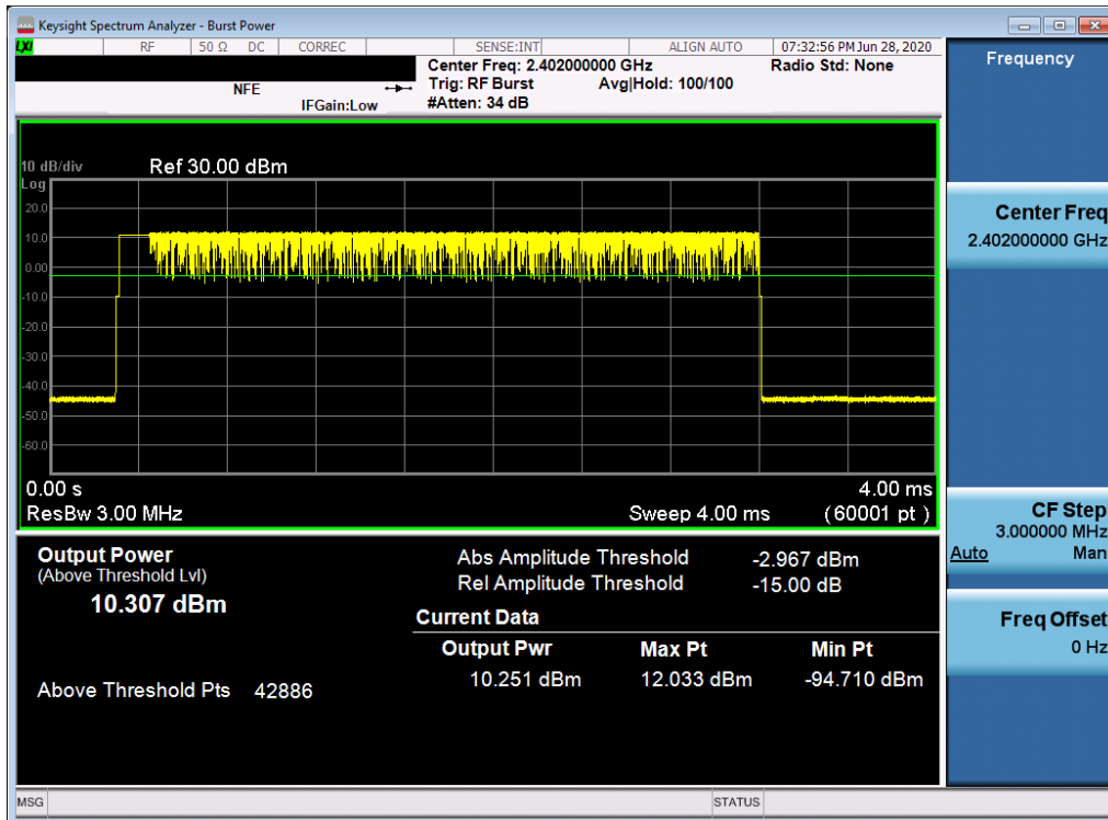
Plot 7-25. Average Conducted Power (3Mbps – Ch. 0)
