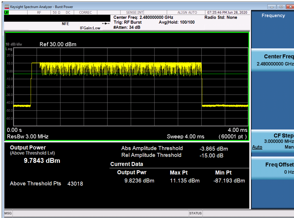
Plot 7-27. Average Conducted Power (3Mbps – Ch. 78)
