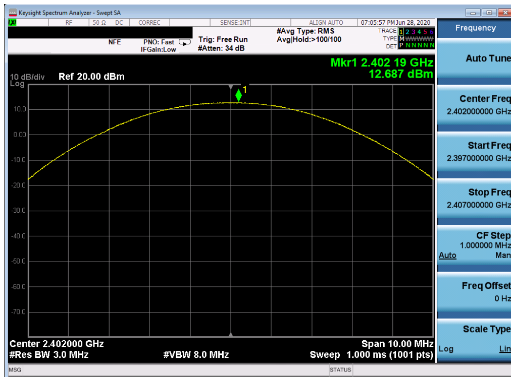
Plot 7-13. Peak Conducted Power (2Mbps – Ch. 0)
