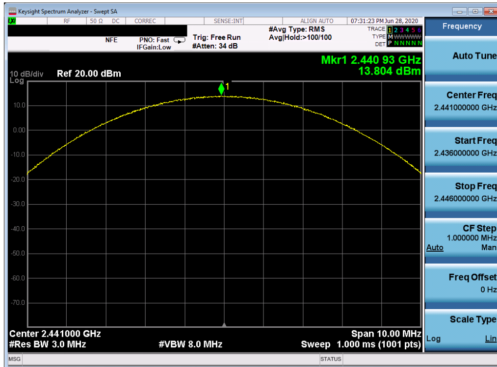
Plot 7-17. Peak Conducted Power (3Mbps – Ch. 39)
