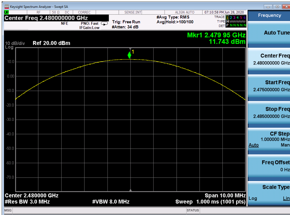
Plot 7-15. Peak Conducted Power (2Mbps – Ch. 78)
