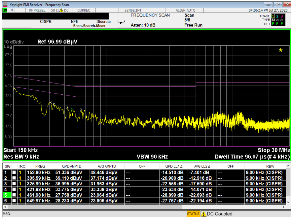
Plot 7-51. Line-Conducted Test Plot (L1)
