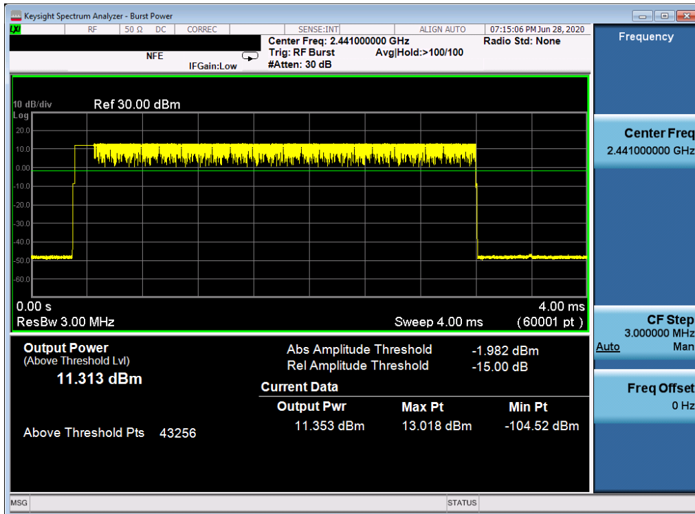
Plot 7-23. Average Conducted Power (2Mbps – Ch. 39)
