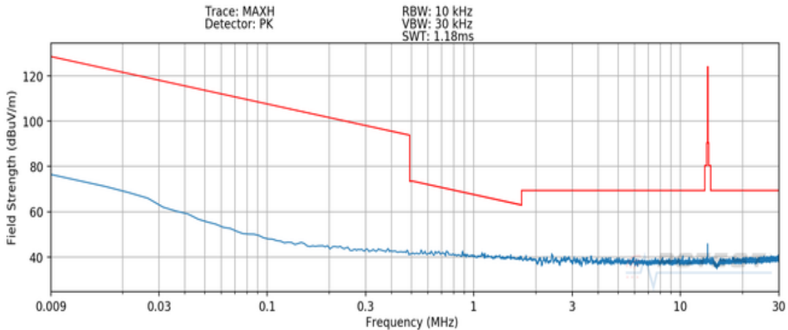
Plot 7-2. Radiated Spurious Plot 9kHz – 30MHz (Pol. Y)
