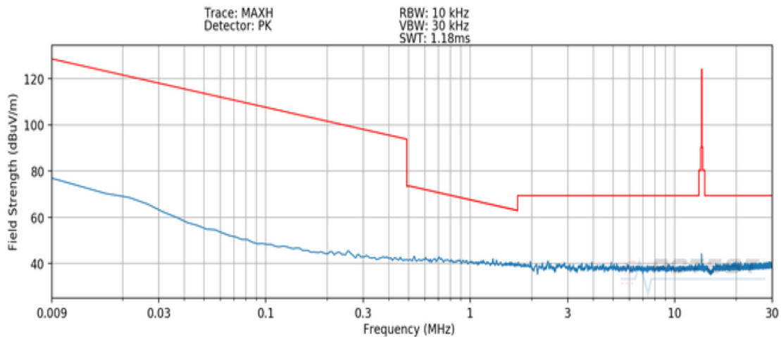
Plot 7-3. Radiated Spurious Plot 9kHz – 30MHz (Pol. Z)
