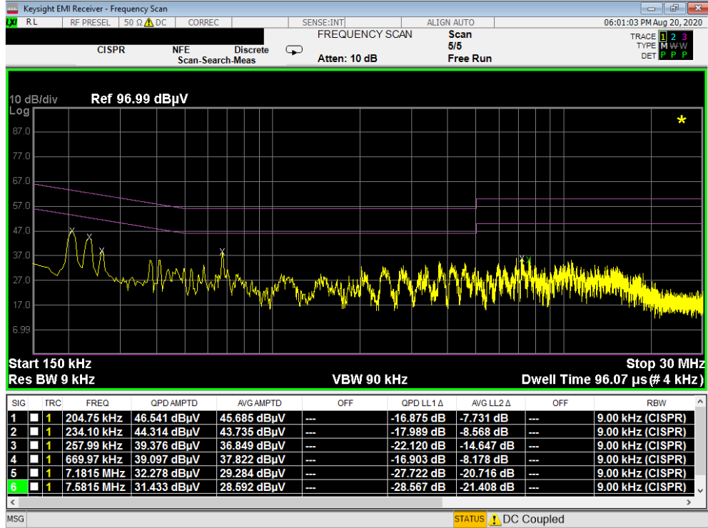
Plot 7-6. Line-Conducted Test Plot (L1) – Terminated in 50Ω
