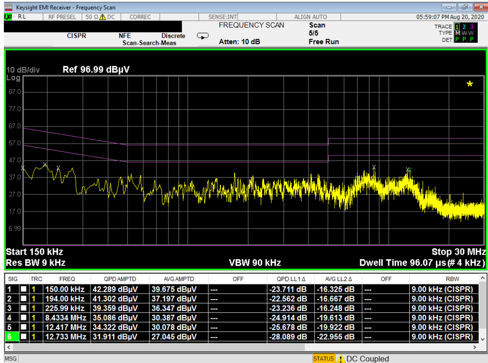
Plot 7-7. Line-Conducted Test Plot (N) – Terminated in 50Ω
