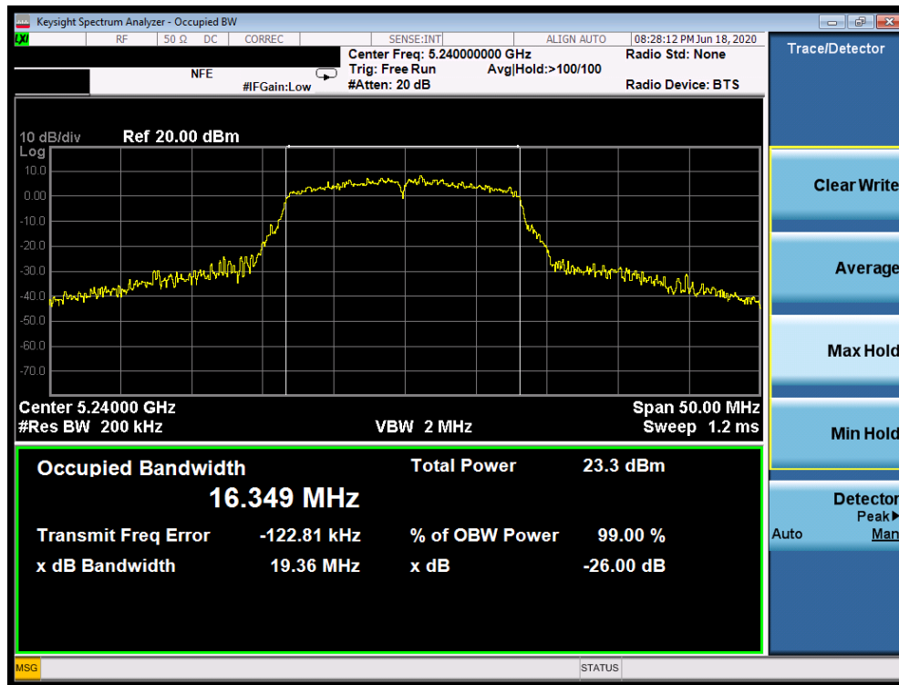
Plot 7-33. 26dB Bandwidth Plot SISO ANT2 (802.11a (UNII Band 1) – Ch. 48)
