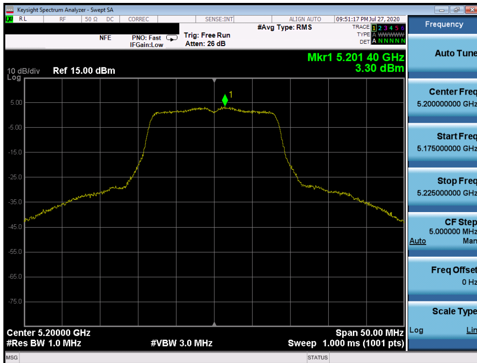
Plot 7-80. Power Spectral Density Plot SISO ANT1 (802.11a (UNII Band 1) – Ch. 40)
