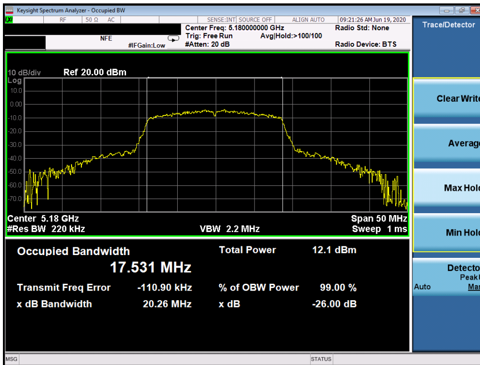
Plot 7-34. 26dB Bandwidth Plot SISO ANT2 (20MHz BW 802.11n (UNII Band 1) – Ch. 36)
