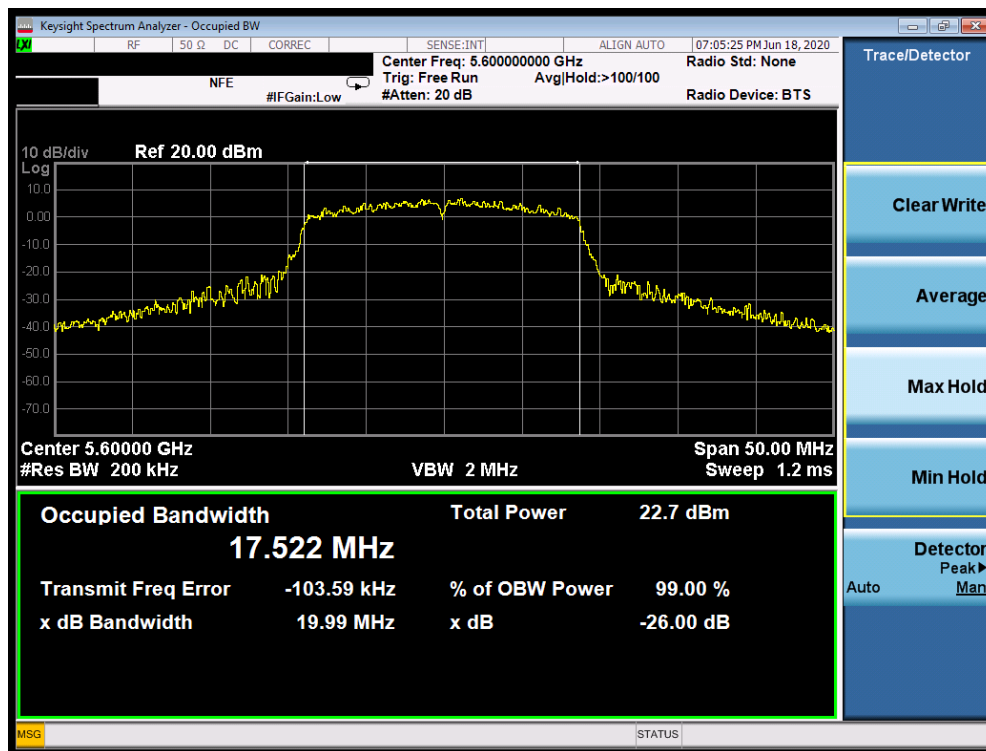
Plot 7-23. 26dB Bandwidth Plot SISO ANT1 (20MHz BW 802.11n (UNII Band 2C) – Ch. 120)
