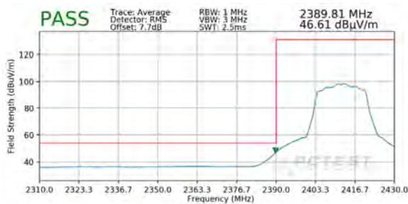
Plot 7-77. Radiated Restricted Lower Band Edge Measurement SISO ANT2 (Average)
