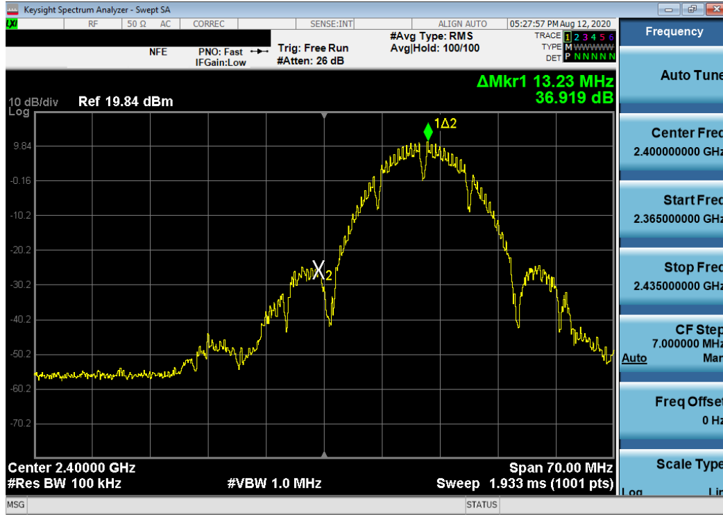
Plot 7-43. Band Edge Plot SISO ANT2 (802.11b – Ch. 1)
