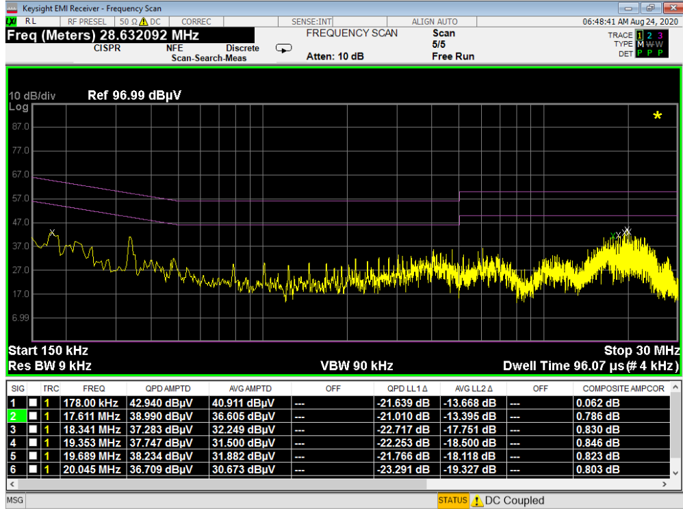
Plot 7-888. Line Conducted Plot with 802.11b (L1) WCP
