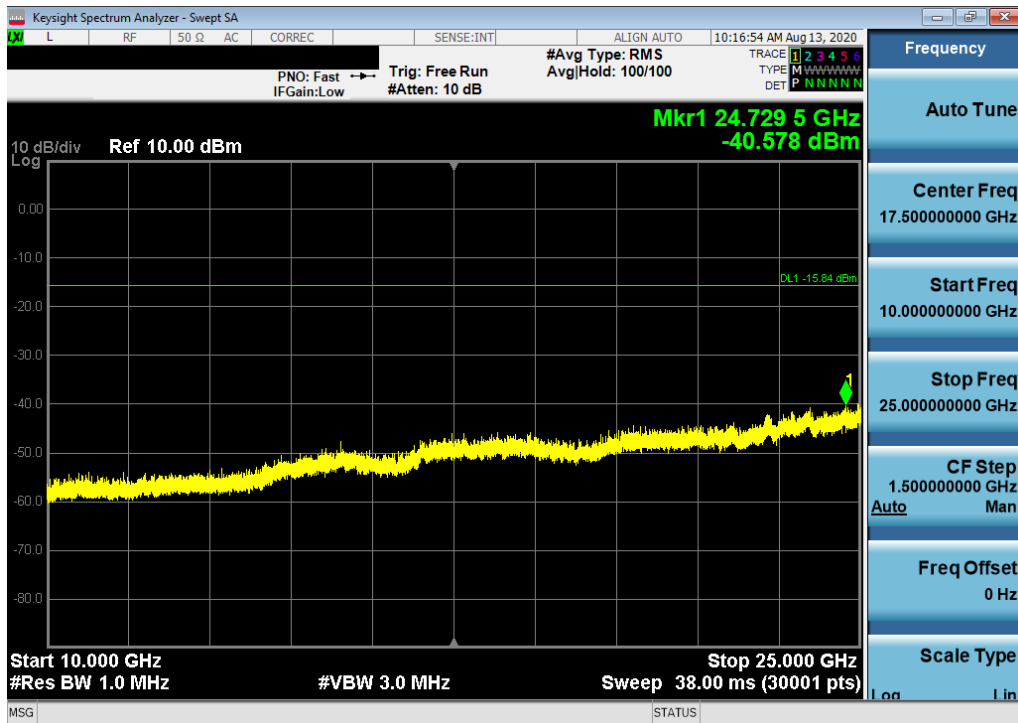
Plot 7-54. Conducted Spurious Plot SISO ANT1 (802.11b – Ch. 11)
