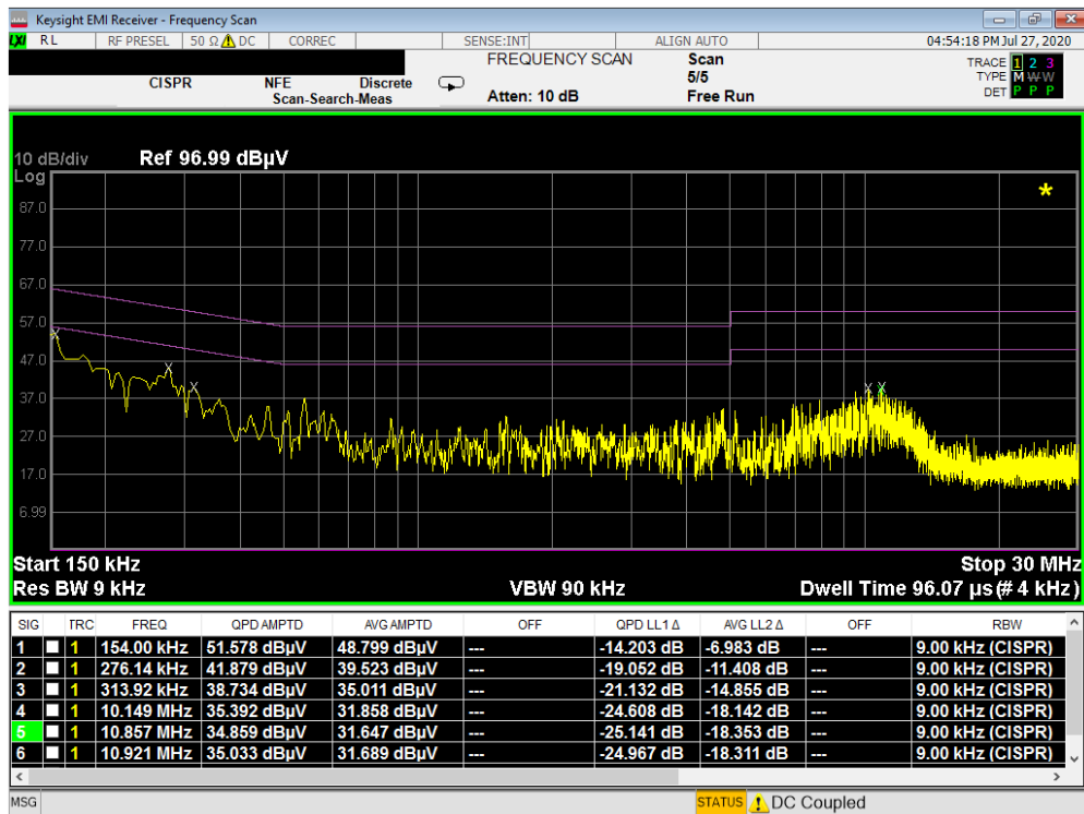
Plot 7-87. Line Conducted Plot with 802.11b (N)
