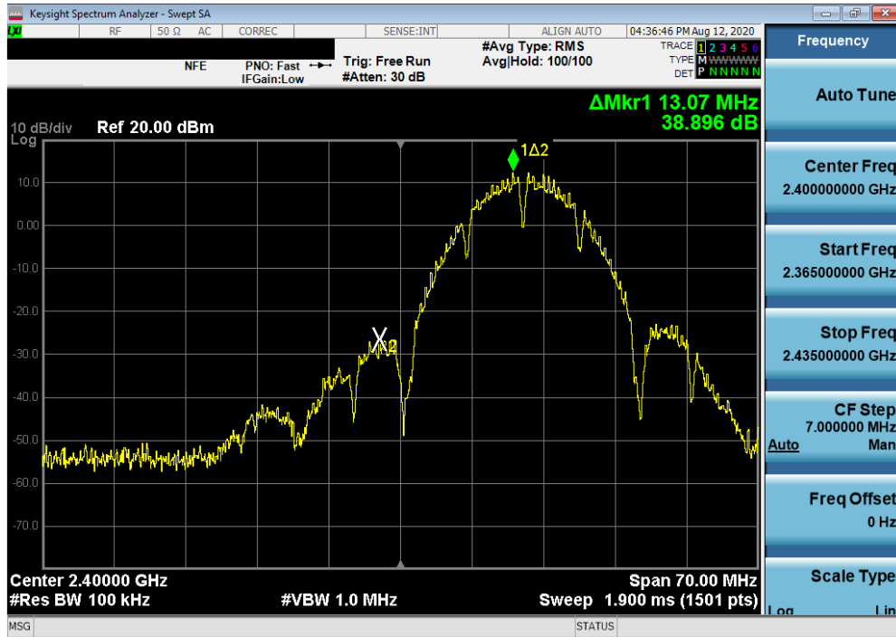
Plot 7-37. Band Edge Plot SISO ANT1 (802.11b – Ch. 1)
