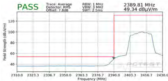
Plot 7-73. Radiated Restricted Lower Band Edge Measurement SISO ANT1 (Average)
