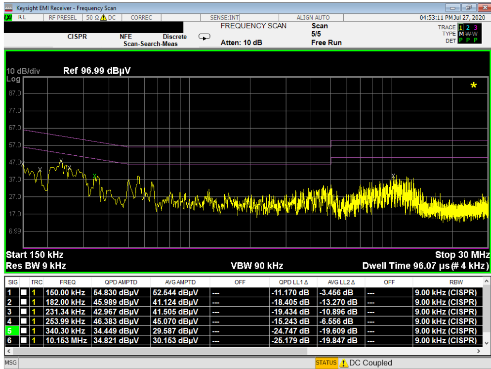
Plot 7-86. Line Conducted Plot with 802.11b (L1)
