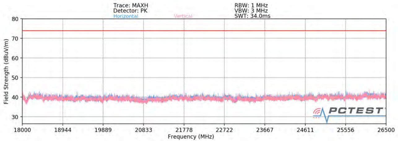
Plot 7-72. Radiated Spurious Plot above 18GHz MIMO/CDD
