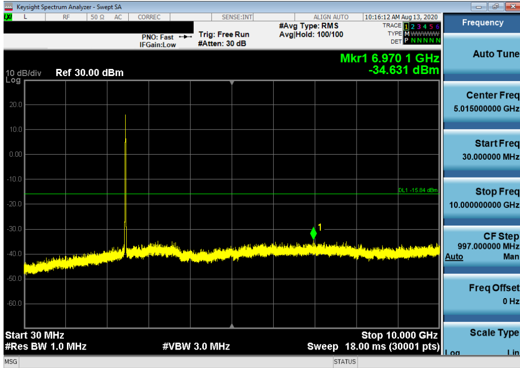
Plot 7-53. Conducted Spurious Plot SISO ANT1 (802.11b – Ch. 11)
