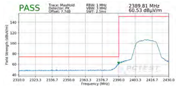
Plot 7-78. Radiated Restricted Lower Band Edge Measurement SISO ANT2 (Peak)
