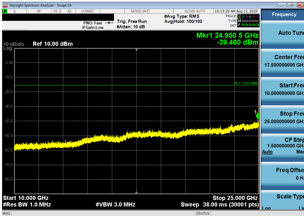
Plot 7-52. Conducted Spurious Plot SISO ANT1 (802.11b – Ch. 6)
