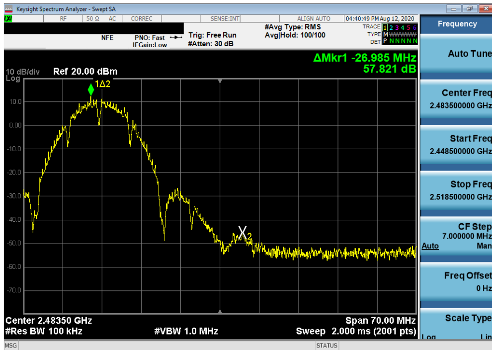
Plot 7-38. Band Edge Plot SISO ANT1 (802.11b – Ch. 11)
