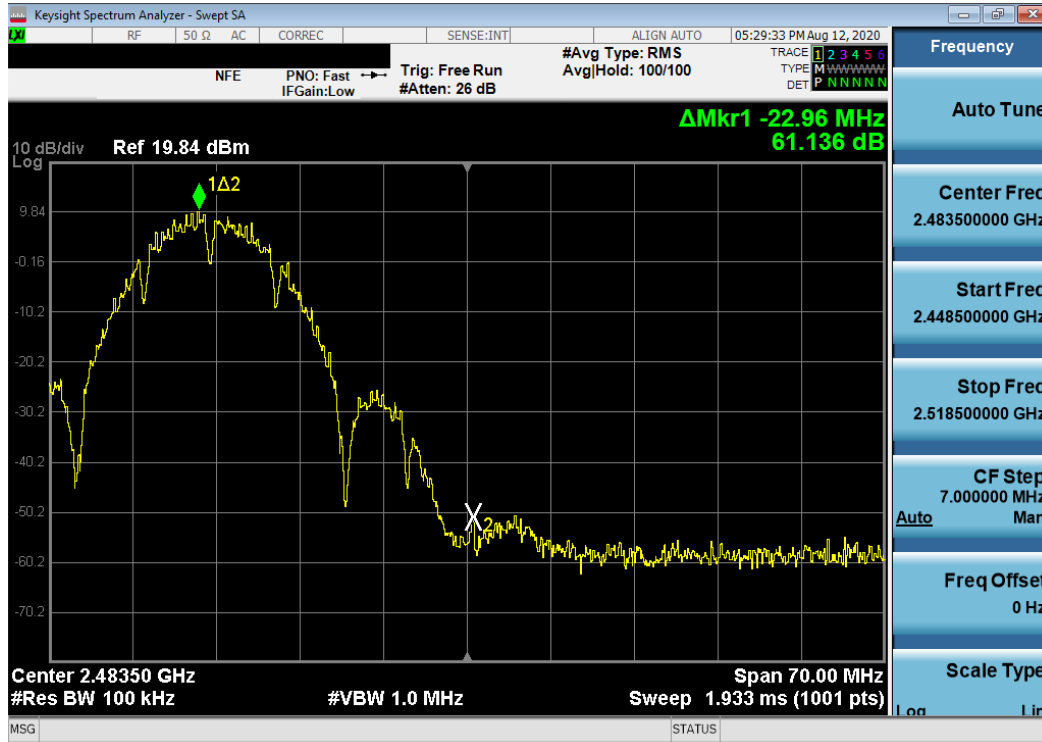
Plot 7-44. Band Edge Plot SISO ANT2 (802.11b – Ch. 11)
