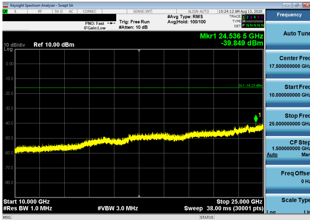
Plot 7-58. Conducted Spurious Plot SISO ANT2 (802.11b – Ch. 6)
