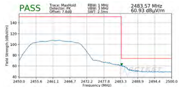
Plot 7-80. Radiated Restricted Upper Band Edge Measurement SISO ANT2 (Peak)
