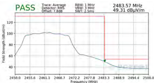
Plot 7-75. Radiated Restricted Upper Band Edge Measurement SISO ANT1 (Average)
