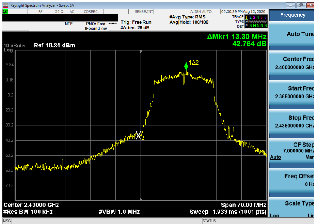
Plot 7-45. Band Edge Plot SISO ANT2 (802.11g- Ch. 1)
