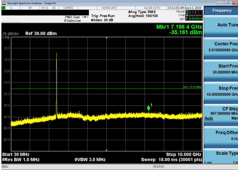
Plot 7-49. Conducted Spurious Plot SISO ANT1 (802.11b – Ch. 1)
