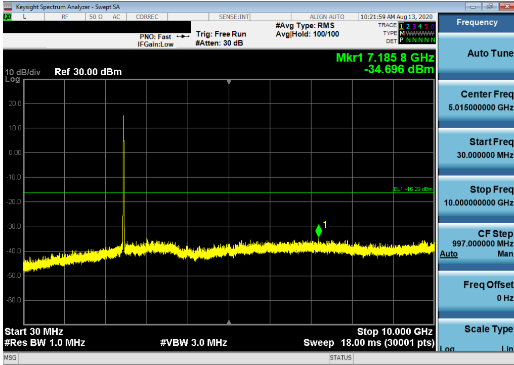
Plot 7-59. Conducted Spurious Plot SISO ANT2 (802.11b – Ch. 11)
