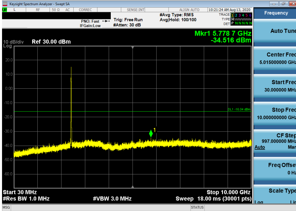
Plot 7-57. Conducted Spurious Plot SISO ANT2 (802.11b – Ch. 6)
