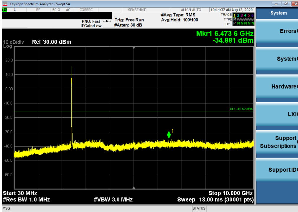
Plot 7-51. Conducted Spurious Plot SISO ANT1 (802.11b – Ch. 6)
