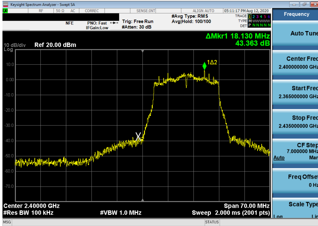
Plot 7-41. Band Edge Plot SISO ANT1 (802.11n (2.4GHz) – Ch. 1)
