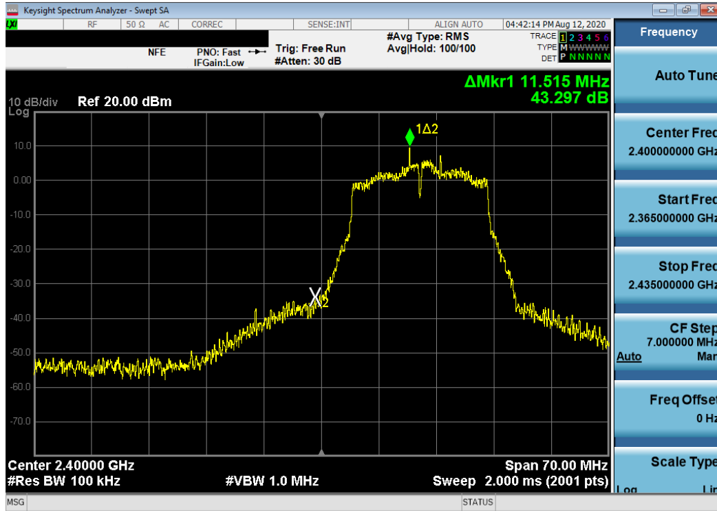
Plot 7-39. Band Edge Plot SISO ANT1 (802.11g- Ch. 1)
