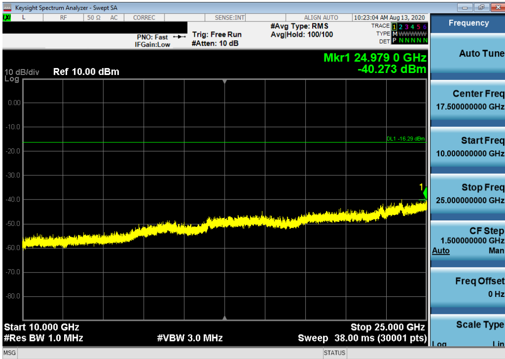
Plot 7-60. Conducted Spurious Plot SISO ANT2 (802.11b – Ch. 11)
