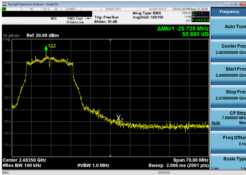
Plot 7-40. Band Edge Plot SISO ANT1 (802.11g - Ch. 11)
