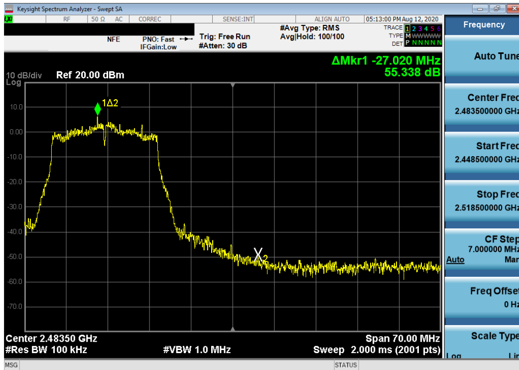
Plot 7-42. Band Edge Plot SISO ANT1 (802.11n (2.4GHz) – Ch. 11)
