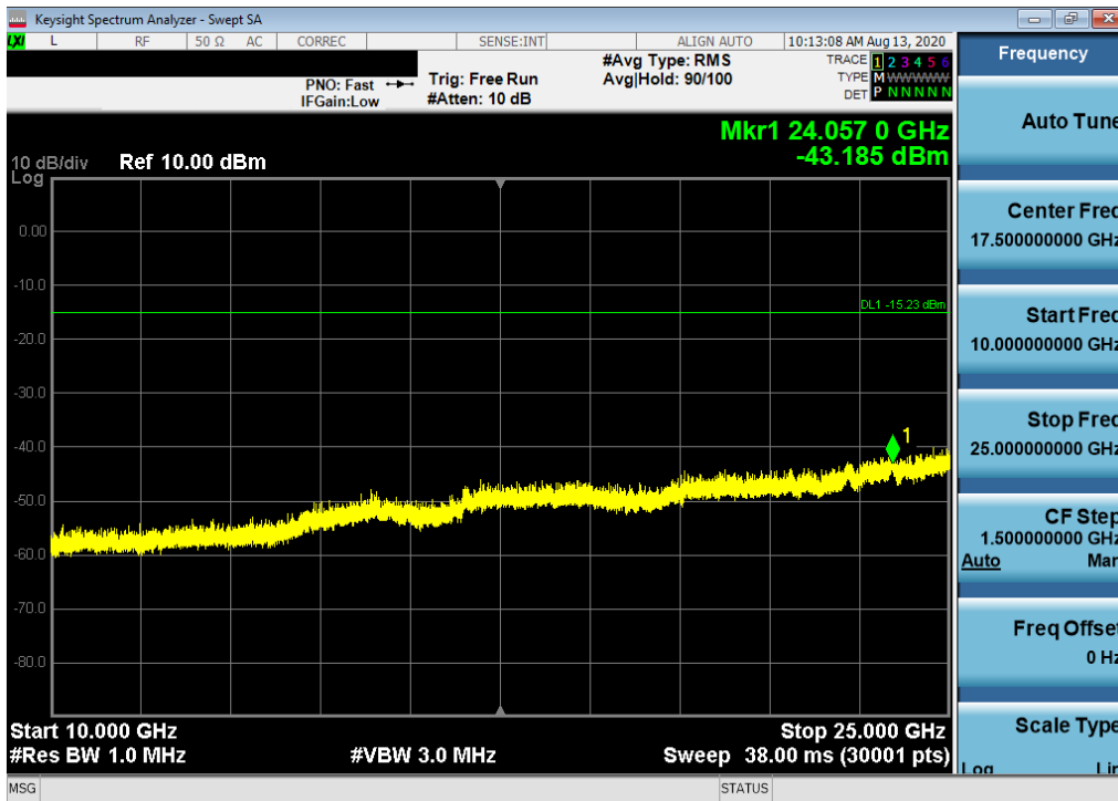
Plot 7-50. Conducted Spurious Plot SISO ANT1 (802.11b – Ch. 1)
