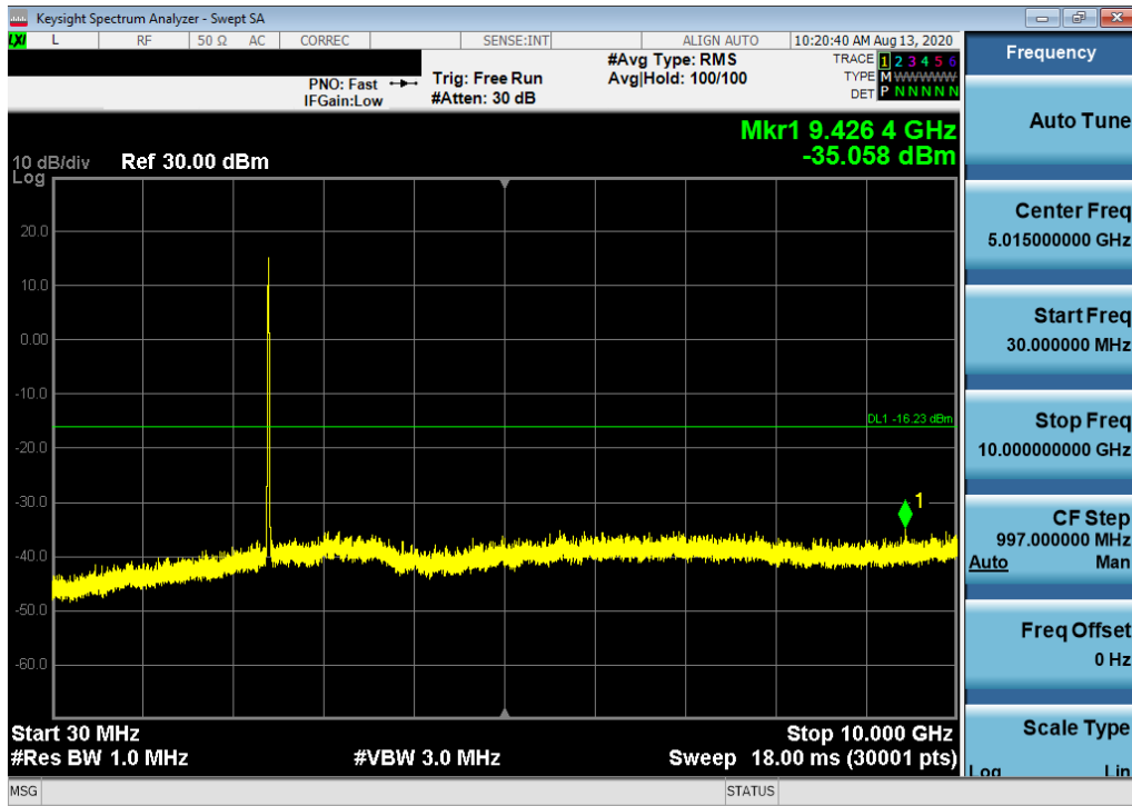
Plot 7-55. Conducted Spurious Plot SISO ANT2 (802.11b – Ch. 1)
