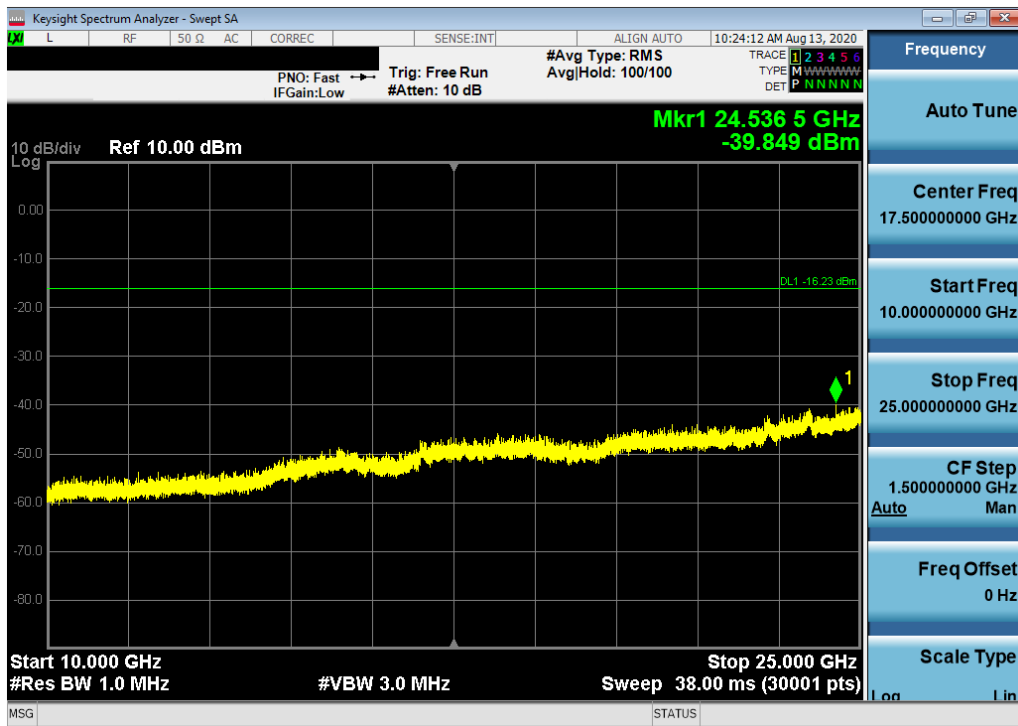
Plot 7-56. Conducted Spurious Plot SISO ANT2 (802.11b – Ch. 1)
