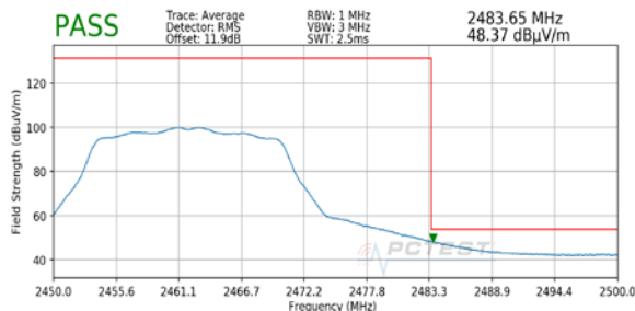
Plot 7-7. Radiated Restricted Upper Band Edge Measurement SISO ANT2 (Average)
