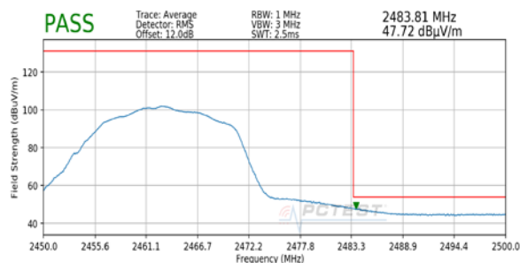
Plot 7-11. Radiated Restricted Upper Band Edge Measurement MIMO (Average)
