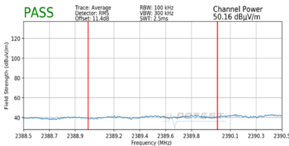
Plot 7-1. Radiated Restricted Lower Band Edge Measurement SISO ANT1 (Average)
