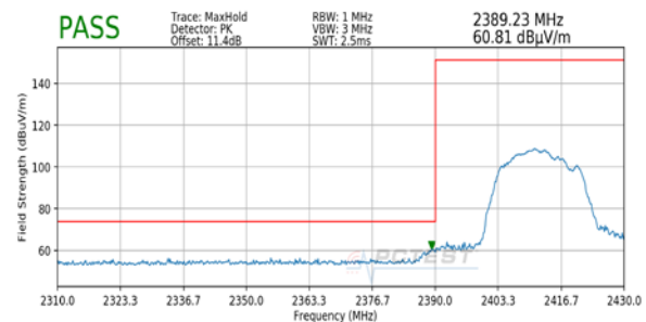
Plot 7-10. Radiated Restricted Lower Band Edge Measurement MIMO (Peak)
