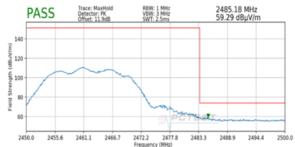
Plot 7-12. Radiated Restricted Upper Band Edge Measurement MIMO (Peak)
