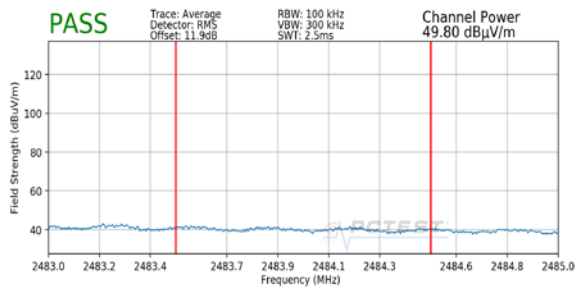
Plot 7-3. Radiated Restricted Upper Band Edge Measurement SISO ANT1 (Average)
