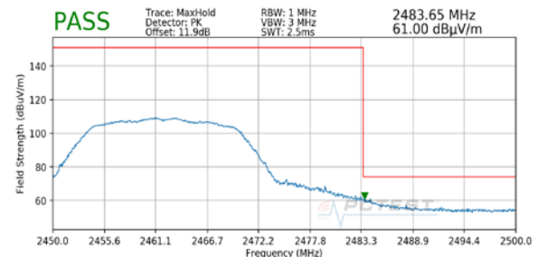
Plot 7-8. Radiated Restricted Upper Band Edge Measurement SISO ANT2 (Peak)
