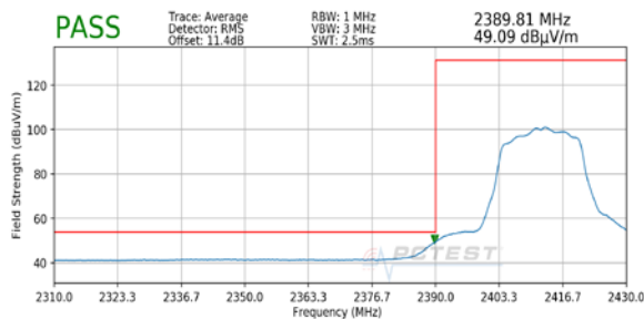
Plot 7-5. Radiated Restricted Lower Band Edge Measurement SISO ANT2 (Average)
