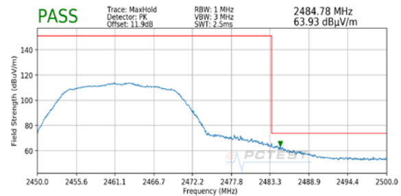
Plot 7-4. Radiated Restricted Upper Band Edge Measurement SISO ANT1 (Peak)
