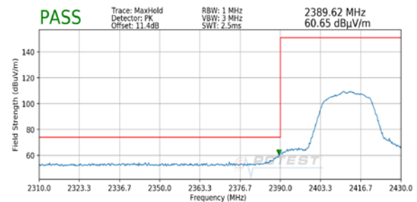
Plot 7-6. Radiated Restricted Lower Band Edge Measurement SISO ANT2 (Peak)
