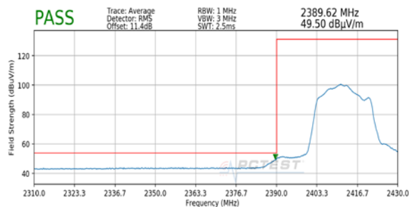
Plot 7-9. Radiated Restricted Lower Band Edge Measurement MIMO (Average)
