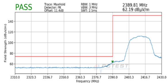
Plot 7-2. Radiated Restricted Lower Band Edge Measurement SISO ANT1 (Peak)
