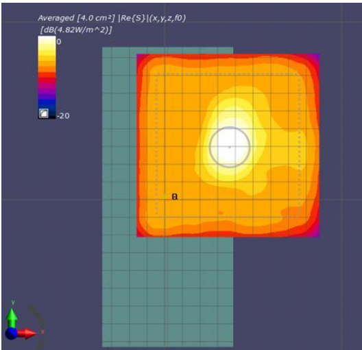
Figure 10-2 4cm 2 psPD distribution measured at input.power.limit of 4.8 dBm on the back surface for n260 beam 30
