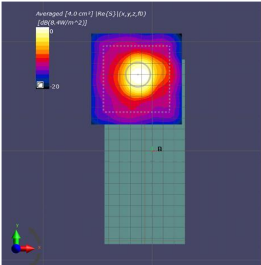
Figure 10-1 4cm 2 psPD distribution measured at input.power.limit of 4.3 dBm on the back surface for n261 beam 20
