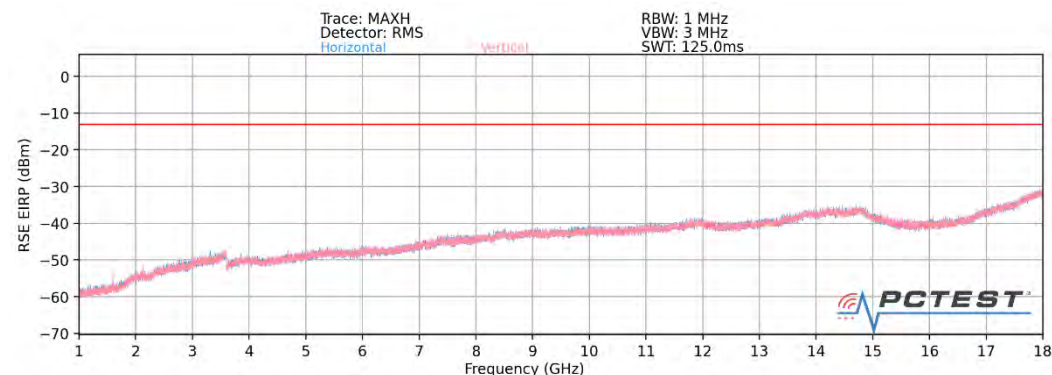
Plot 7-48. Ant 3 - n260 Radiated Spurious Plot (1CC \pi/2 BPSK Mid Channel MIMO)
