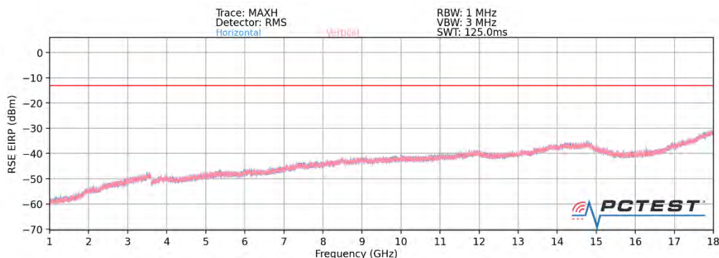
Plot 7-48. Ant 1-n260 Radiated Spurious Plot (1CC \pi/2 BPSK Mid Channel MIMO)
