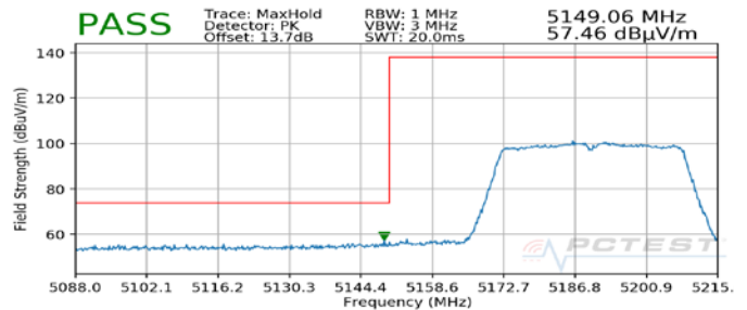
Plot 7-30. Radiated Lower Band Edge Plot SISO ANT2 (Peak – UNII Band 1)
