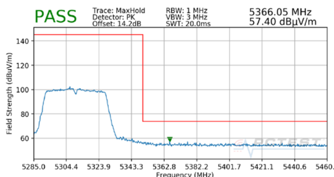
Plot 7-11. Radiated Upper Band Edge Plot SISO ANT1 (Peak – UNII Band 2A)
