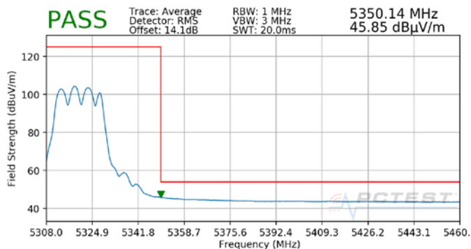
Plot 7-45. Radiated Upper Band Edge Plot MIMO (Average – UNII Band 2A)
