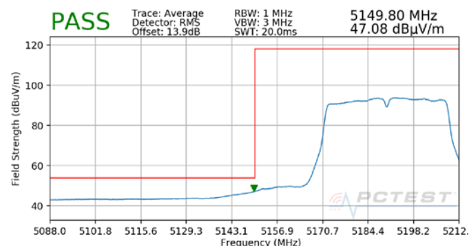
Plot 7-50. Radiated Lower Band Edge Plot MIMO (Average – UNII Band 1)
