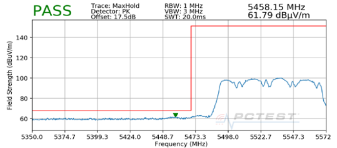
Plot 7-62. Radiated Lower Band Edge Plot MIMO (Peak – UNII Band 2C)
