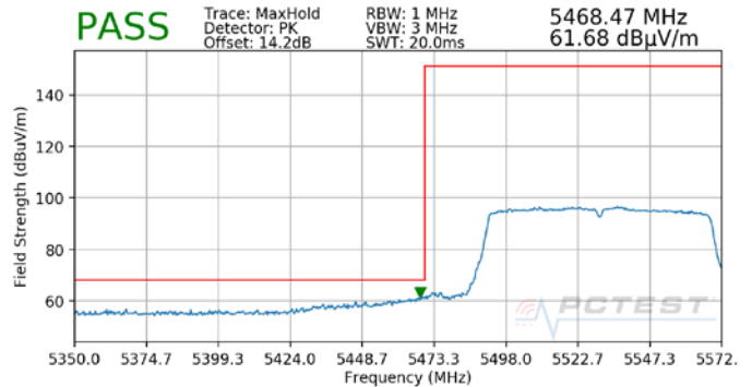
Plot 7-20. Radiated Lower Band Edge Plot SISO ANT1 (Peak - UNII Band 2C)
