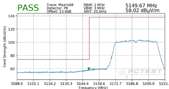
Plot 7-51. Radiated Lower Band Edge Plot MIMO (Peak – UNII Band 1)
