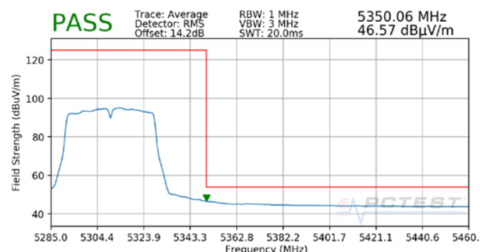
Plot 7-52. Radiated Upper Band Edge Plot MIMO (Average – UNII Band 2A)
