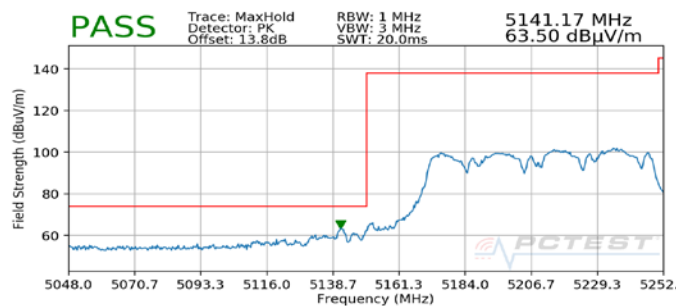
Plot 7-58. Radiated Lower Band Edge Plot MIMO (Peak – UNII Band 1)
