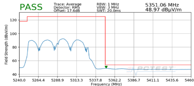
Plot 7-59. Radiated Upper Band Edge Plot MIMO (Average – UNII Band 2A)
