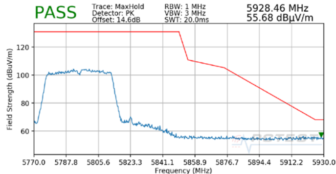
Plot 7-56. Radiated Upper Band Edge Plot MIMO (Peak – UNII Band 3)
