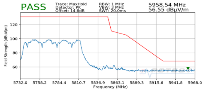
Plot 7-63. Radiated Upper Band Edge Plot MIMO (Peak – UNII Band 3)
