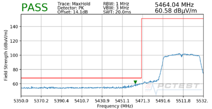
Plot 7-13. Radiated Lower Band Edge Plot SISO ANT1 (Peak - UNII Band 2C)
