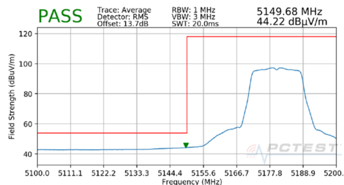
Plot 7-1. Radiated Lower Band Edge Plot SISO ANT1 (Average – UNII Band 1)
