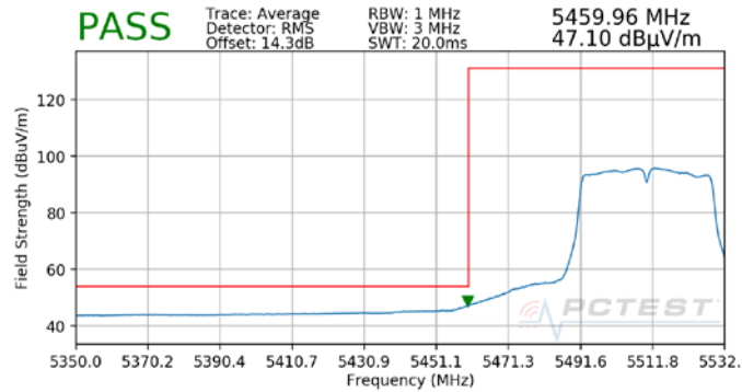
Plot 7-54. Radiated Lower Band Edge Plot MIMO (Average – UNII Band 2C)
