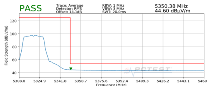
Plot 7-3. Radiated Upper Band Edge Plot SISO ANT1 (Average – UNII Band 2A)
