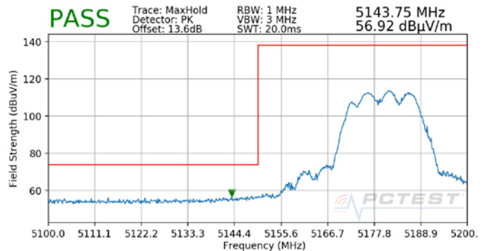
Plot 7-44. Radiated Lower Band Edge Plot MIMO (Peak – UNII Band 1)
