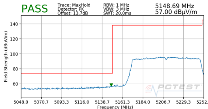
Plot 7-16. Radiated Lower Band Edge Plot SISO ANT1 (Peak – UNII Band 1)
