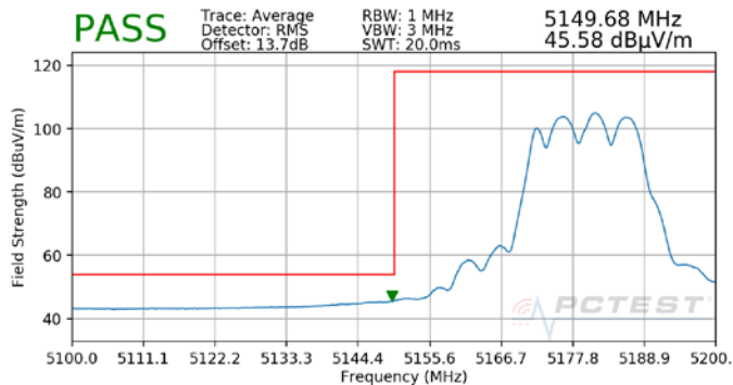
Plot 7-43. Radiated Lower Band Edge Plot MIMO (Average – UNII Band 1)
