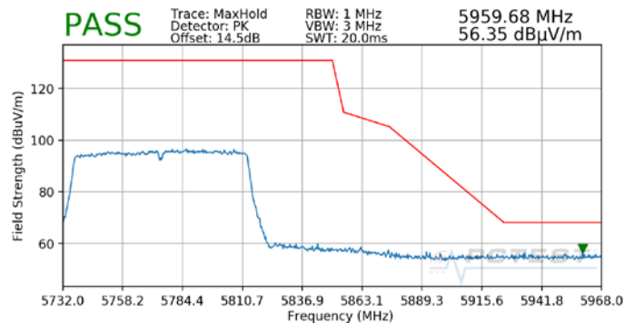
Plot 7-21. Radiated Upper Band Edge Plot SISO ANT1 (Peak - UNII Band 3)
