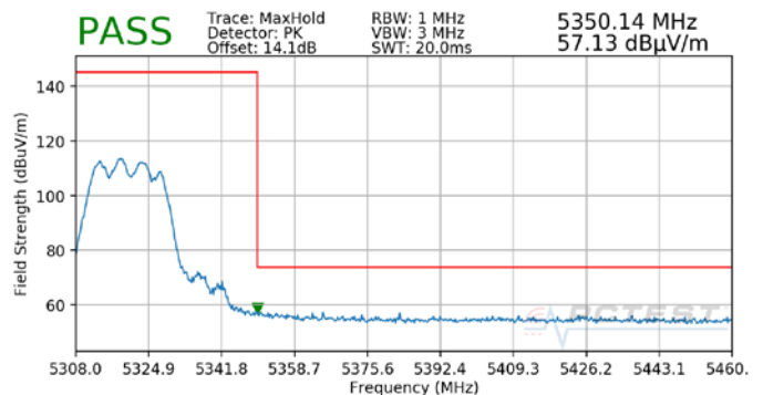
Plot 7-46. Radiated Upper Band Edge Plot MIMO (Peak – UNII Band 2A)
