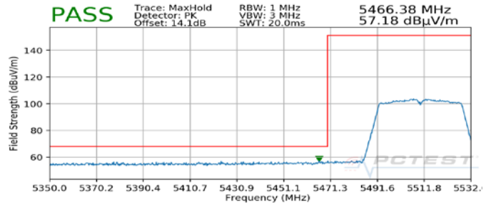
Plot 7-34. Radiated Lower Band Edge Plot SISO ANT2 (Peak - UNII Band 2C)
