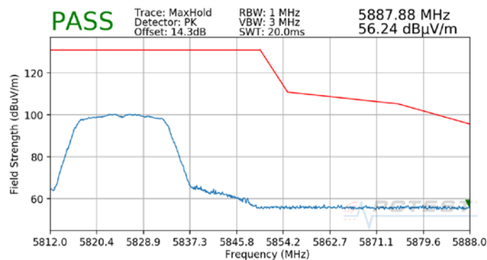
Plot 7-7. Radiated Upper Band Edge Plot SISO ANT1 (Peak – UNII Band 3)
