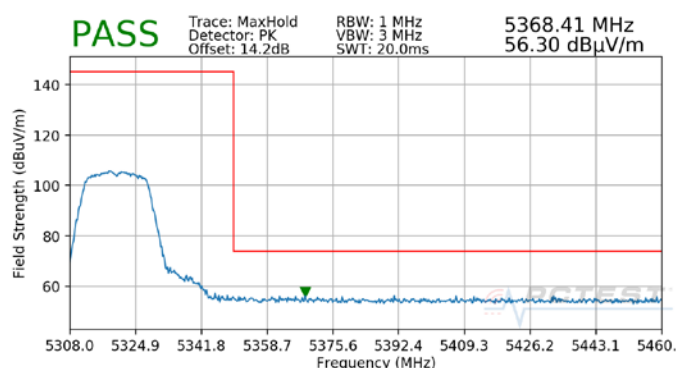
Plot 7-4. Radiated Upper Band Edge Plot SISO ANT1 (Peak – UNII Band 2A)
