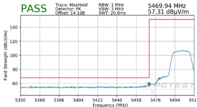
Plot 7-6. Radiated Lower Band Edge Plot SISO ANT1 (Peak – UNII Band 2C)
