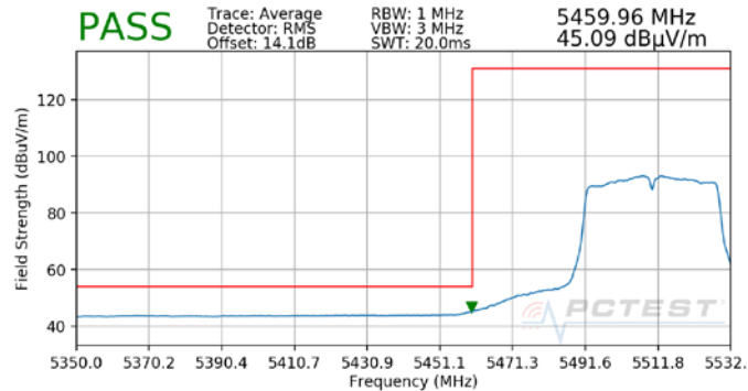
Plot 7-12. Radiated Lower Band Edge Plot SISO ANT1 (Average - UNII Band 2C)
