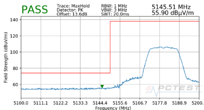
Plot 7-2. Radiated Lower Band Edge Plot SISO ANT1 (Peak – UNII Band 1)
