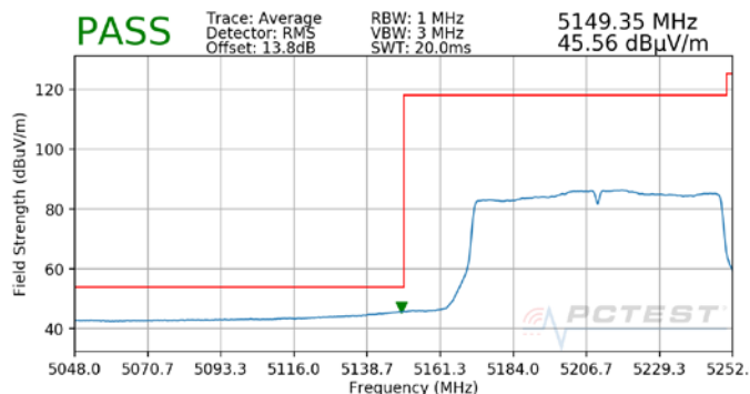
Plot 7-15. Radiated Lower Band Edge Plot SISO ANT1 (Average – UNII Band 1)
