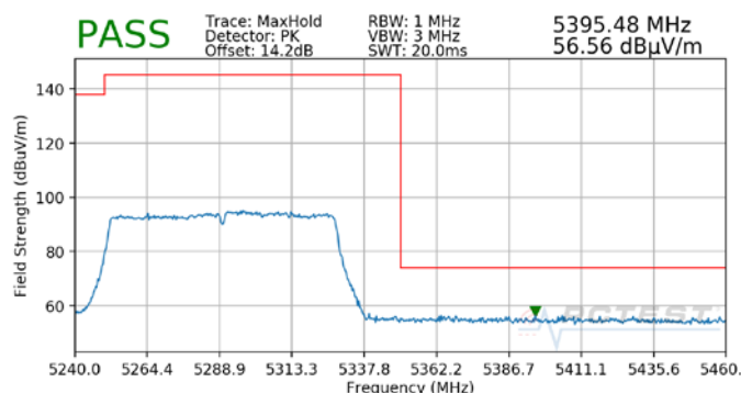
Plot 7-18. Radiated Upper Band Edge Plot SISO ANT1 (Peak – UNII Band 2A)
