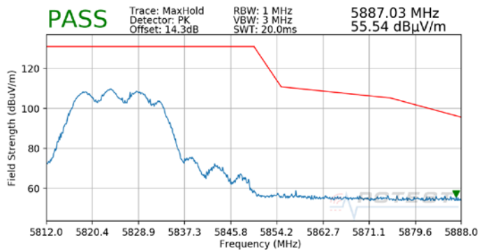
Plot 7-49. Radiated Upper Band Edge Plot MIMO (Peak – UNII Band 3)
