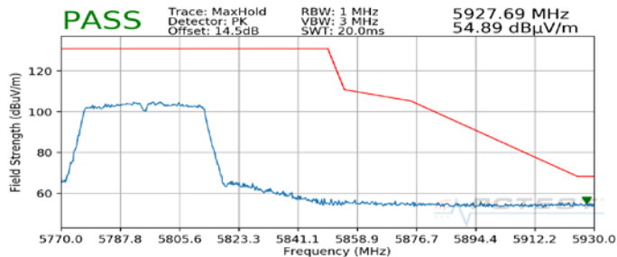
Plot 7-35. Radiated Upper Band Edge Plot SISO ANT2 (Peak - UNII Band 3)
