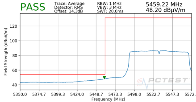
Plot 7-19. Radiated Lower Band Edge Plot SISO ANT1 (Average - UNII Band 2C)
