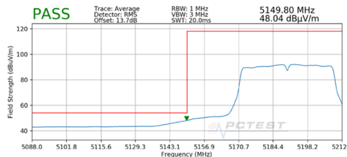
Plot 7-8. Radiated Lower Band Edge Plot SISO ANT1 (Average – UNII Band 1)
