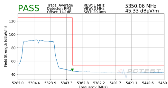
Plot 7-10. Radiated Upper Band Edge Plot SISO ANT1 (Average – UNII Band 2A)
