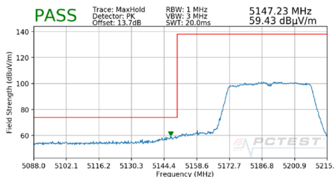
Plot 7-9. Radiated Lower Band Edge Plot SISO ANT1 (Peak – UNII Band 1)
