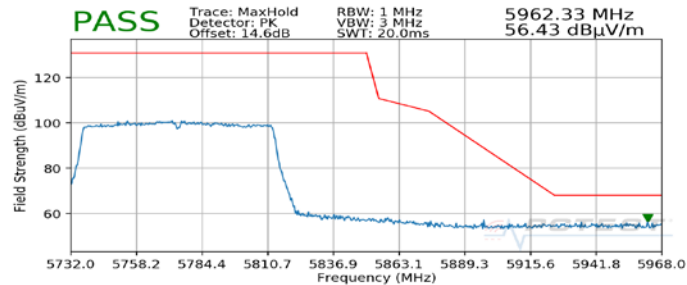
Plot 7-42. Radiated Upper Band Edge Plot SISO ANT2 (Peak - UNII Band 3)
