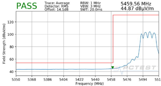
Plot 7-47. Radiated Lower Band Edge Plot MIMO (Average – UNII Band 2C)
