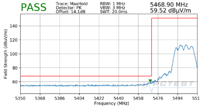
Plot 7-48. Radiated Lower Band Edge Plot MIMO (Peak – UNII Band 2C)
