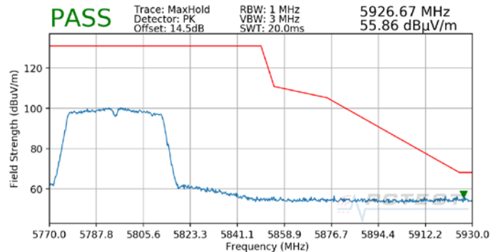
Plot 7-14. Radiated Upper Band Edge Plot SISO ANT1 (Peak - UNII Band 3)
