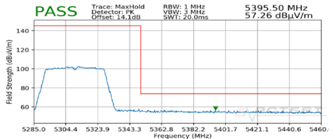
Plot 7-32. Radiated Upper Band Edge Plot SISO ANT2 (Peak – UNII Band 2A)
