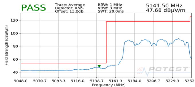
Plot 7-57. Radiated Lower Band Edge Plot MIMO (Average – UNII Band 1)
