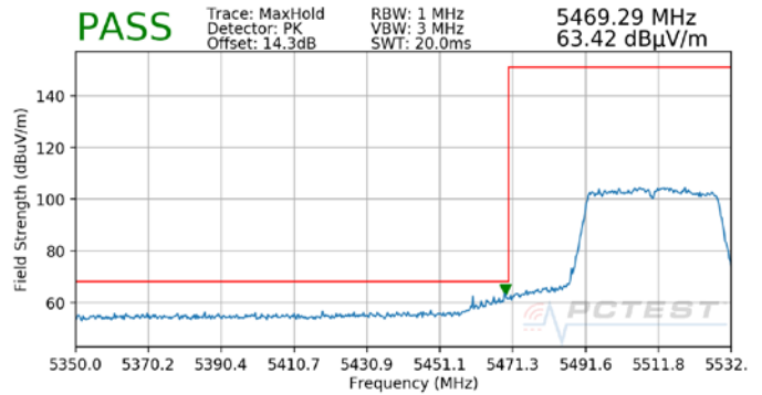
Plot 7-55. Radiated Lower Band Edge Plot MIMO (Peak – UNII Band 2C)
