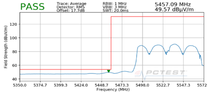
Plot 7-61. Radiated Lower Band Edge Plot MIMO (Average – UNII Band 2C)
