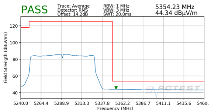
Plot 7-17. Radiated Upper Band Edge Plot SISO ANT1 (Average – UNII Band 2A)
