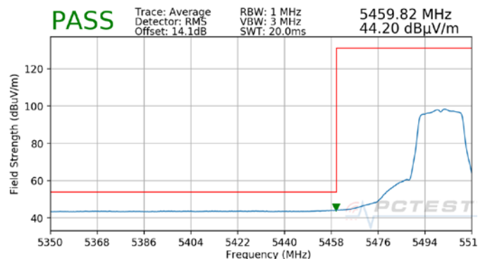
Plot 7-5. Radiated Lower Band Edge Plot SISO ANT1 (Average – UNII Band 2C)
