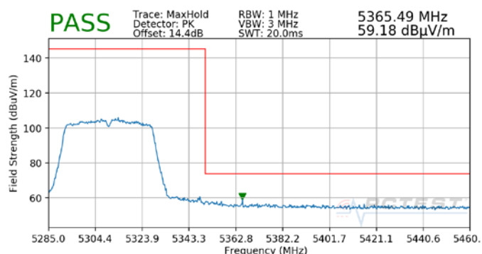
Plot 7-53. Radiated Upper Band Edge Plot MIMO (Peak – UNII Band 2A)
