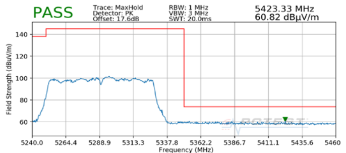
Plot 7-60. Radiated Upper Band Edge Plot MIMO (Peak – UNII Band 2A)
