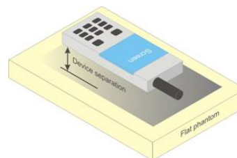
Figure 6-4 Sample Body-Worn Diagram
