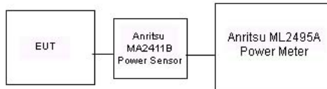
Figure 9-5 Power Measurement Setup for Bandwidths < 50 MHz
