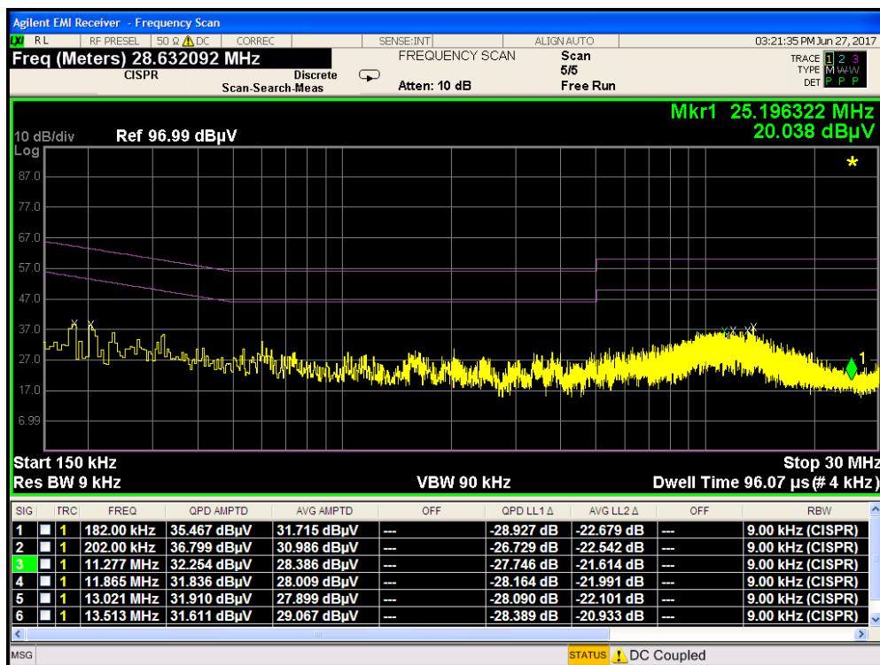
Plot 7-38. Line Conducted Plot with Bluetooth LE (N)
