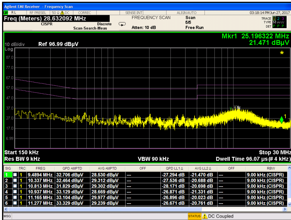
Plot 7-37. Line Conducted Plot with Bluetooth LE (L1)
