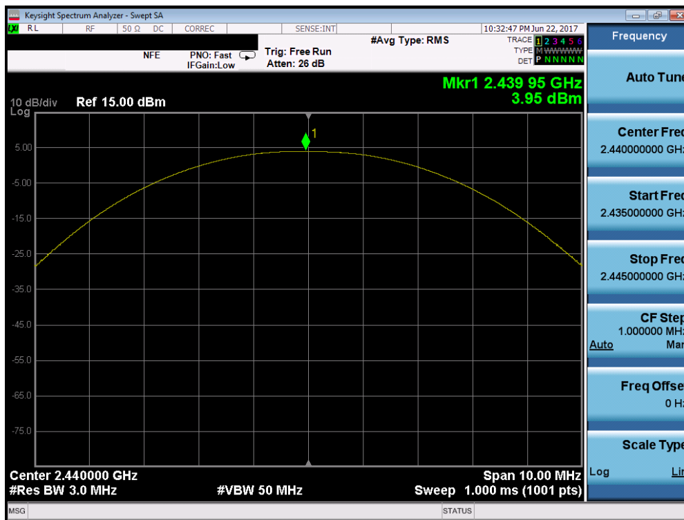
Plot 7-8. Peak Power Plot (Bluetooth (LE), 1Mbps – Ch. 19)
