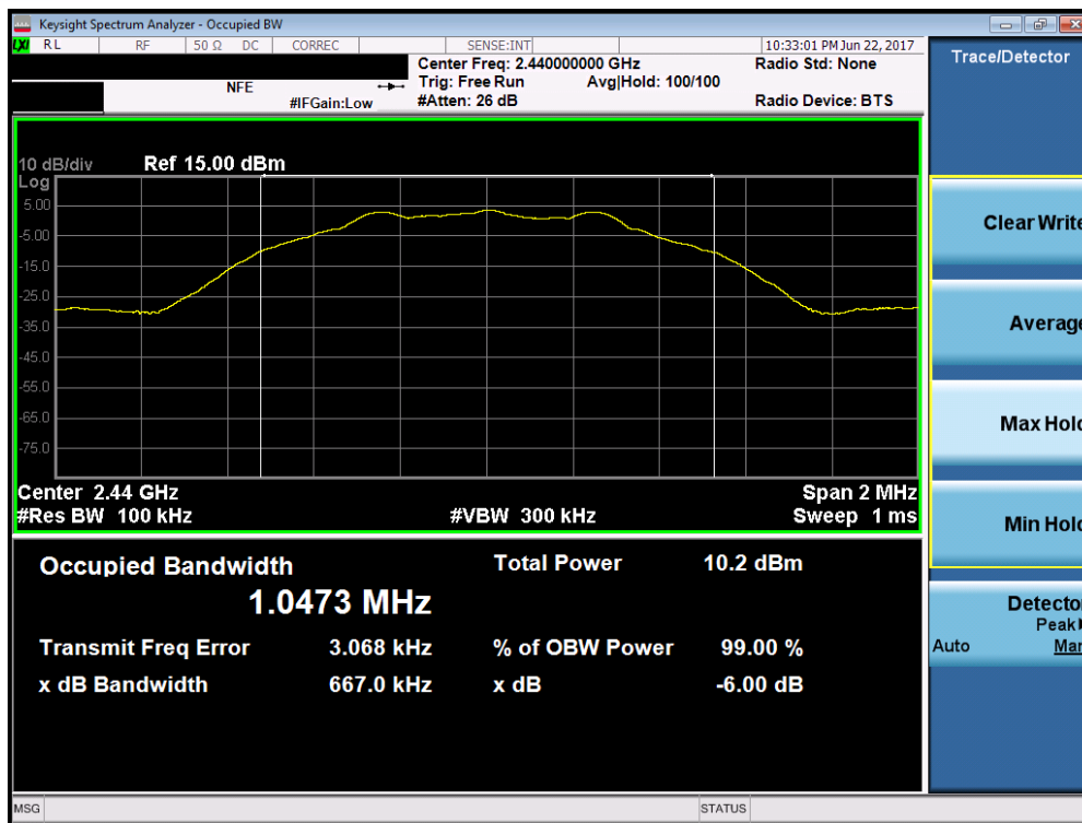
Plot 7-2. 6dB Bandwidth Plot (Bluetooth (LE), 1Mbps – Ch. 19)
