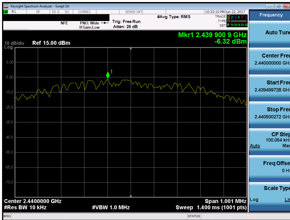
Plot 7-14. Power Spectral Density Plot (Bluetooth (LE), 1Mbps – Ch. 19)
