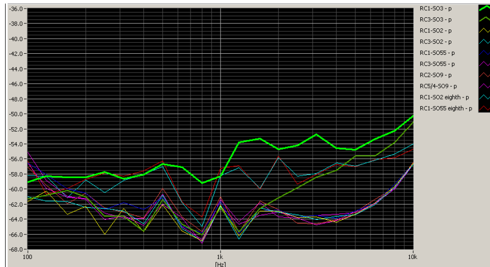
Figure 6-1 CDMA Audio Band Magnetic Noise
