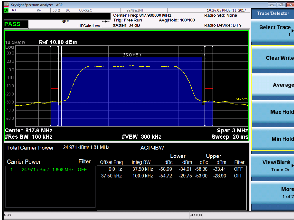
Plot 7-26. Channel Edge Plot (CDMA BC10 - Ch. 476)
