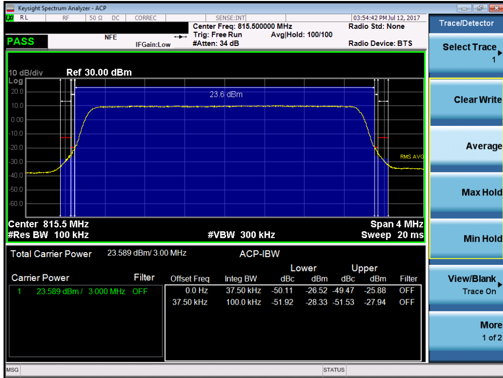
Plot 7-30. Channel Edge Plot (LTE Band 26 - 3MHz QPSK – RB Size 15– Low Channel)
