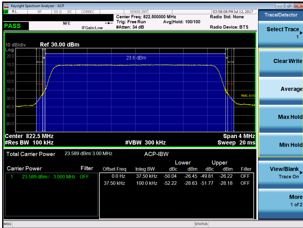
Plot 7-31. Channel Edge Plot (LTE Band 26 - 3MHz QPSK – RB Size 15 – High Channel)
