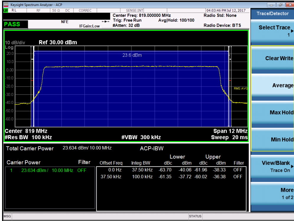
Plot 7-34. Channel Edge Plot (LTE Band 26 - 10MHz QPSK – RB Size 50)
