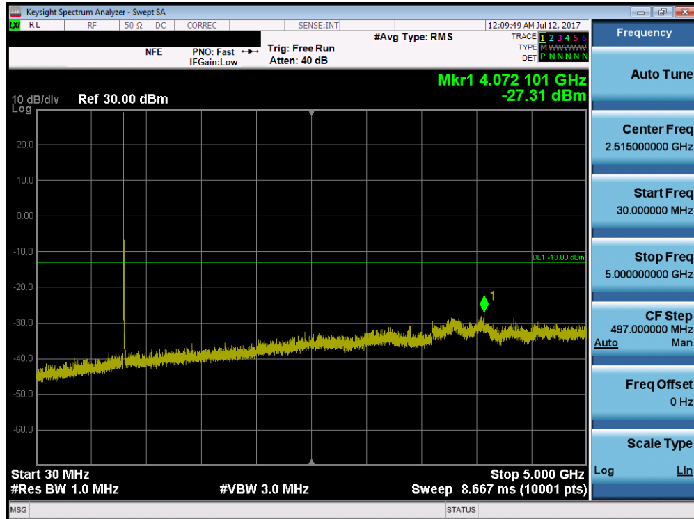
Plot 7-24. Conducted Spurious Plot (LTE Band 26 - 5.0MHz QPSK – RB Size 1, RB Offset 0 – High Channel)
