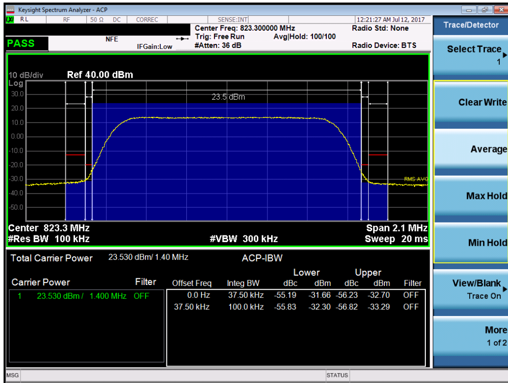
Plot 7-29. Channel Edge Plot (LTE Band 26 - 1.4MHz QPSK – RB Size 6 – High Channel)
