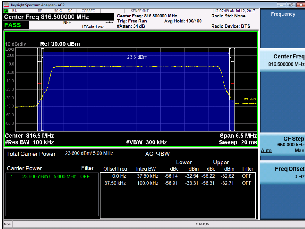
Plot 7-32. Channel Edge Plot (LTE Band 26 - 5MHz QPSK – RB Size 25– Low Channel)
