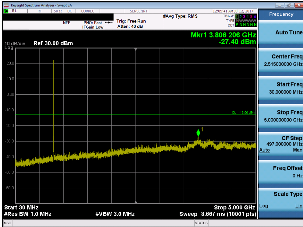
Plot 7-22. Conducted Spurious Plot (LTE Band 26 - 5.0MHz QPSK – RB Size 1, RB Offset 0 – Low Channel)
