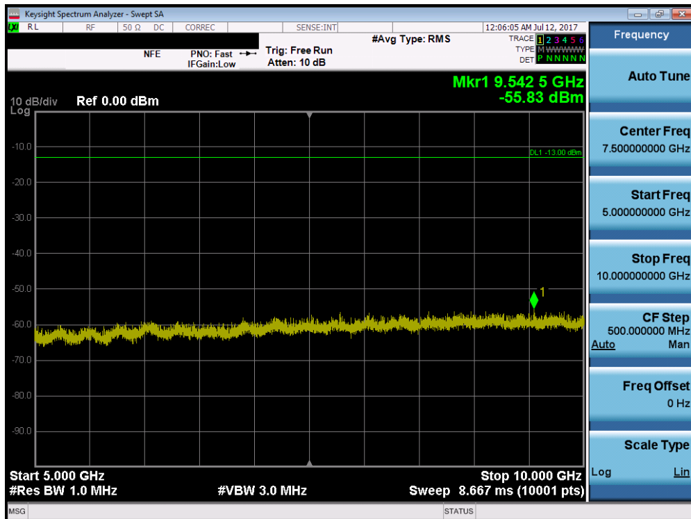
Plot 7-23. Conducted Spurious Plot (LTE Band 26 - 5.0MHz QPSK – RB Size 1, RB Offset 0 – Low Channel)
