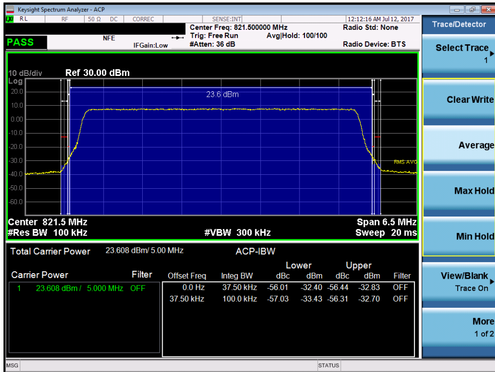
Plot 7-33. Channel Edge Plot (LTE Band 26 - 5MHz QPSK – RB Size 25 – High Channel)
