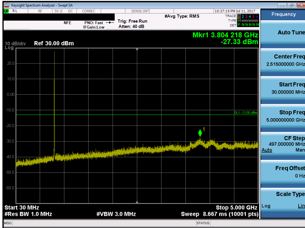
Plot 7-20. Conducted Spurious Plot (CDMA BC10 - Ch. 684)
