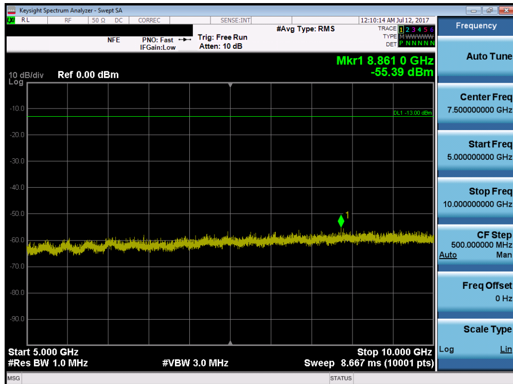
Plot 7-25. Conducted Spurious Plot (LTE Band 26 - 5.0MHz QPSK – RB Size 1, RB Offset 0 – High Channel)
