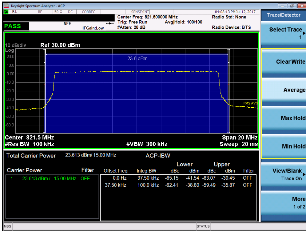
Plot 7-35. Channel Edge Plot (LTE Band 26 - 15MHz QPSK – RB Size 75)
