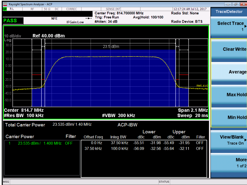
Plot 7-28. Channel Edge Plot (LTE Band 26 - 1.4MHz QPSK – RB Size 6– Low Channel)
