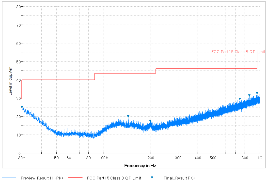
Plot 7-52. Radiated Spurious Plot below 1GHz (Pol. H)
