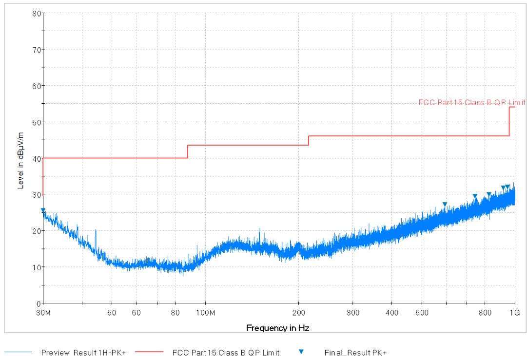
Plot 7-53. Radiated Spurious Plot below 1GHz (Pol. V)
