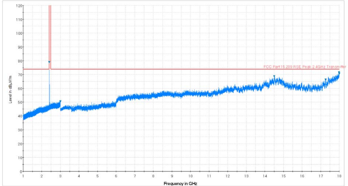
Plot 7-43. Radiated Spurious Plot above 1GHz (BT – Ch. 0, Ant. Pol. V)
